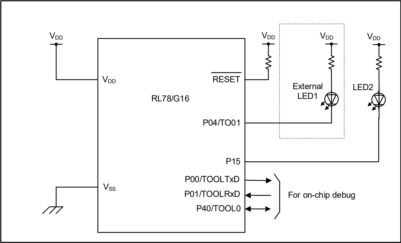
Figure 3-1 Hardware Configuration
