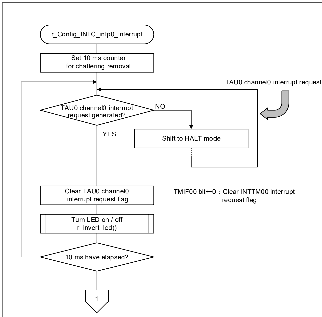
Figure 4-3 External Interrupt Processing (1/2)
