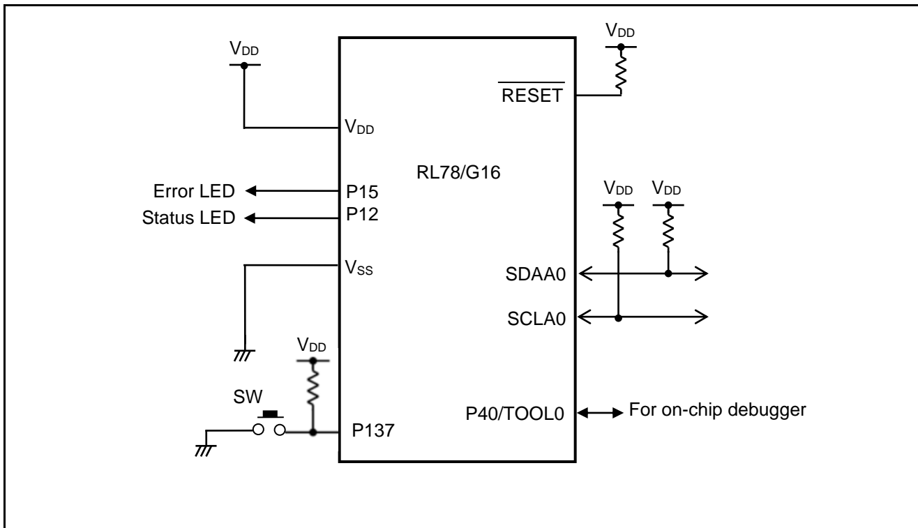
Figure 4.1 Hardware Configuration
