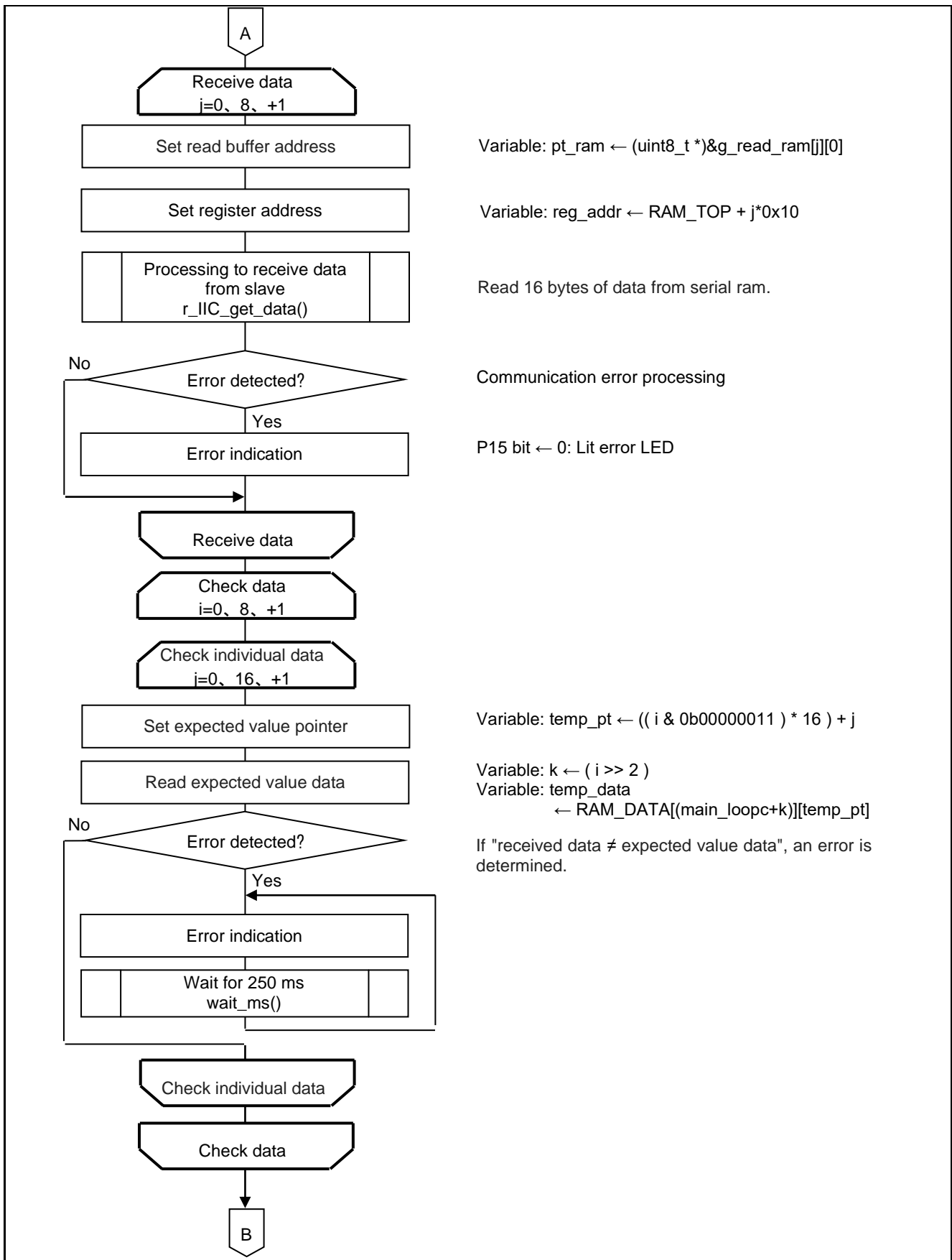
Figure 5.2 Main Processing (2/3)
