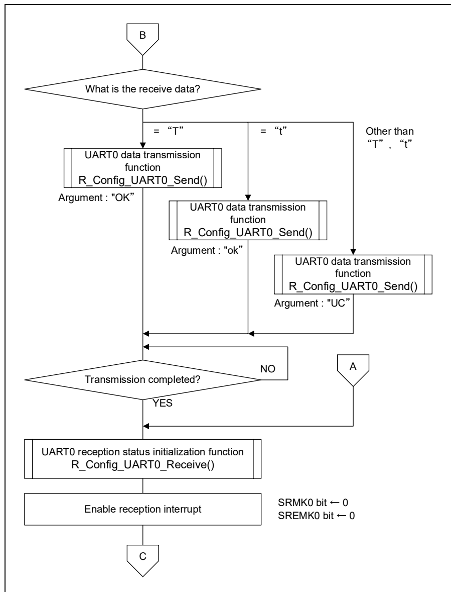
Figure 4-2 Main Processing (2/2)
