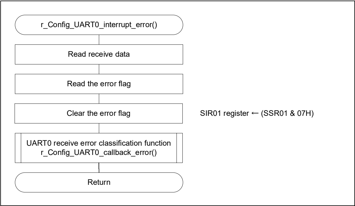
Figure 4-5 UART0 Error Interrupt Handling
