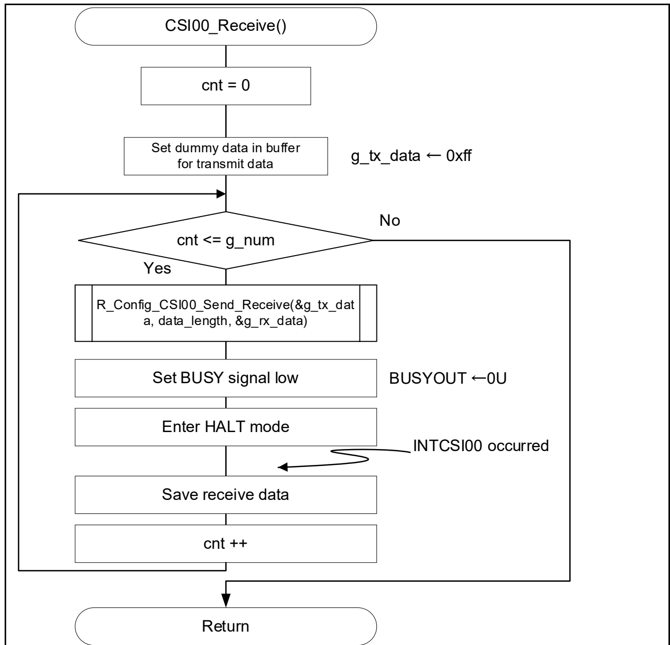
Figure 5-6 CSI Reception
