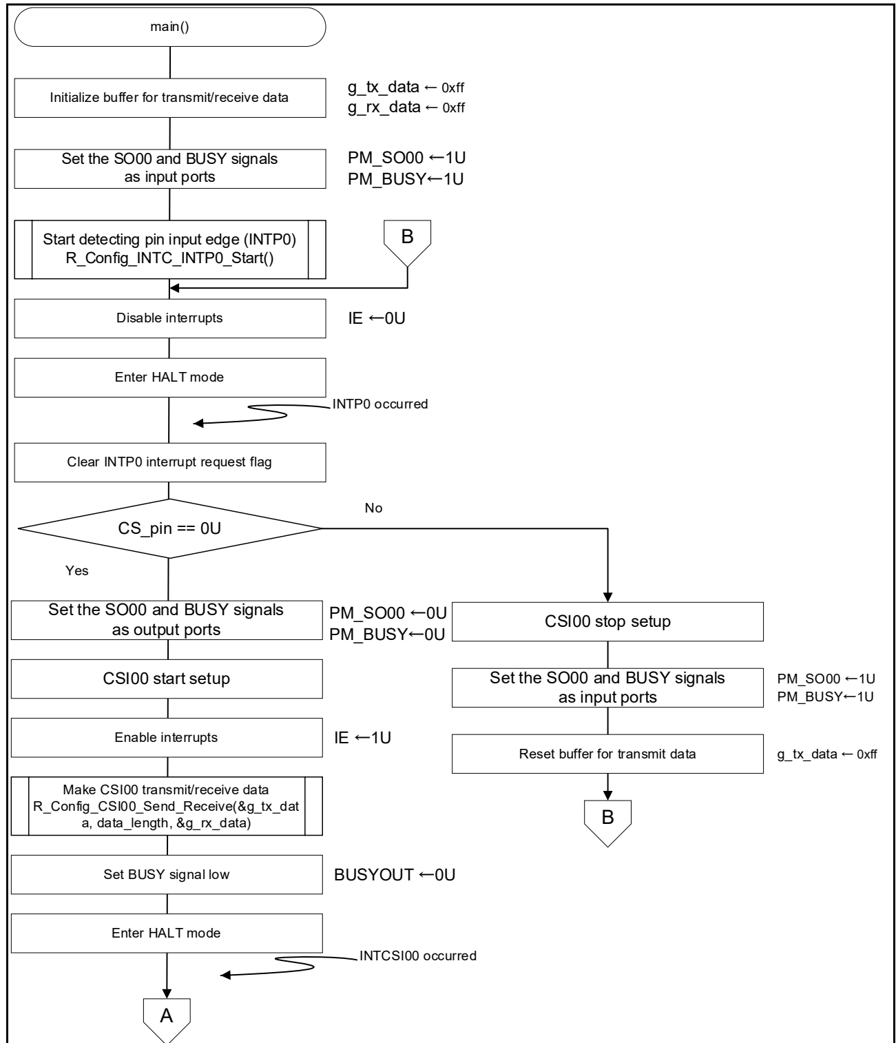
Figure 5-1 Main Processing 1/2
