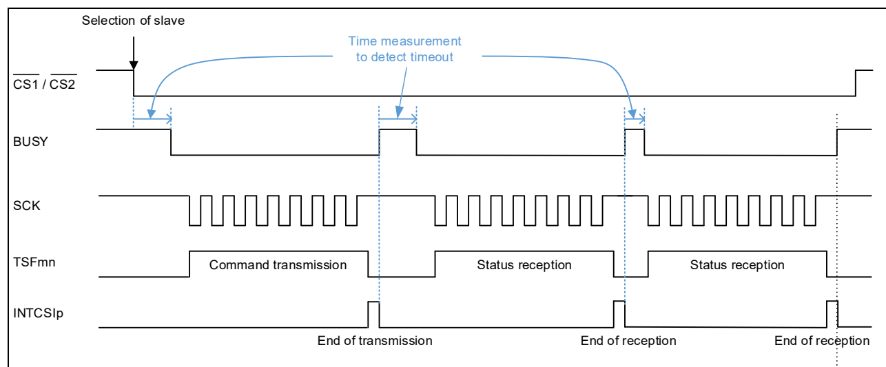
Figure 1-1 Handshaking Example
