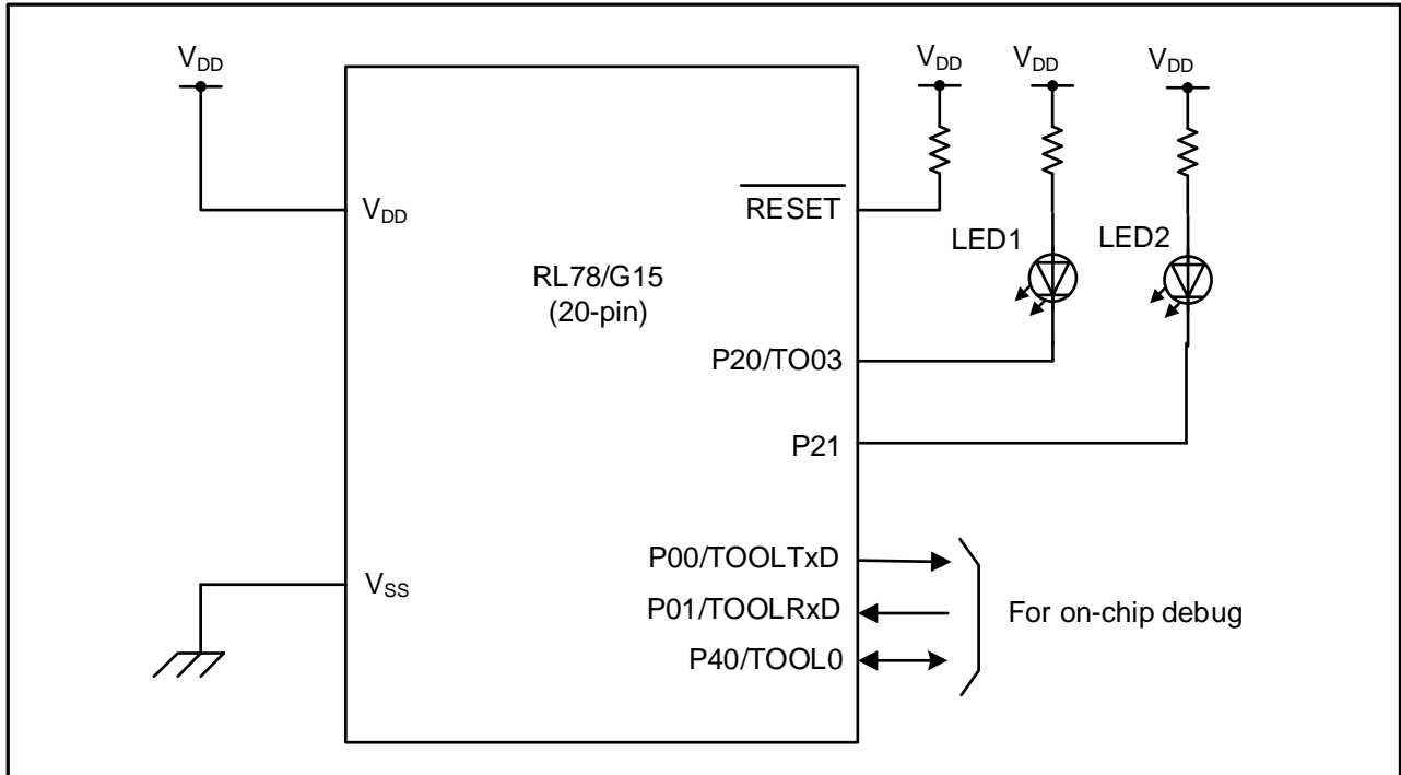
Figure 3-1 Hardware Configuration
