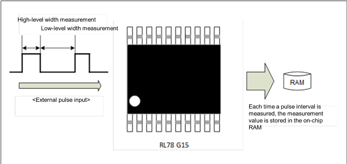
Figure 1-1 Overview of Pulse Interval Measurement
