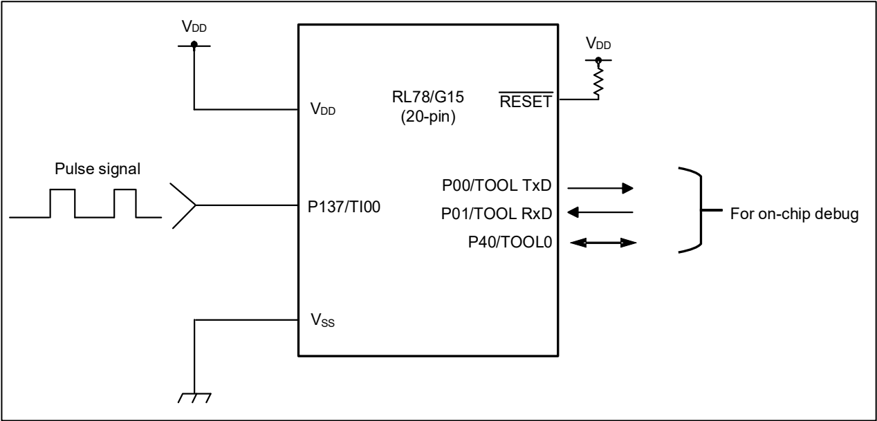
Figure 3-1 Hardware Configuration
