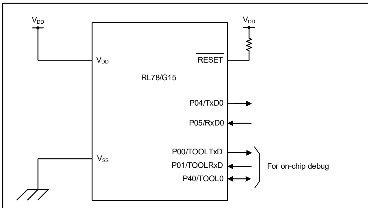
Figure 3-1 Hardware Configuration
