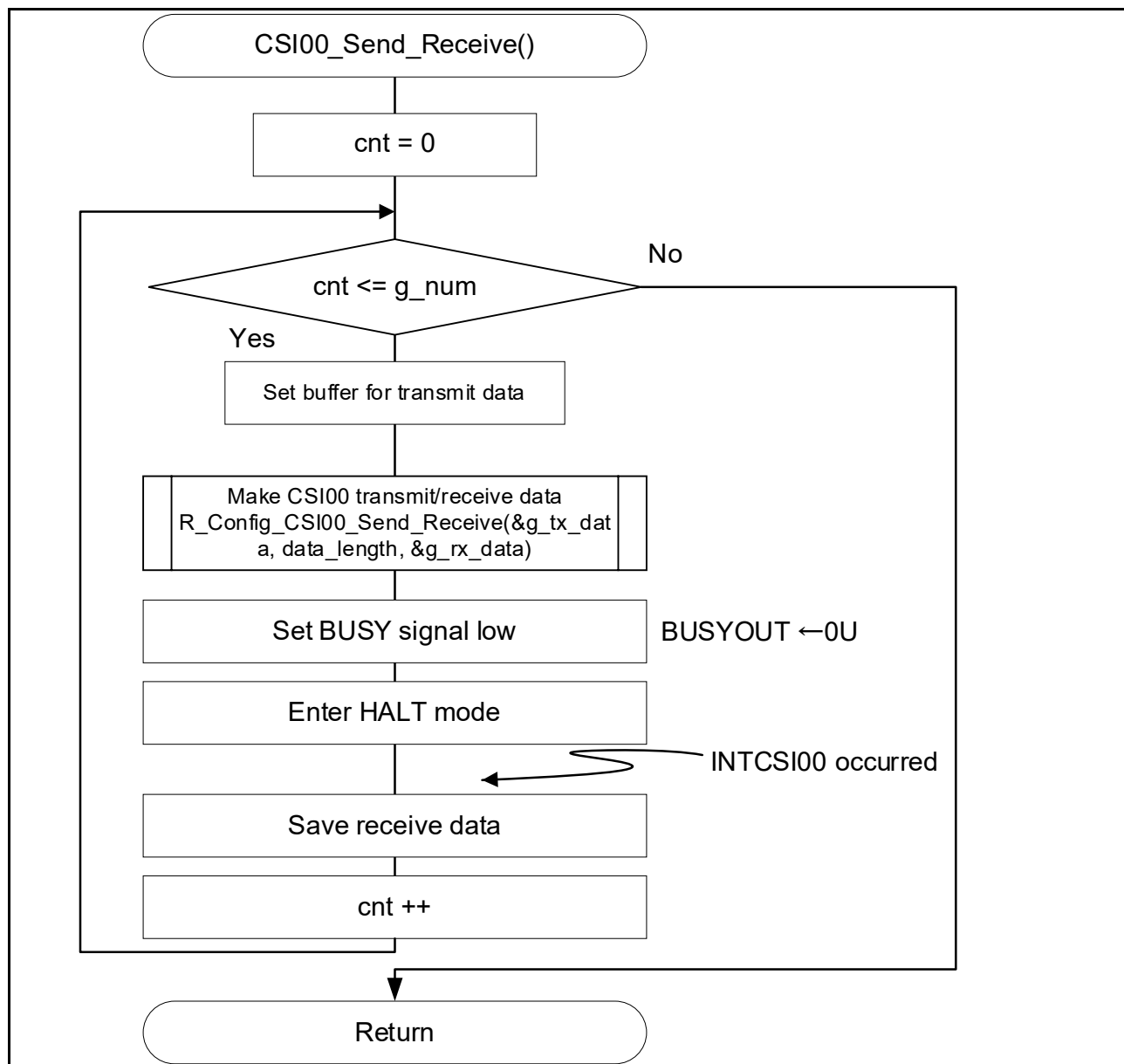
Figure 5-4 CSI Transmission/Reception
