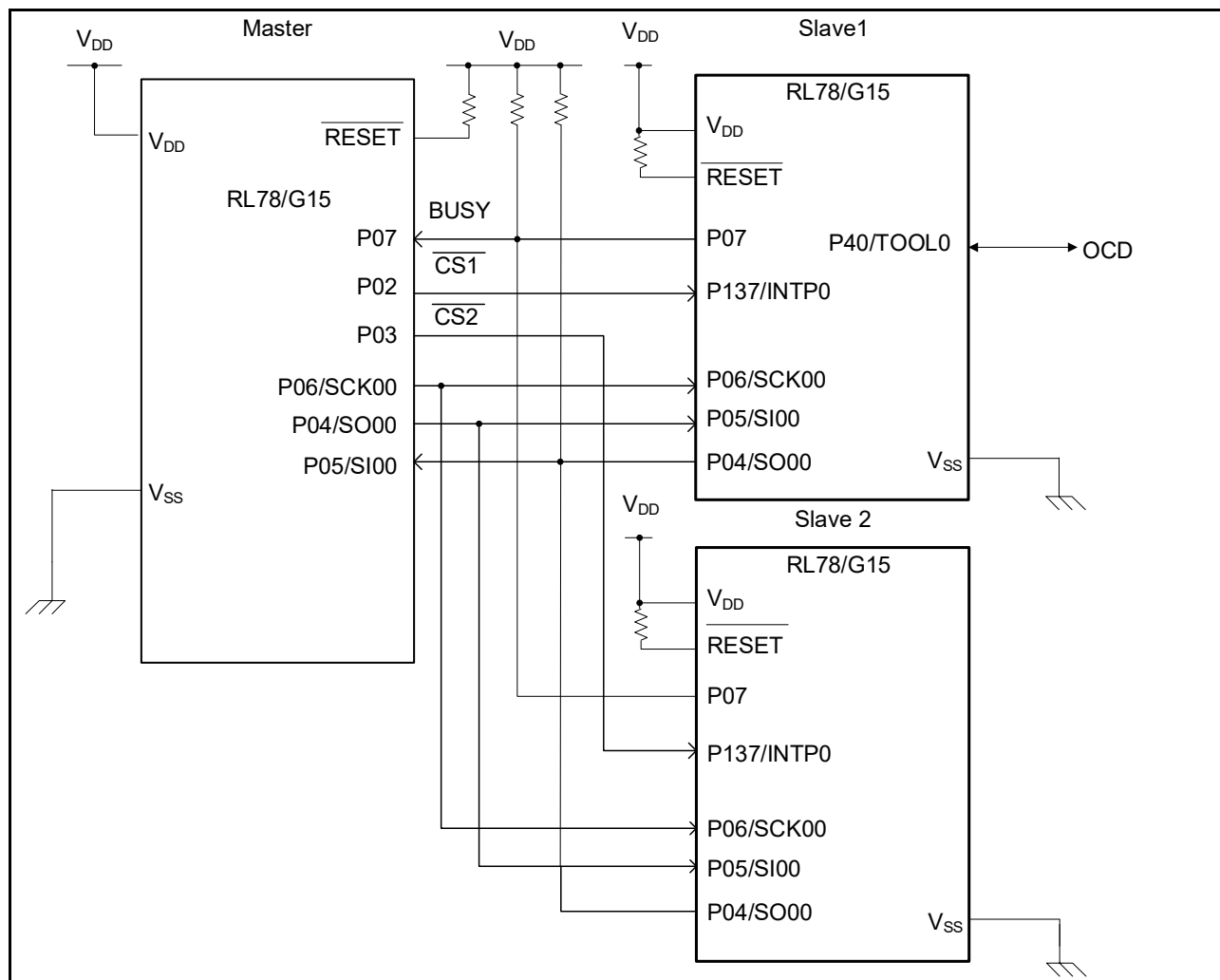
Figure 4-1 Hardware Configuration
