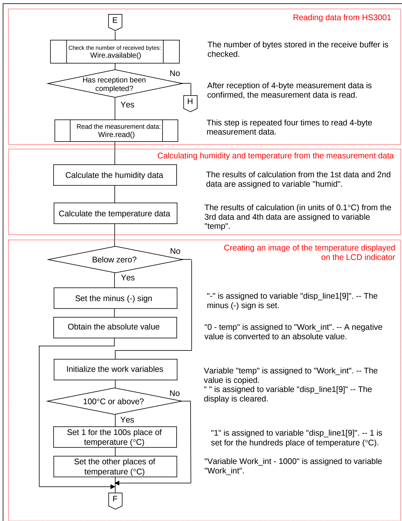
Figure 5.4 Main Function (3/4)
