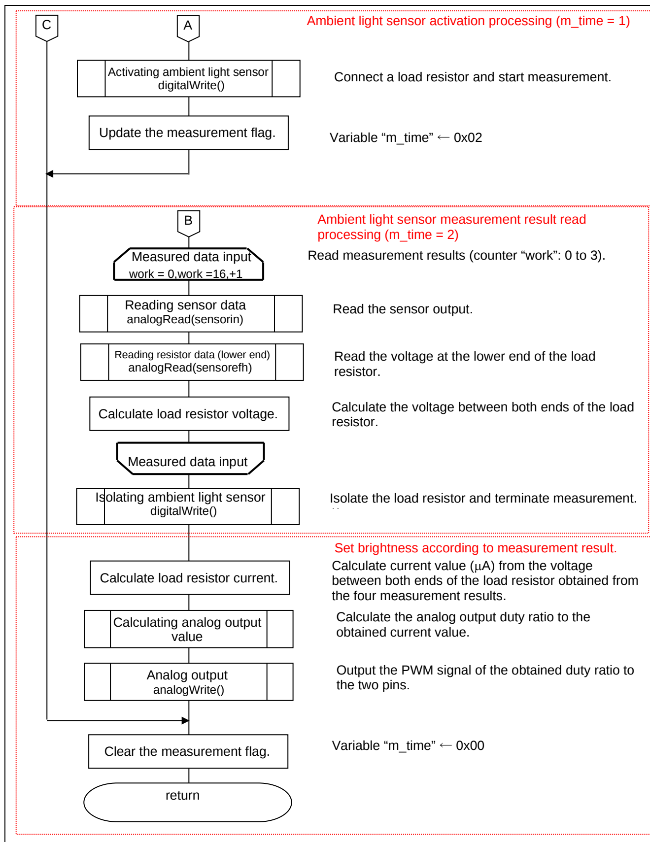
Figure 5.3 Main Function (2/2)
