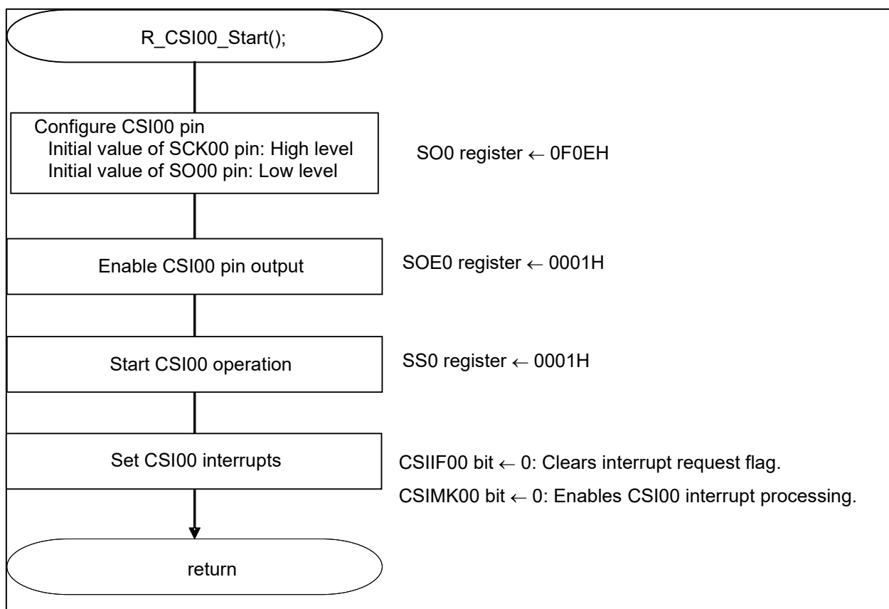
Figure 5-12 CSI00 start operation
