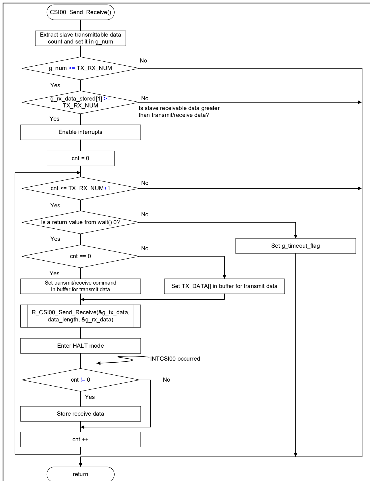
Figure 5-16 CSI Transmission/Reception
