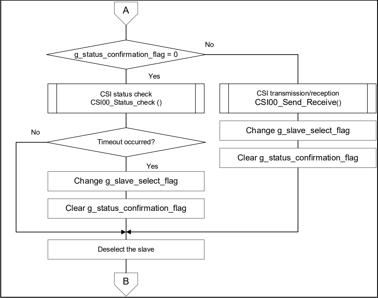
Figure 5-9 Main Processing 2/2
