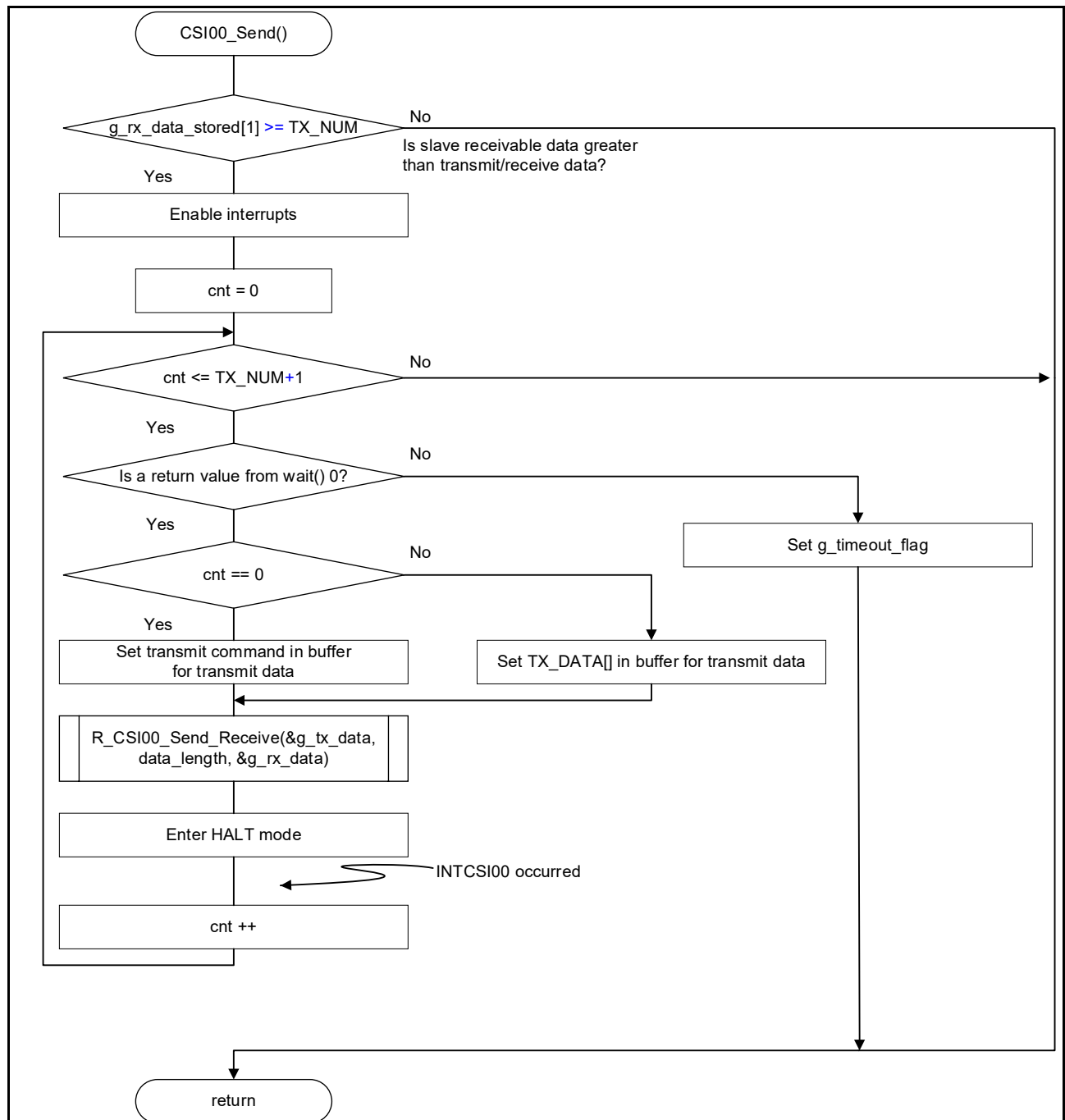
Figure 5-17 CSI Transmission
