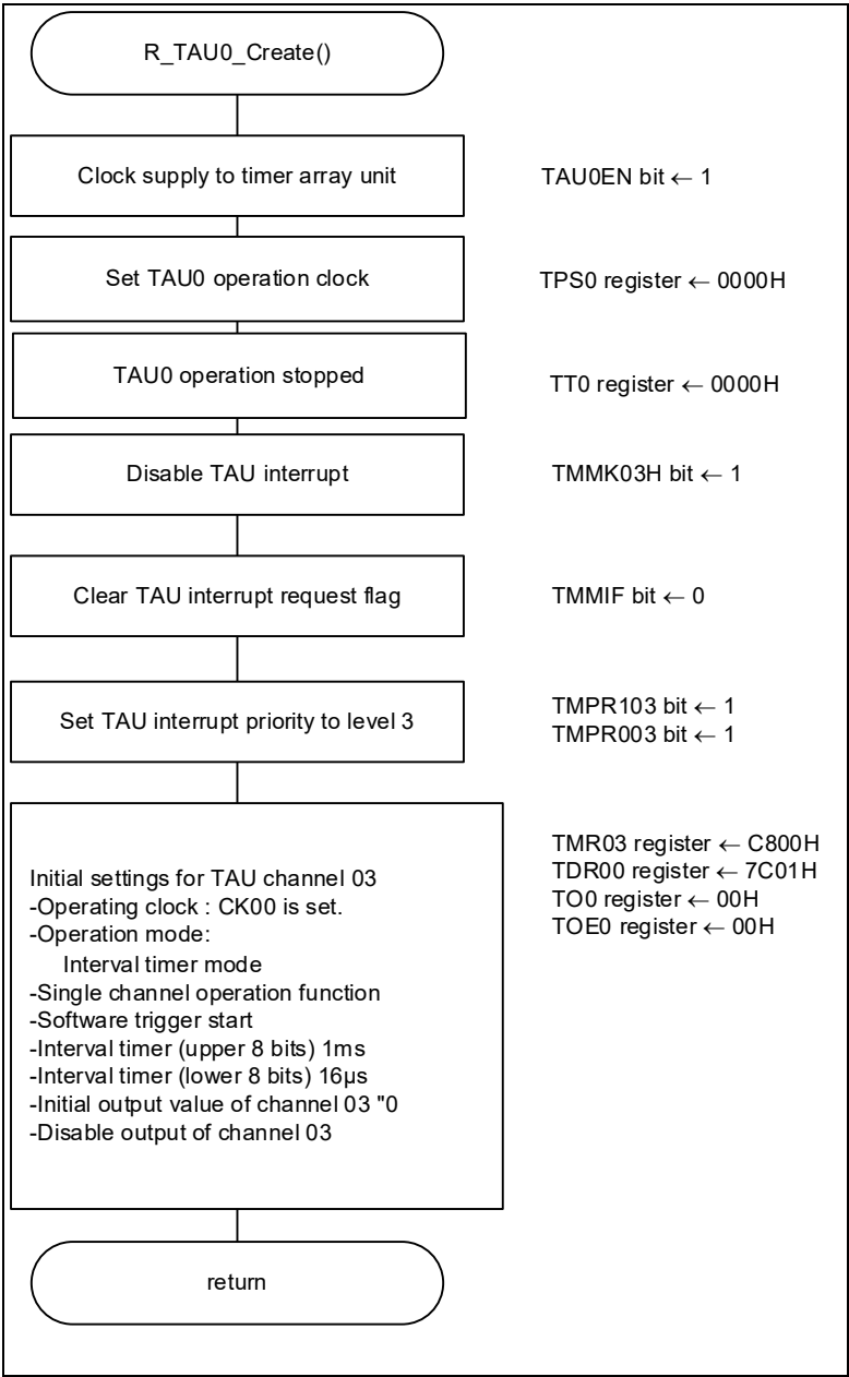
Figure 5-7 TAU0 Configuration
