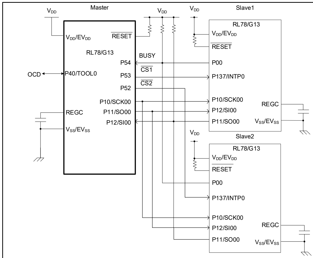
Figure 4-1 Hardware Configuration
