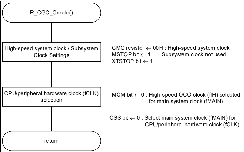
Figure 5-3 CPU clock Configuration
