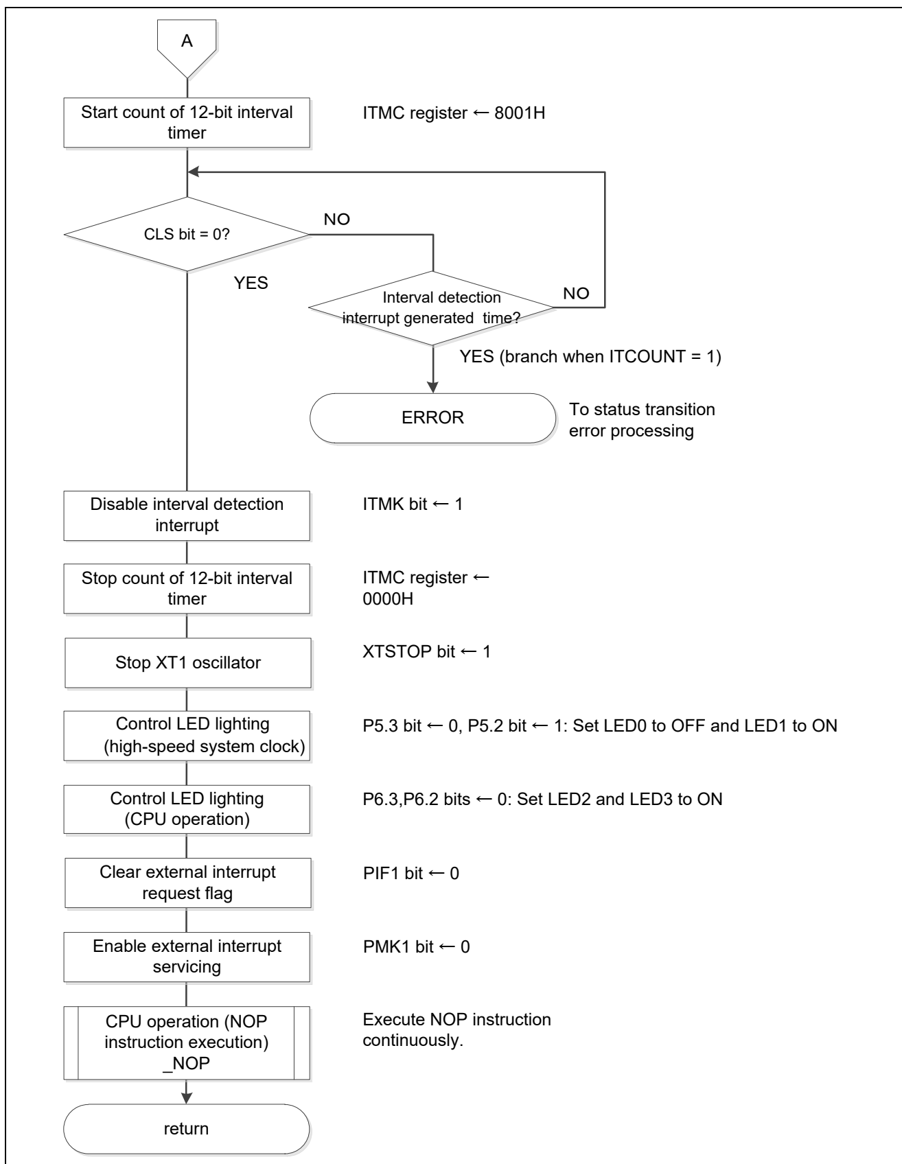
Figure 5.23 Status Transition DtoC (2/2)
