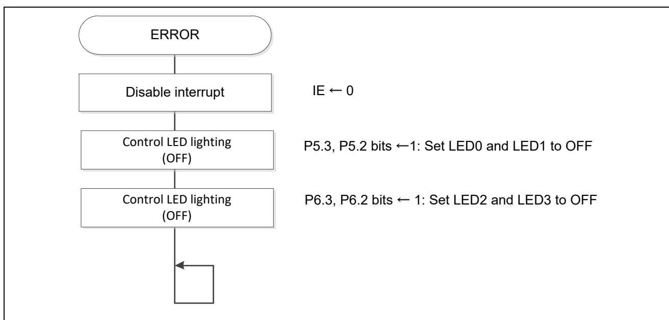
Figure 5.13 Error Processing of Status Transition
