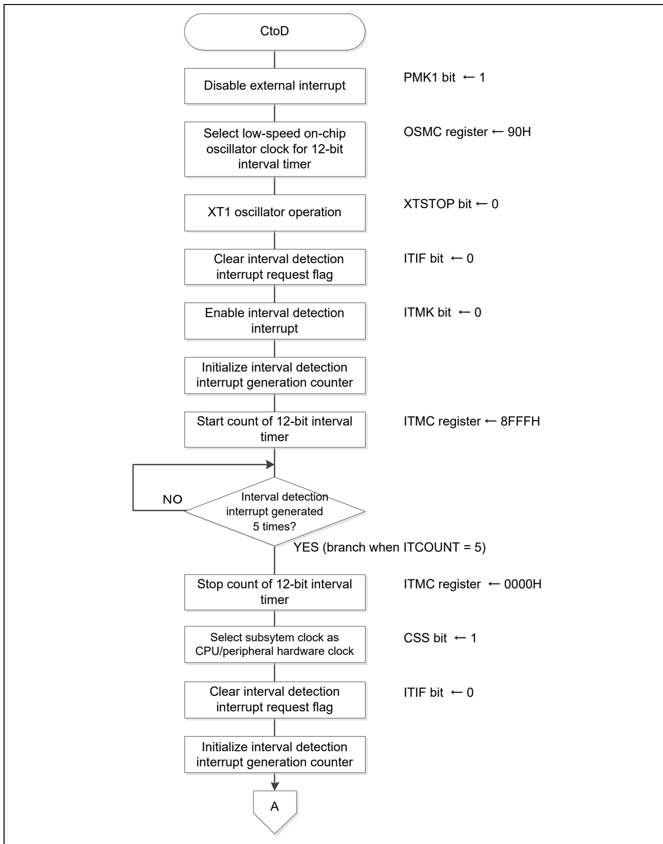
Figure 5.20 Status Transition CtoD (1/2)
