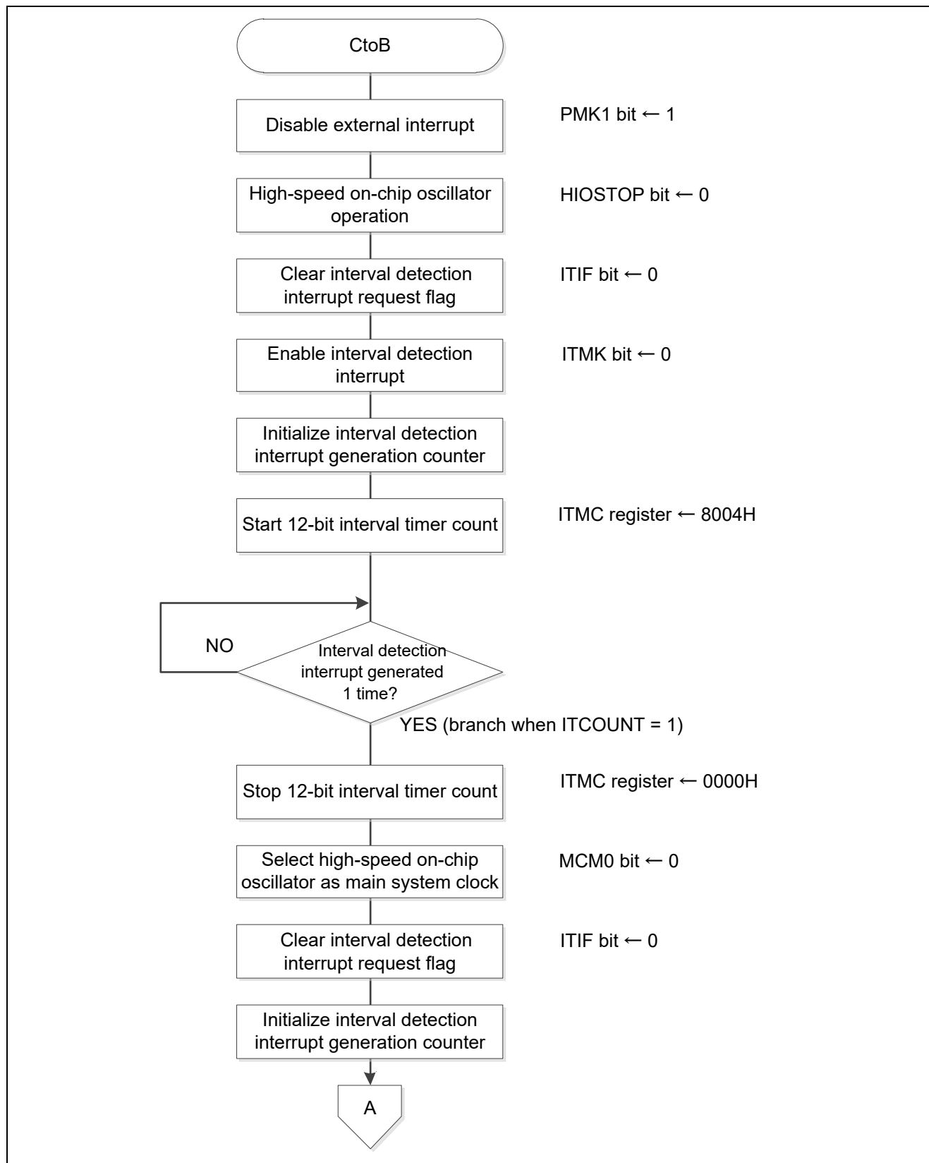
Figure 5.28 Status Transition CtoB (1/2)
