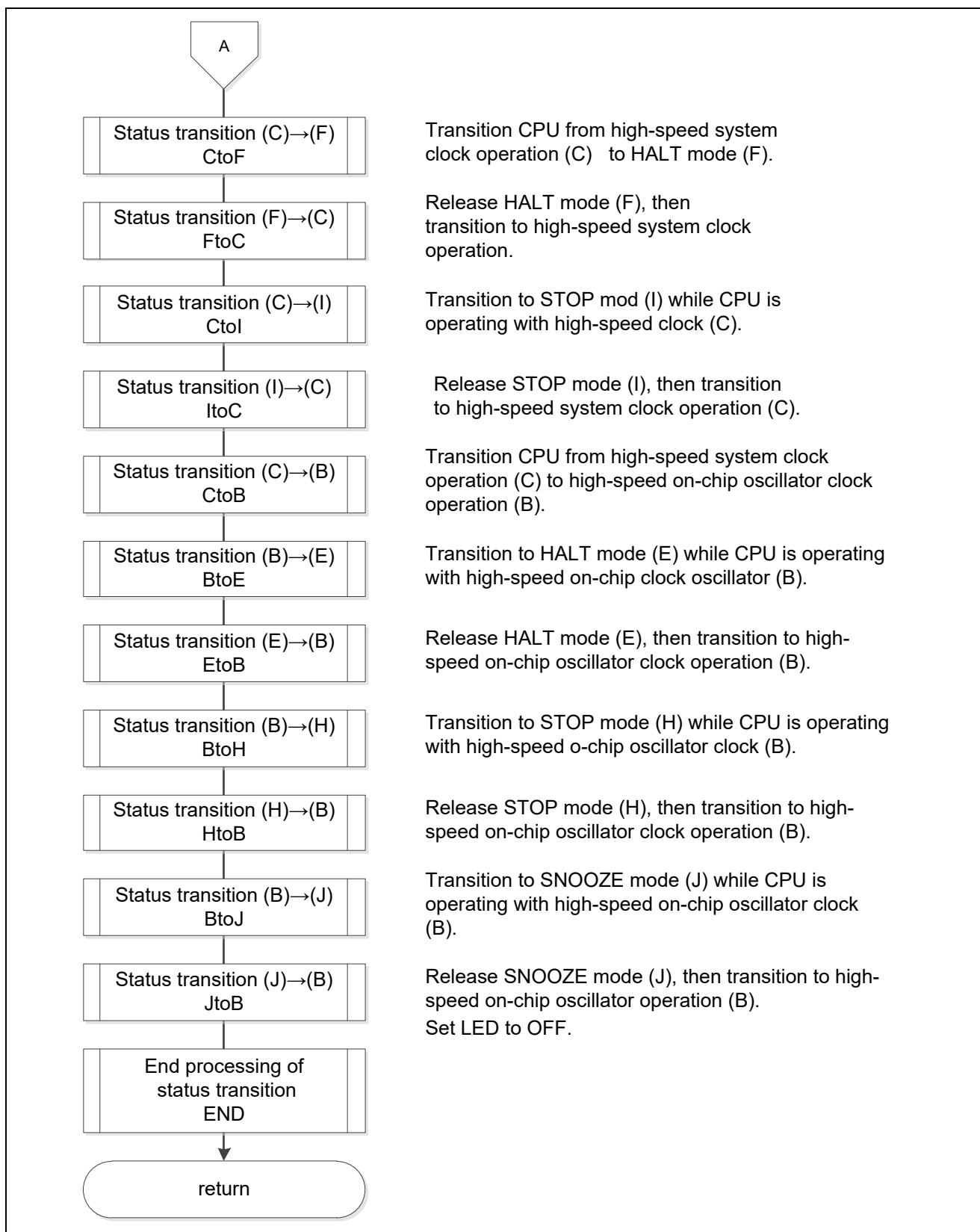
Figure 5.8 Main Processing (2/2)
