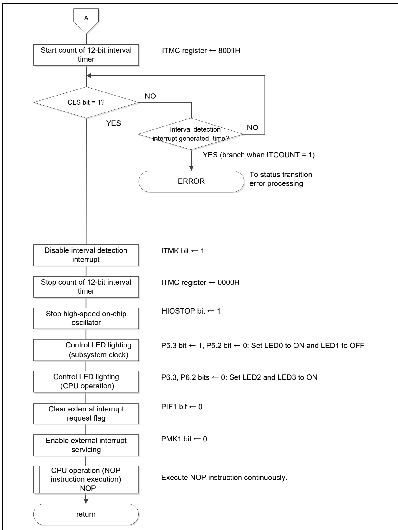
Figure 5.12 Status Transition BtoD (2/2)
