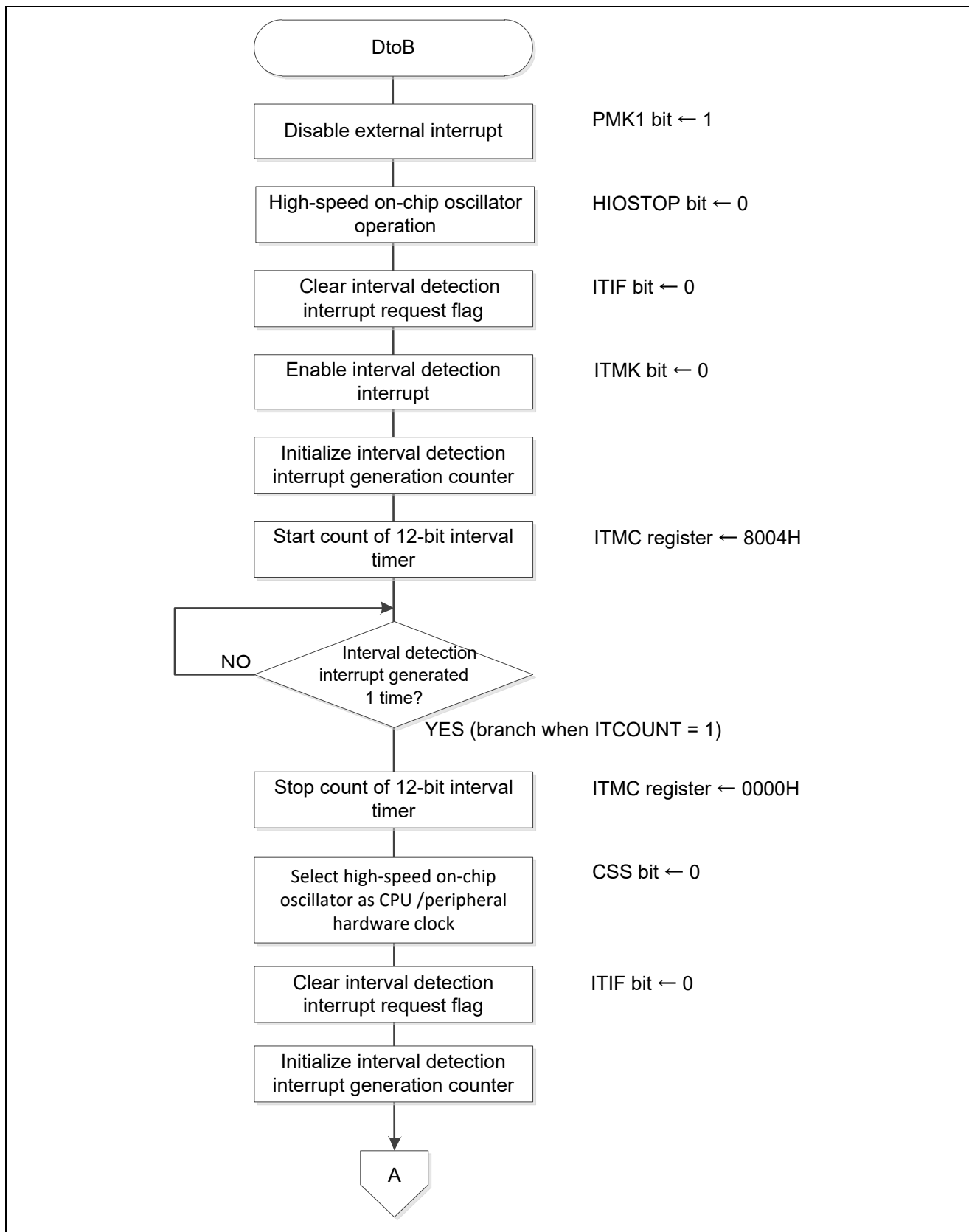
Figure 5.16 Status Transition DtoB (1/2)
