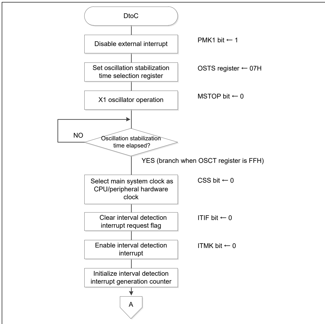
Figure 5.22 Status Transition DtoC (1/2)
