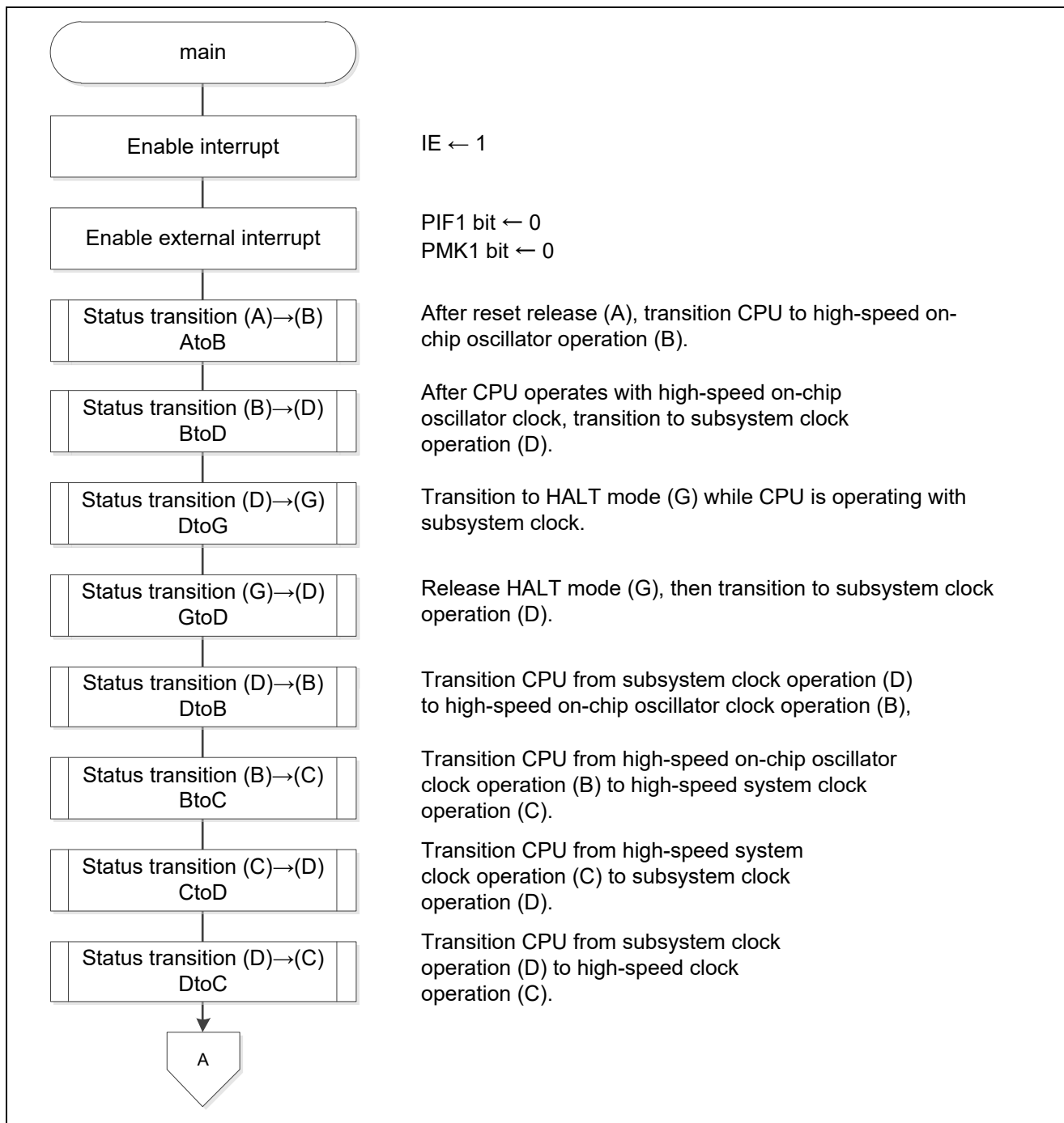
Figure 5.7 Main Processing (1/2)
