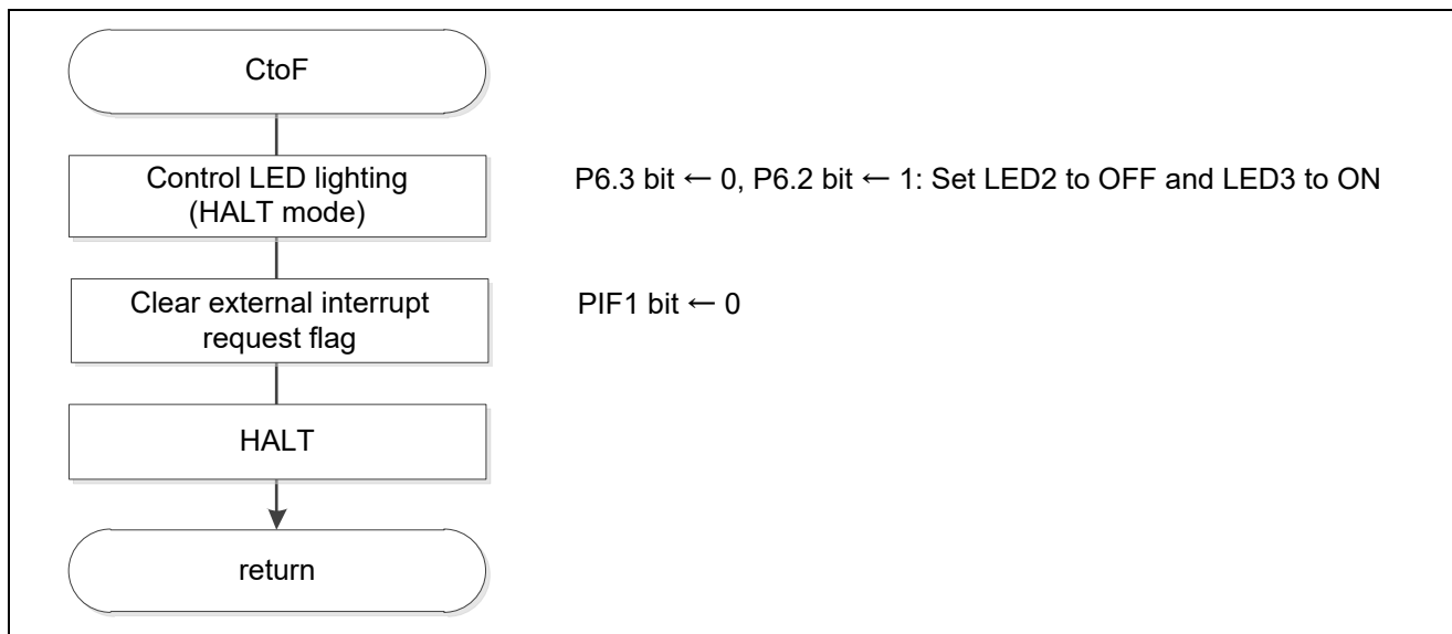
Figure 5.24 Status Transition CtoF
