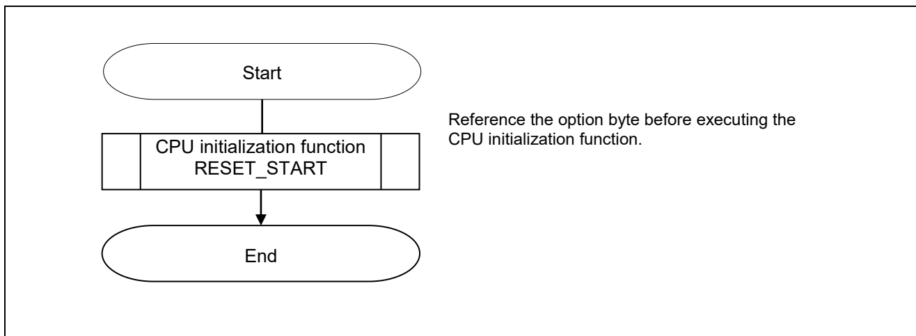
Figure 5.1 Overall Flowchart
