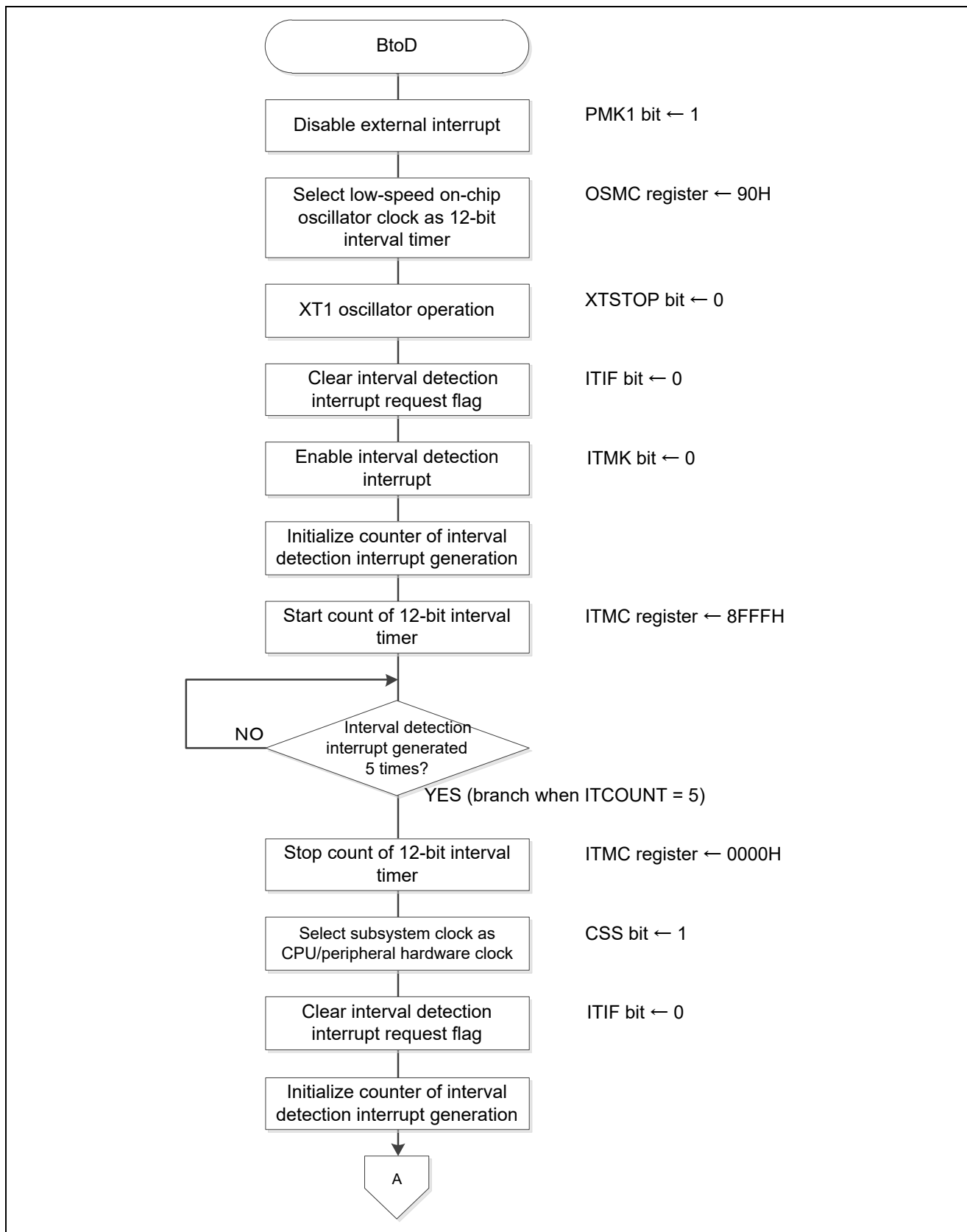
Figure 5.11 Status Transition BtoD (1/2)
