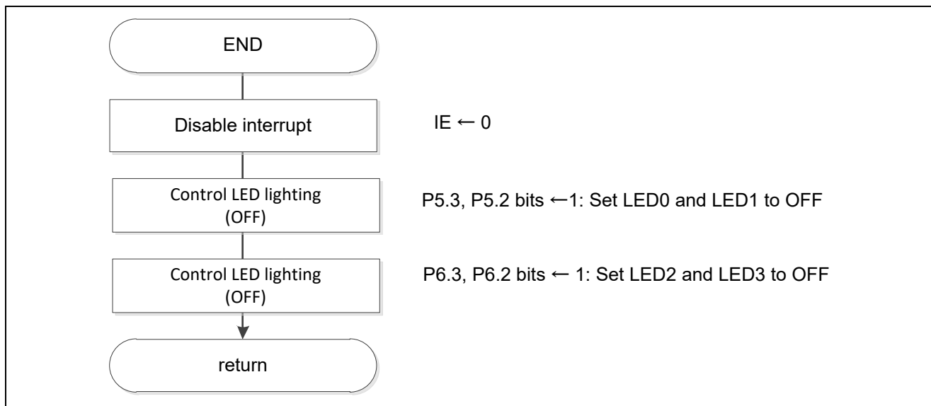
Figure 5.37 Status Transition End Processing
