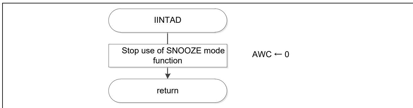
Figure 5.40 A/D Conversion Completion Interrupt Servicing
