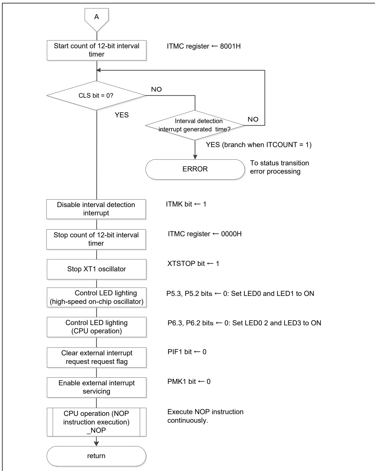
Figure 5.17 Status Transition DtoB (2/2)
