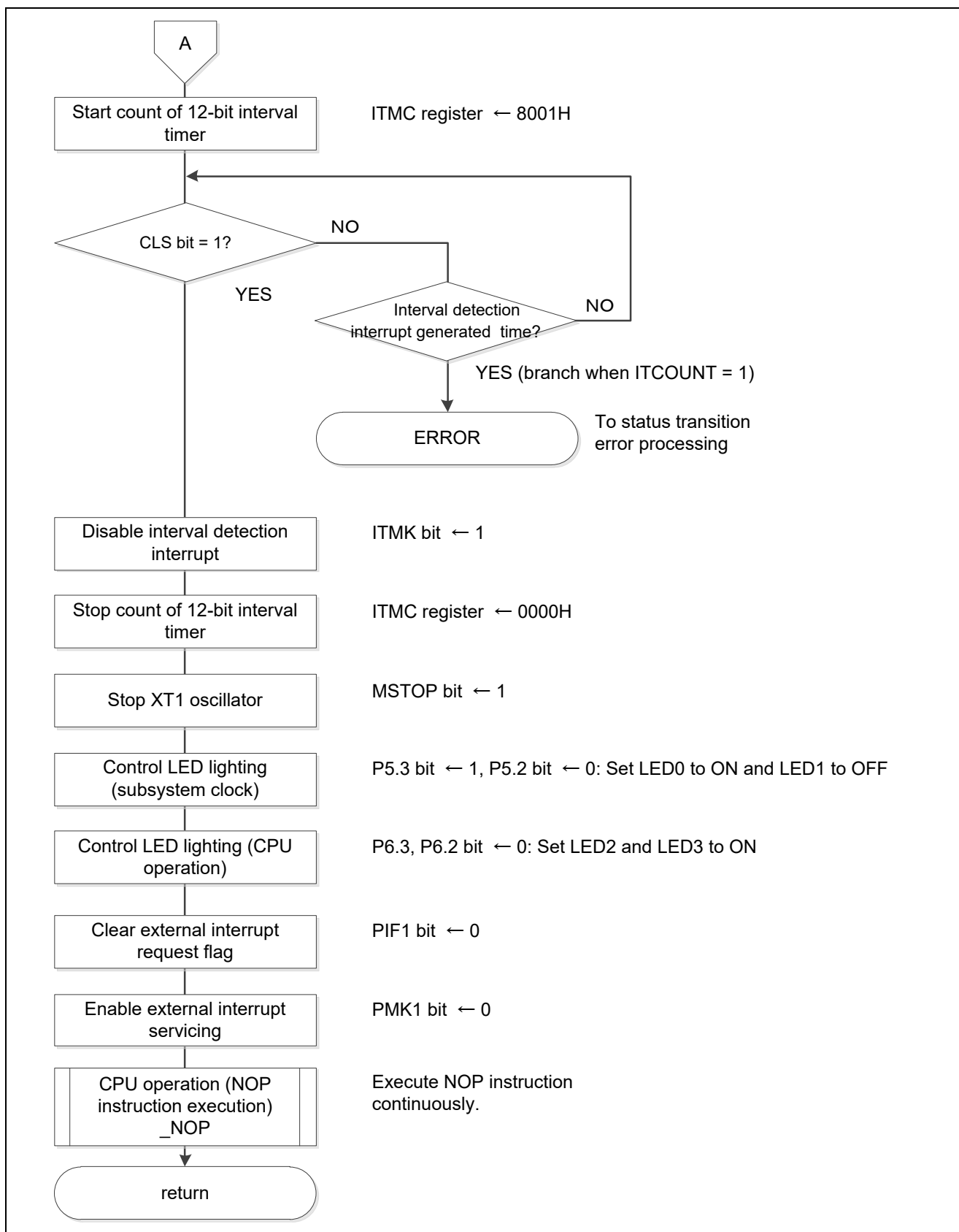
Figure 5.21 Status Transition CtoD (2/2)
