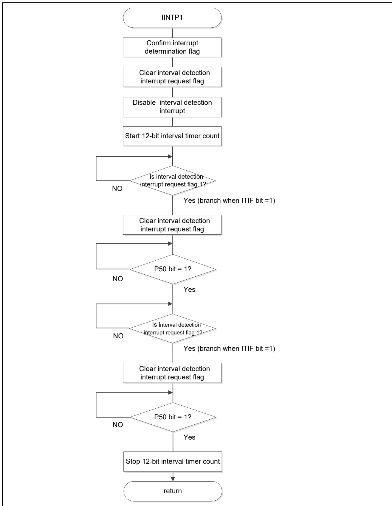
Figure 5.38 External Interrupt Servicing
