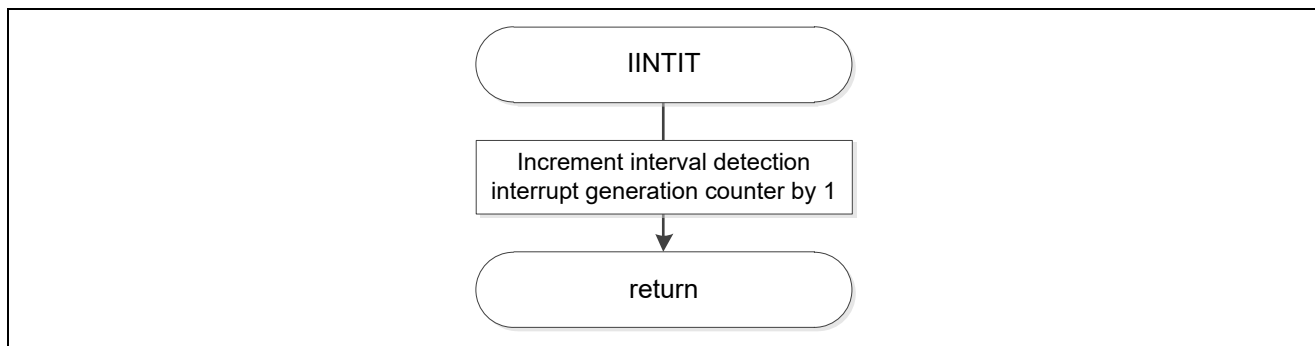
Figure 5.39 12-bit Interval Timer Interrupt Servicing
