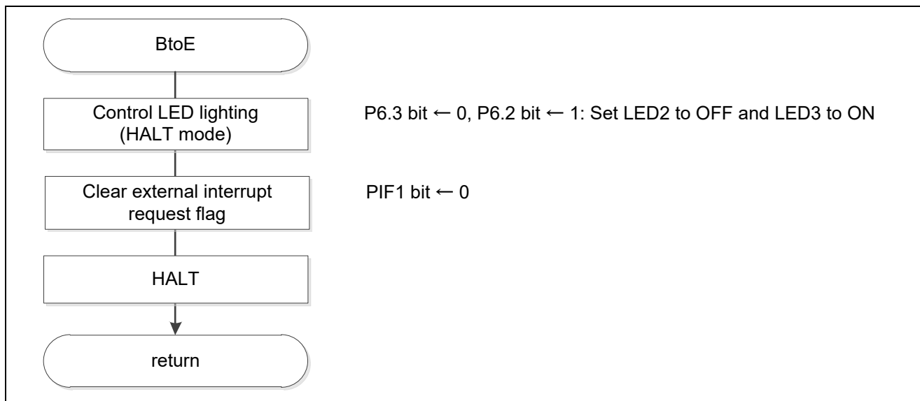
Figure 5.30 Status Transition BtoE
