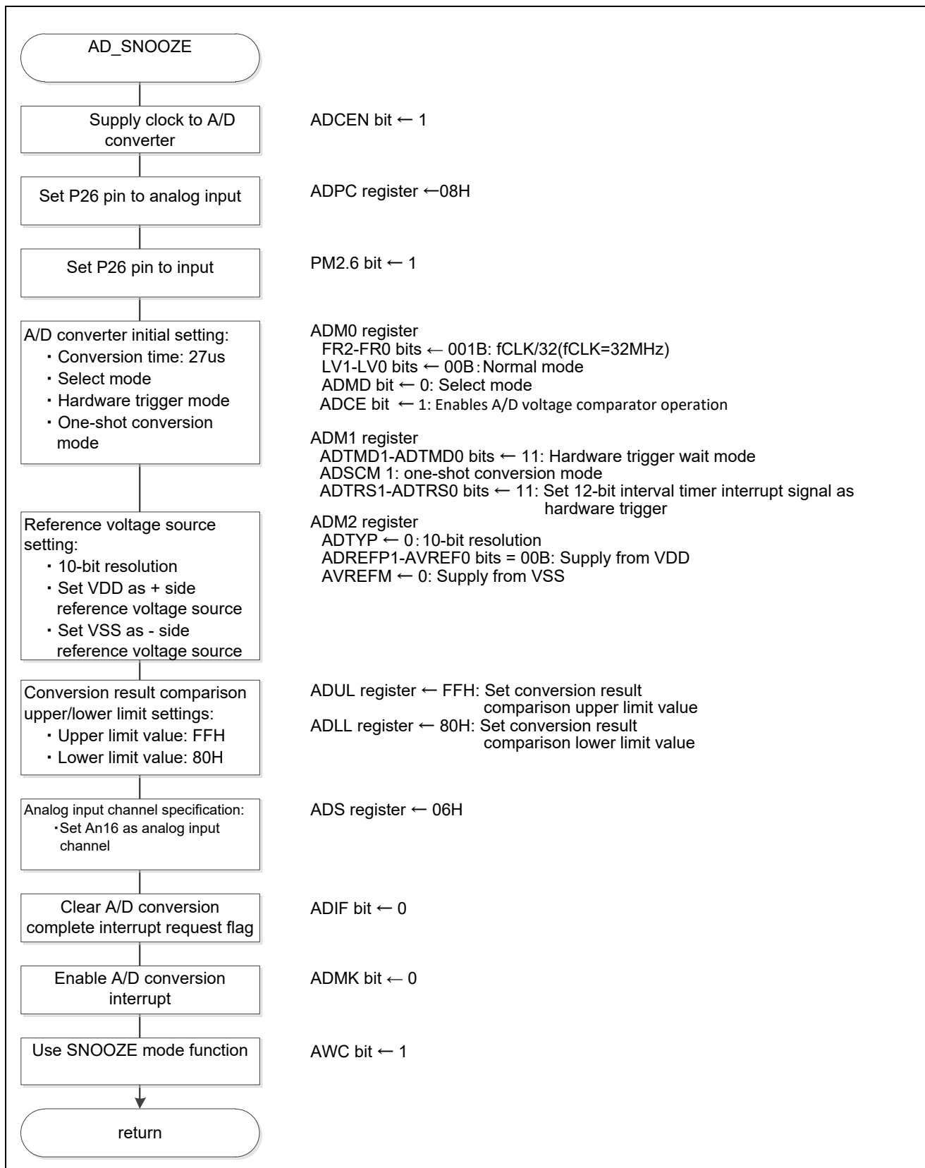
Figure 5.35 A/D Converter Setting
