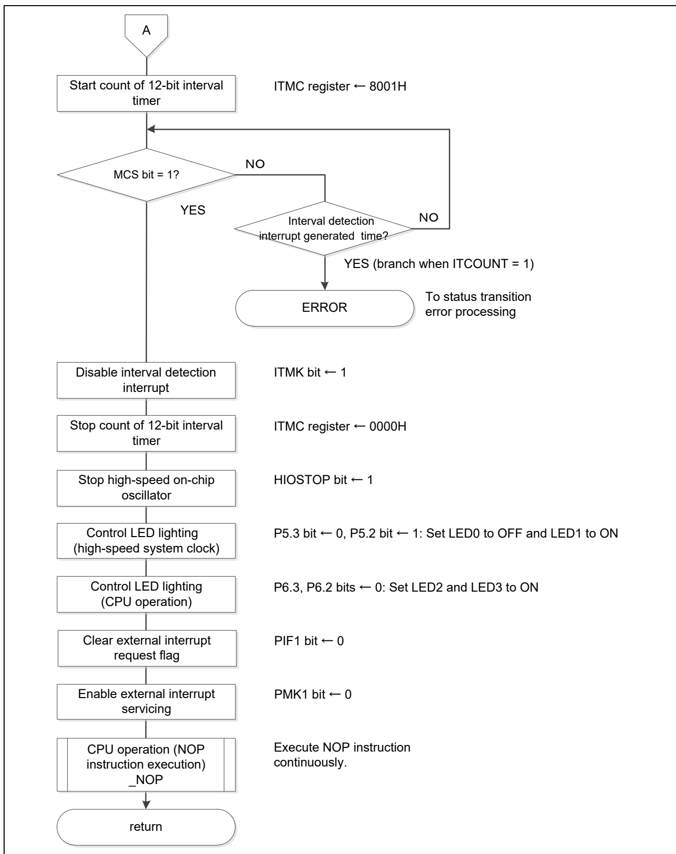
Figure 5.19 Status Transition BtoC (2/2)
