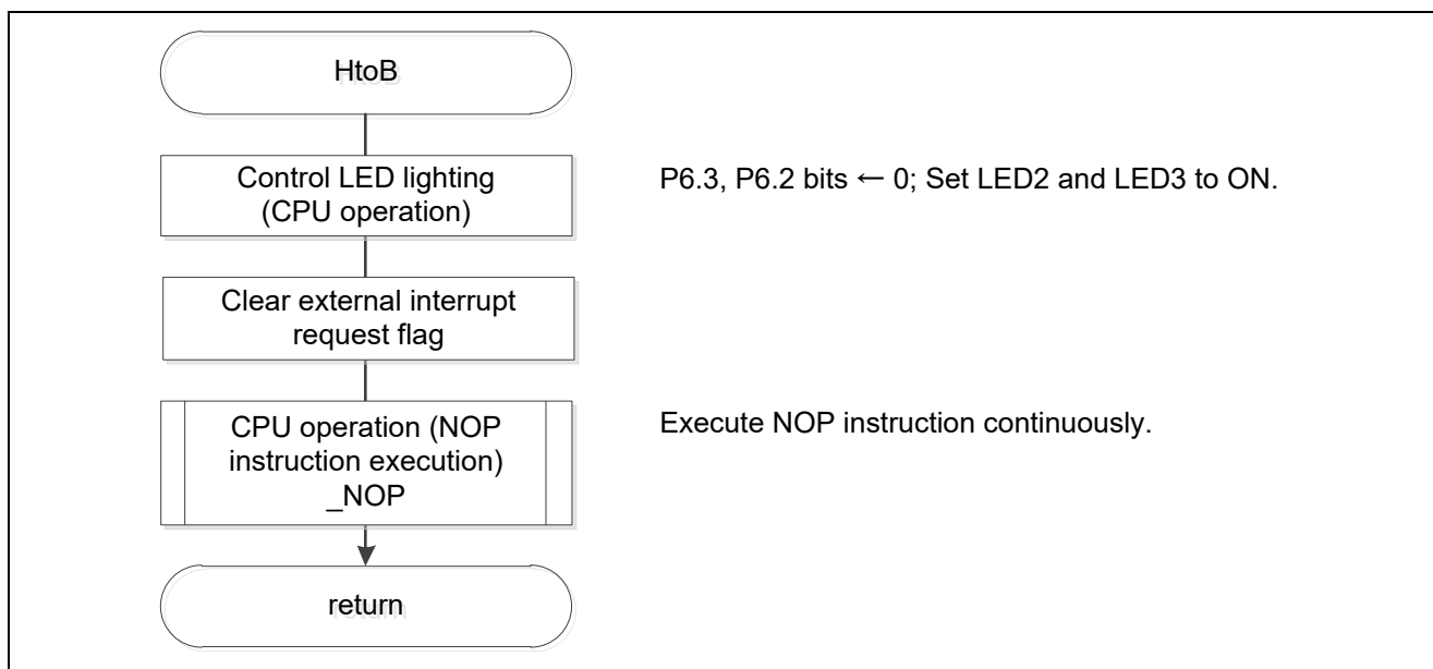
Figure 5.33 Status Transition HtoB
