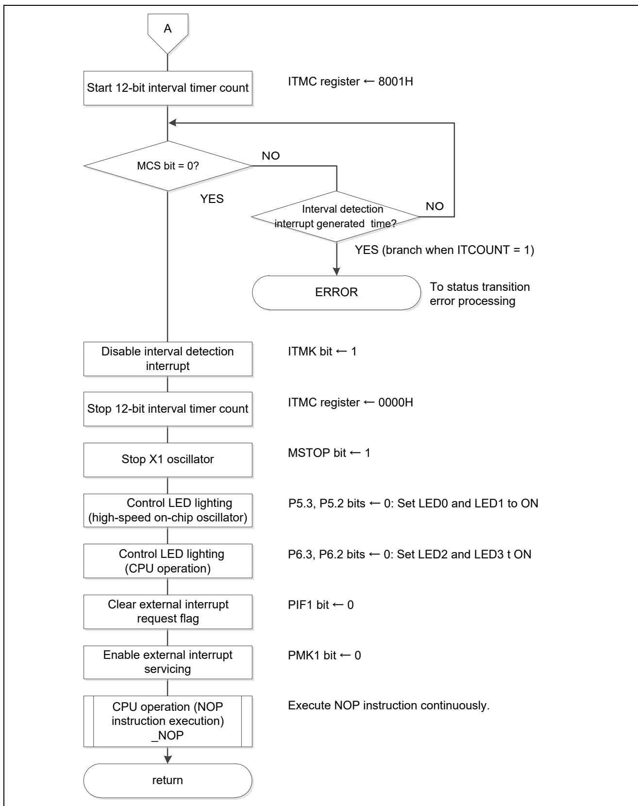
Figure 5.29 Status Transition CtoB(2/2)
