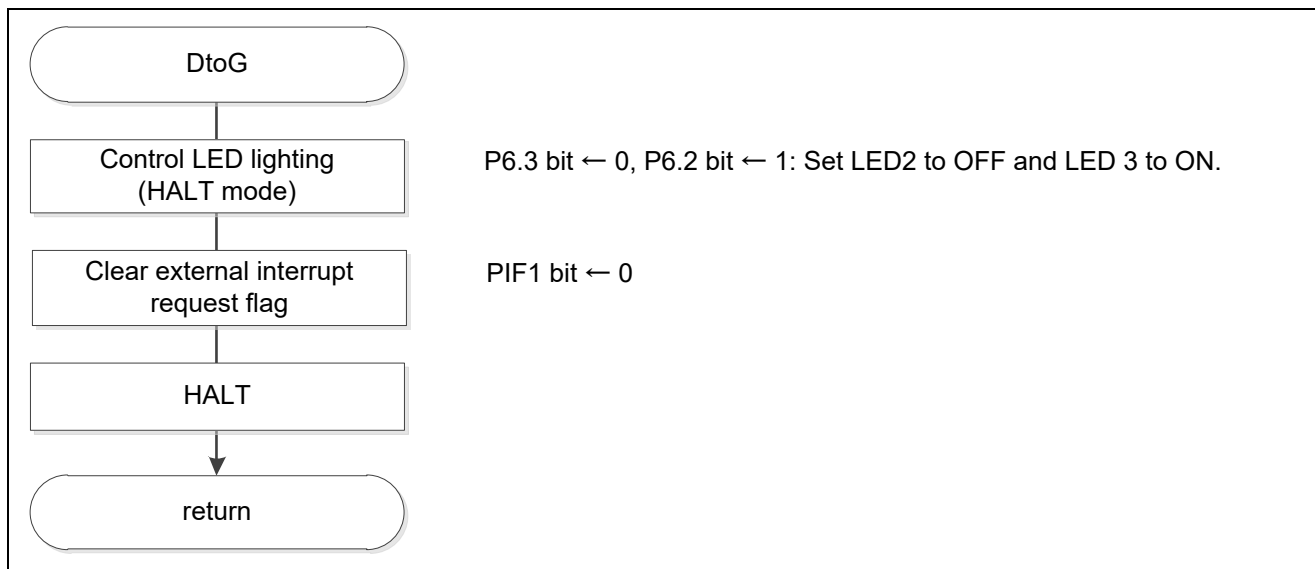
Figure 5.14 Status Transition DtoG
