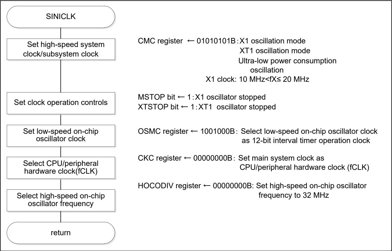
Figure 5.4 Clock Generator Setting
