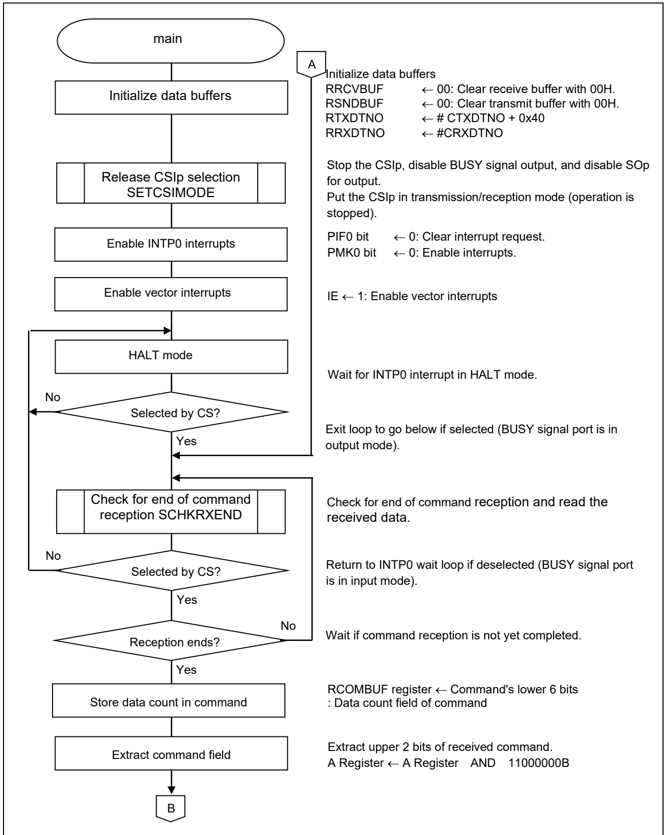
Figure 5.7 Main Processing (1/2)
