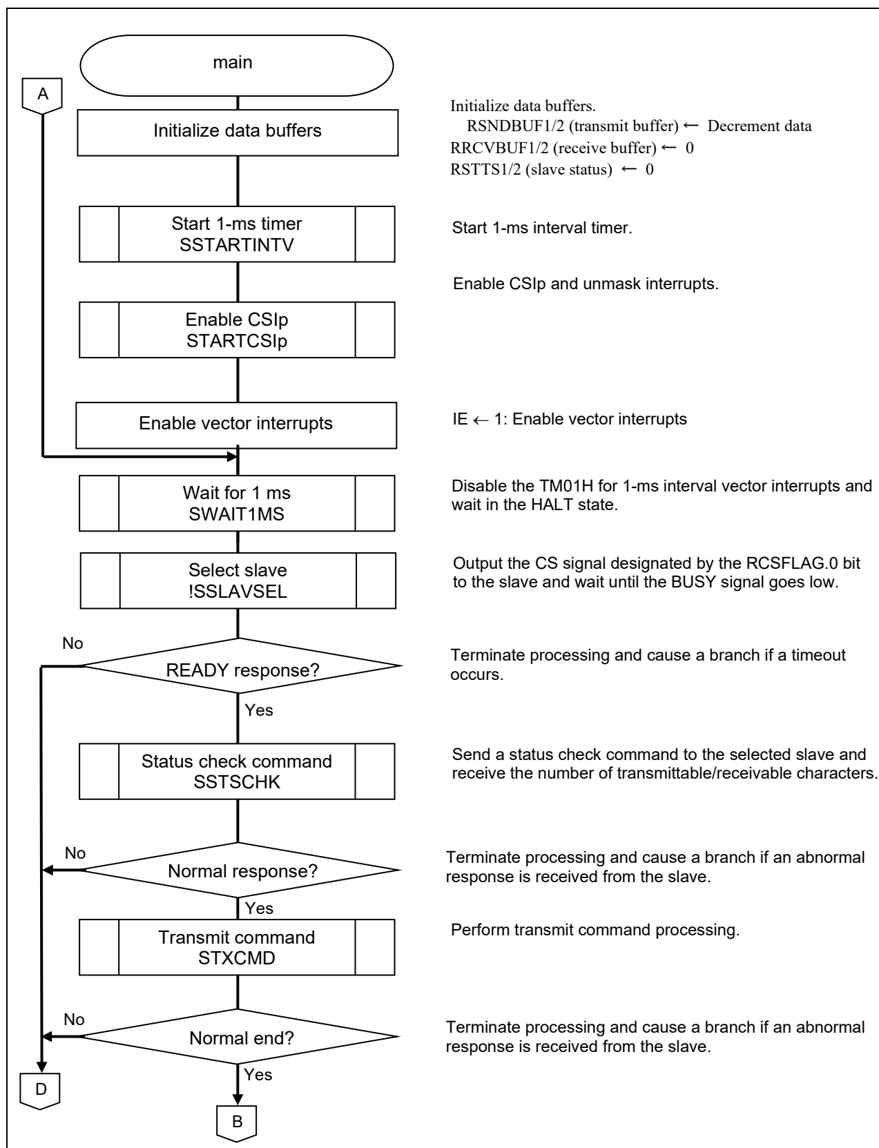
Figure 5.7 Main Processing (1/3)
