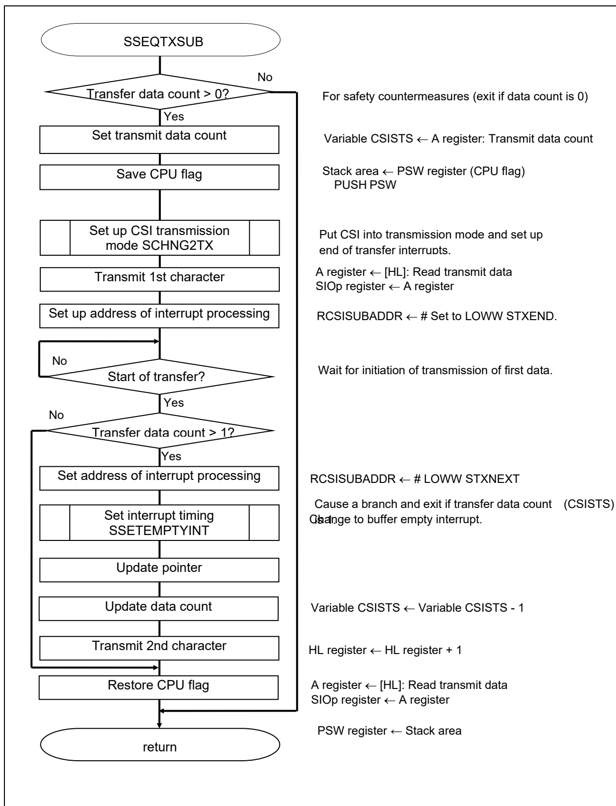
Figure 5.31 Continuous Transmission Start Processing
