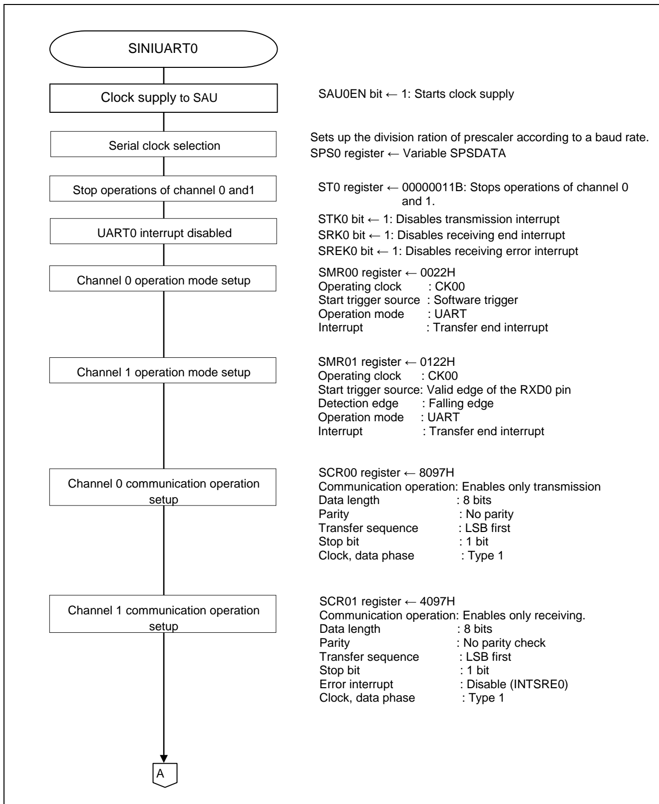
Figure 5.9 Initialization of UART0 (1/2)
