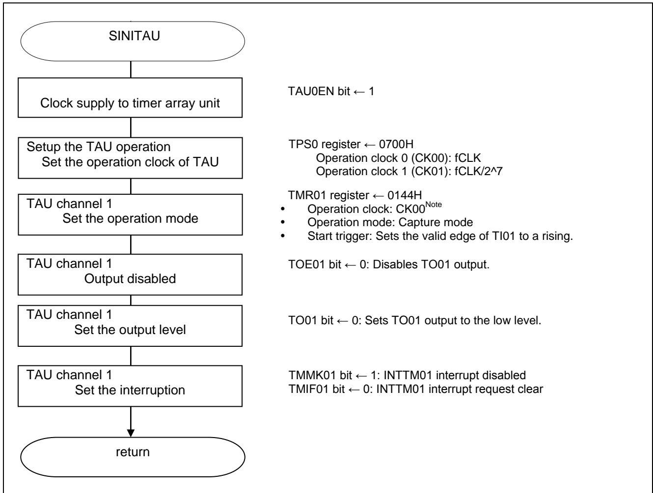
Figure 5.5 Setup of Timer Array Unit
