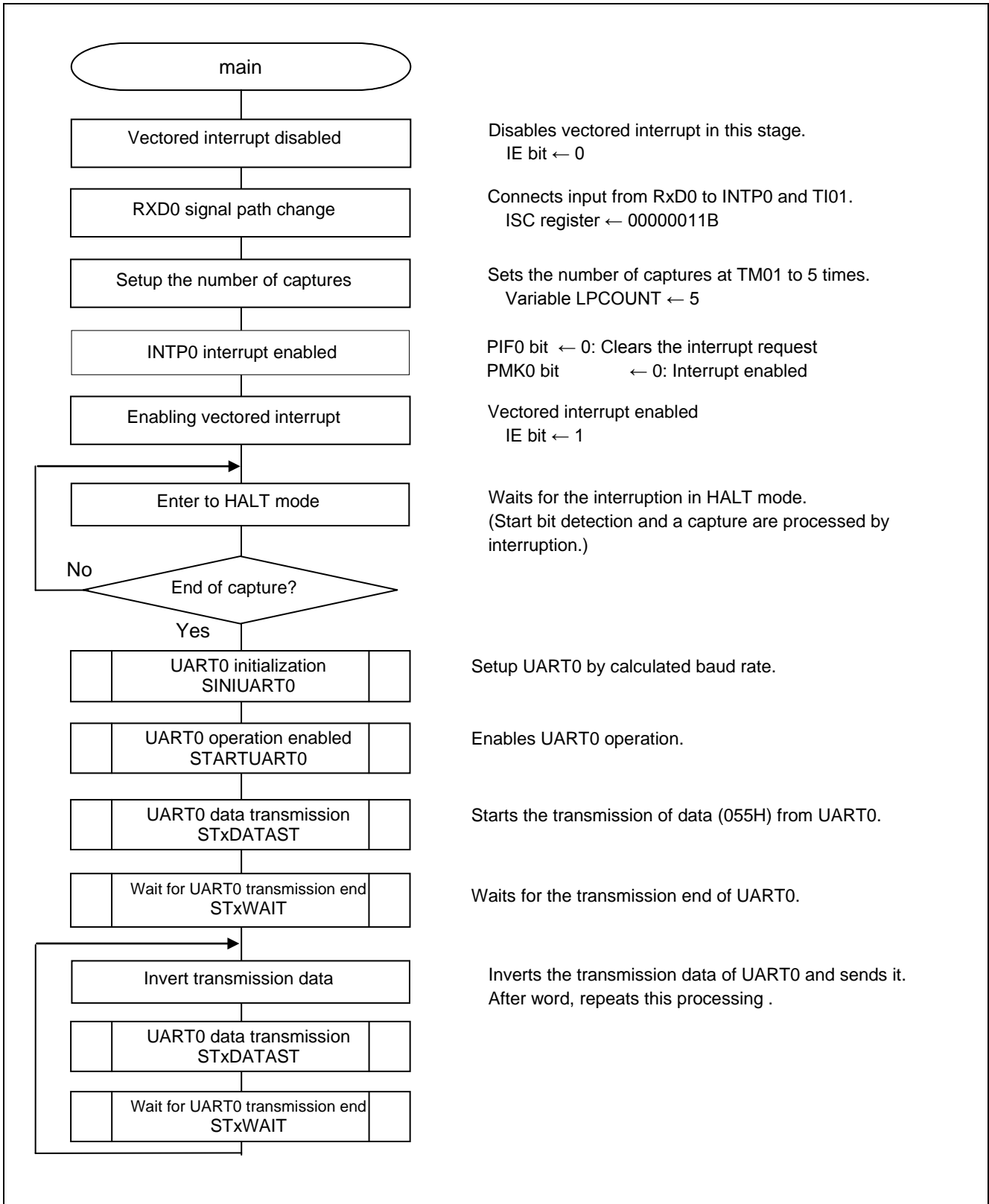
Figure 5.6 Main Processing
