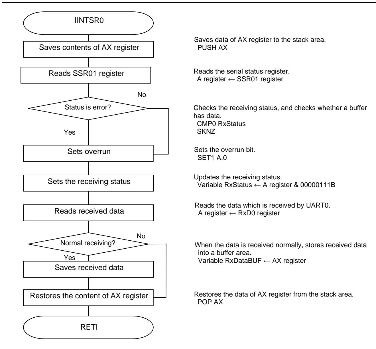
Figure 5.15 Receiving End Interrupt Processing
