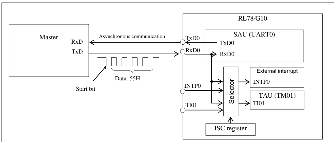
Figure 1.1 Circuit Configuration of Baud Rate Measurement
