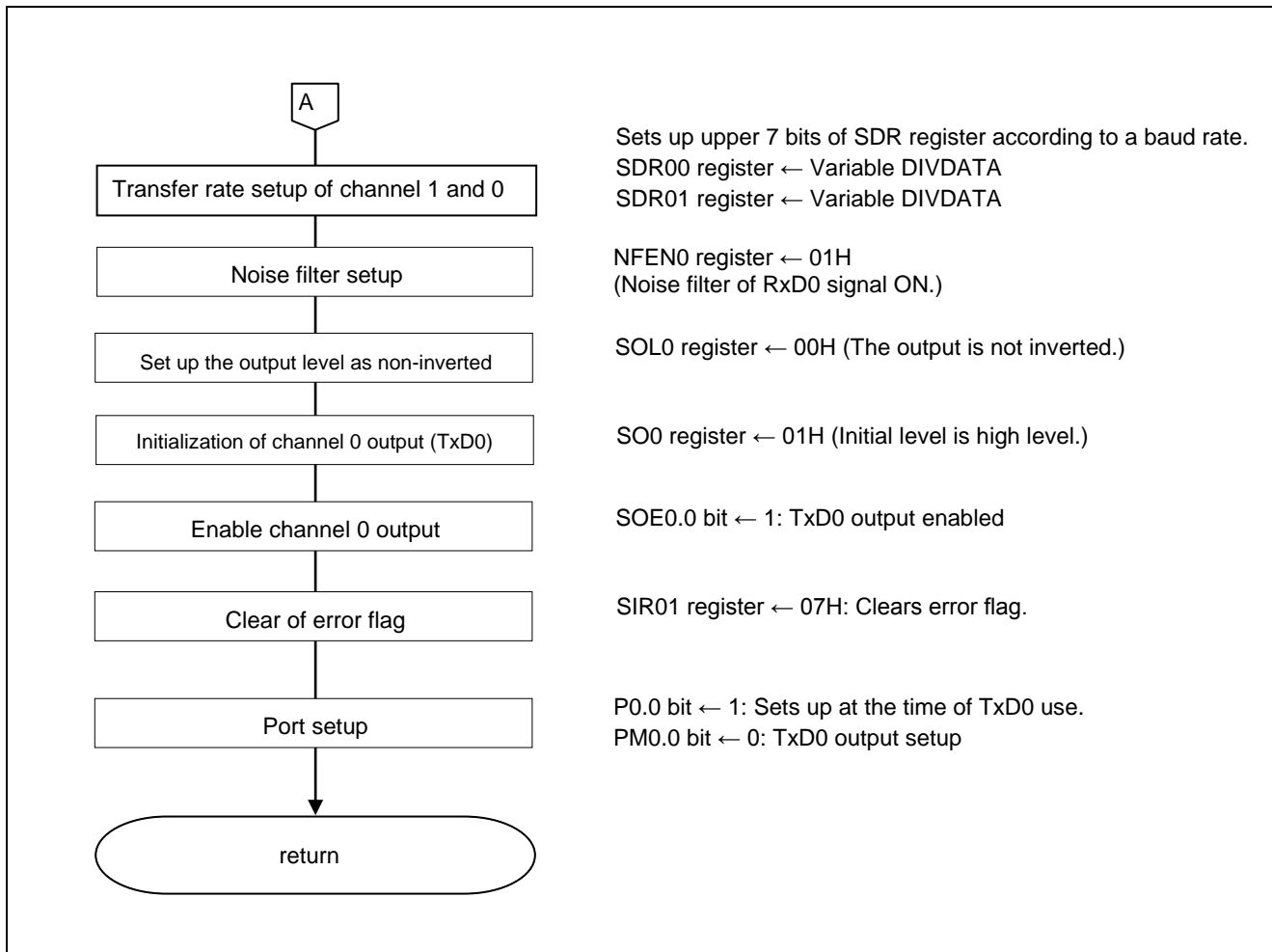
Figure 5.9 Initialization of UART0 (2/2)
