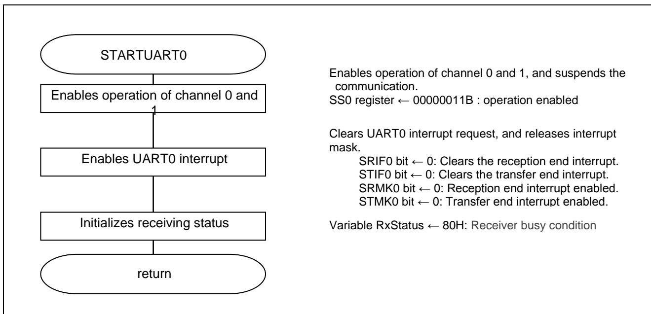
Figure 5.9 Enabling UART0 Operation
