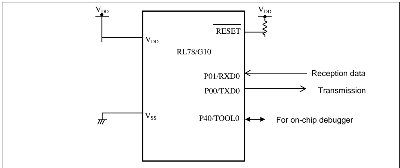
Figure 4.1 Hardware Configuration
