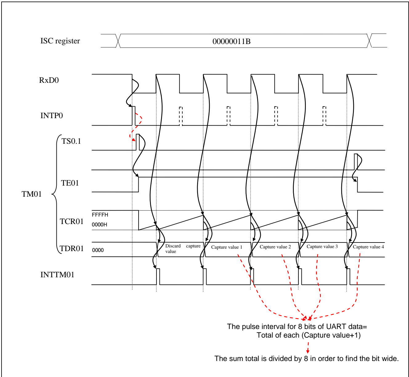
Figure 1.2 Timing Chart of Baud Rate Measurement
