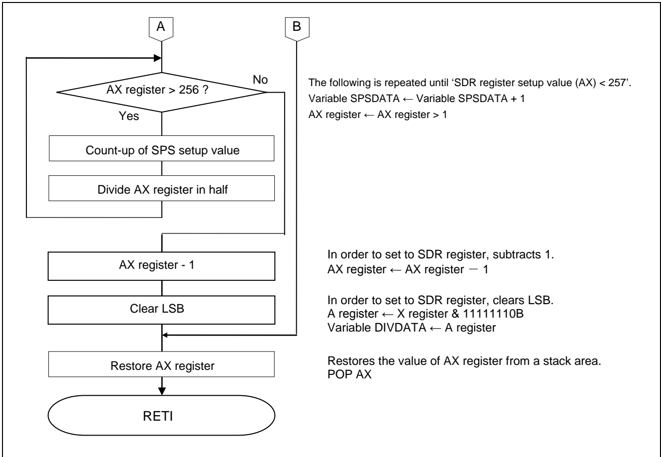
Figure 5.8 Completion of INTTM01 Capture Interrupt Processing (2/2)
