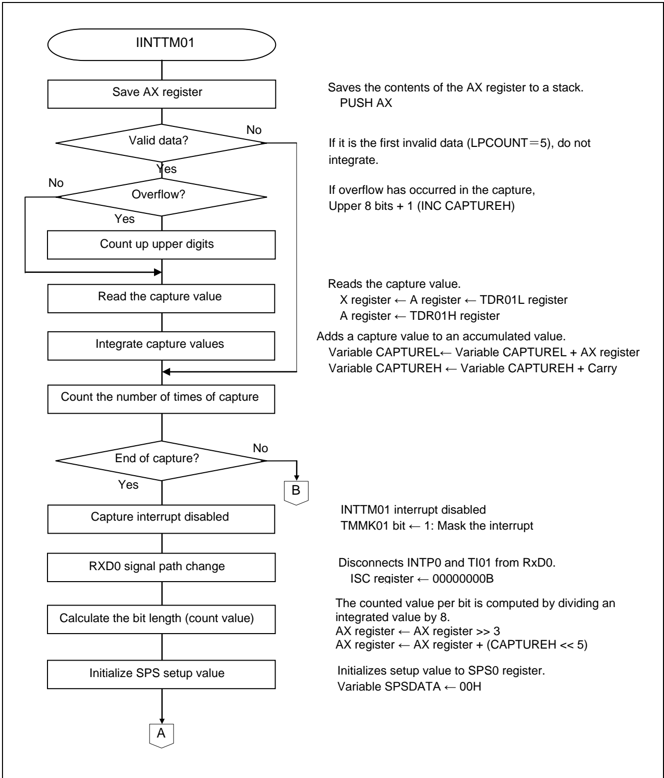
Figure 5.8 Completion of INTTM01 Capture Interrupt Processing (1/2)
