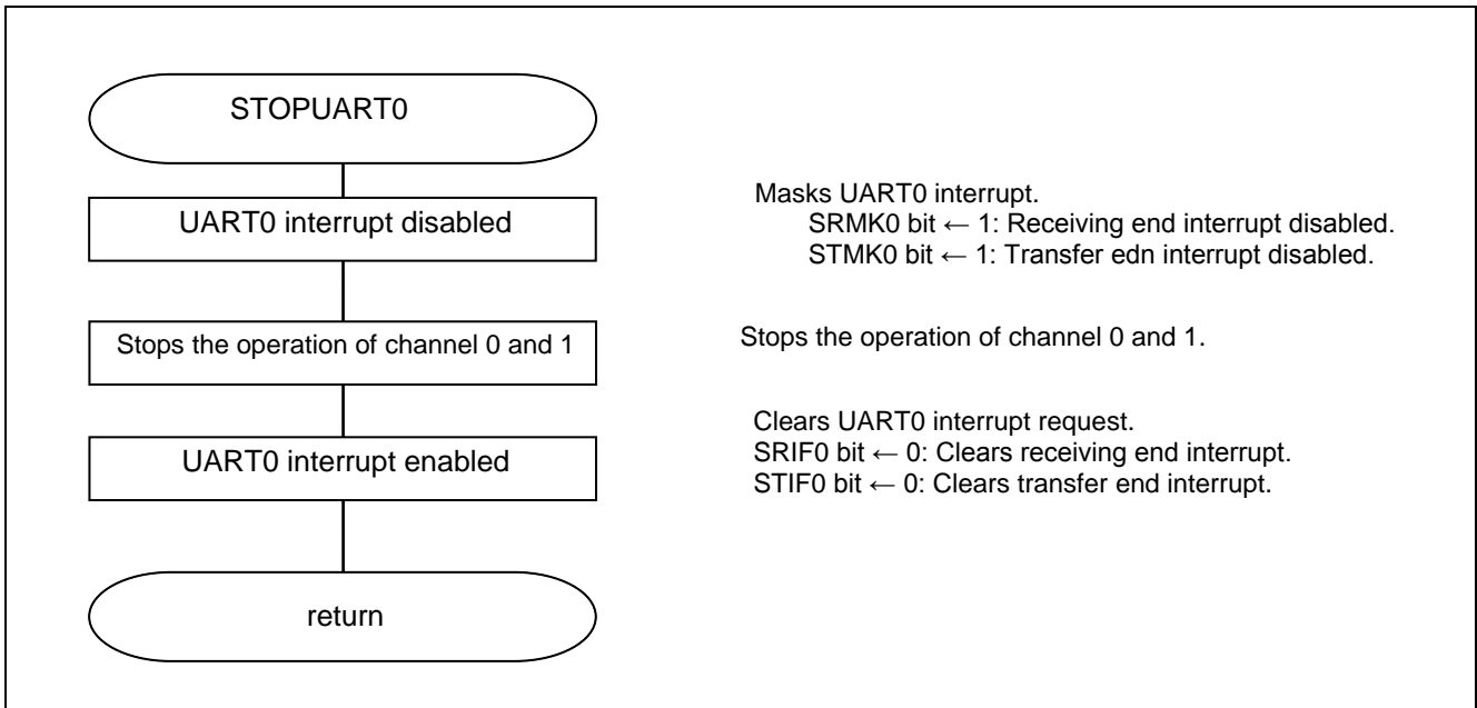
Figure 5.11 UART0 Operation Disabled
