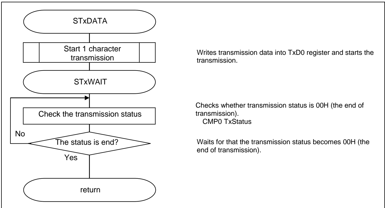
Figure 5.13 1 Character Transmission/Wait for the End of Transmission Processing
