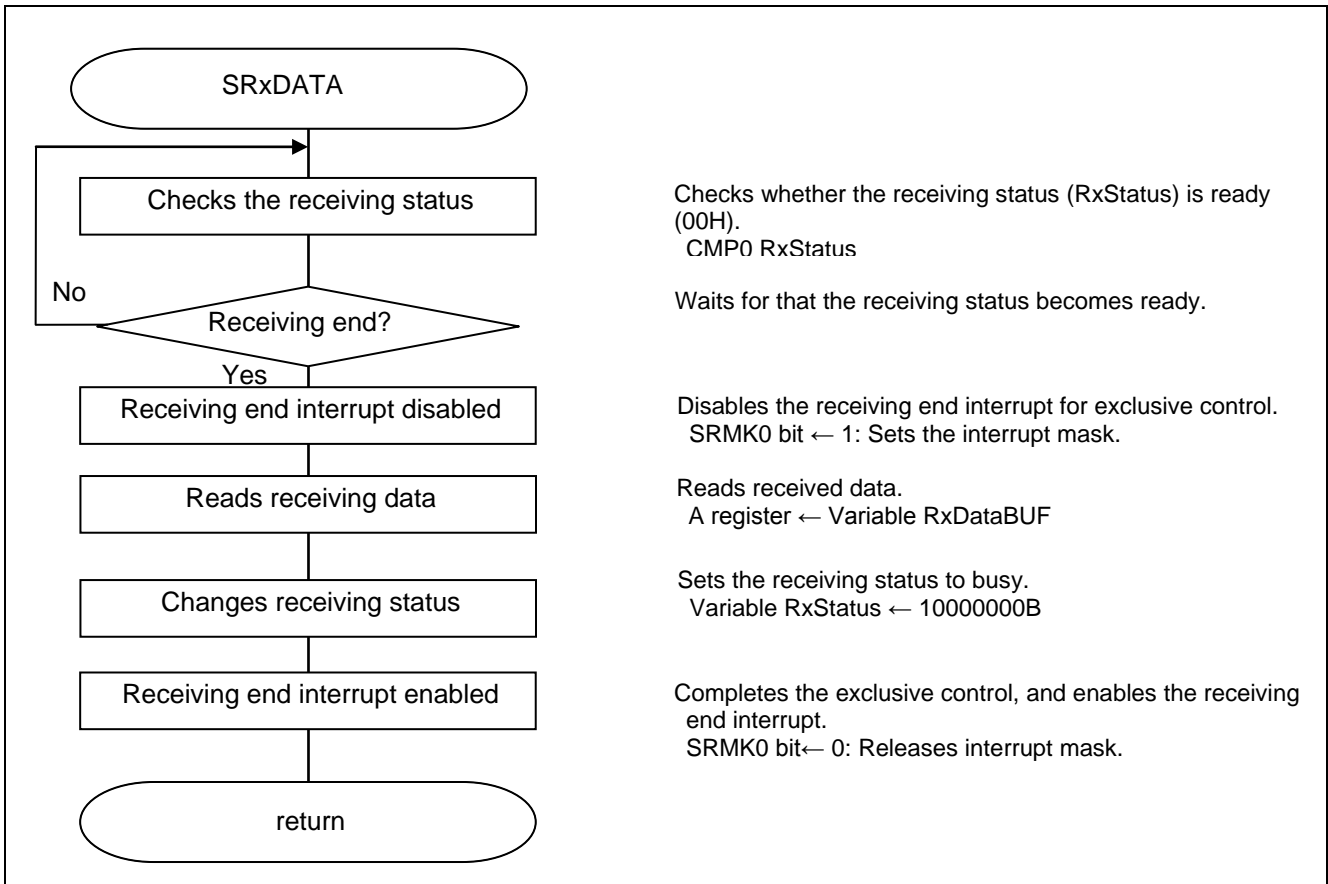
Figure 5.14 1 Character Receiving Processing
