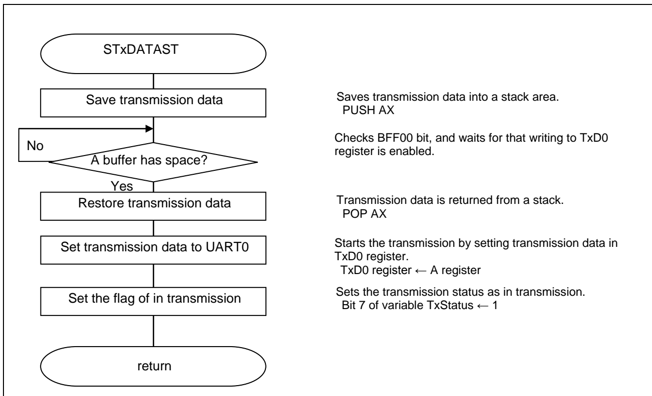
Figure 5.12 1 Character Transmission Start Processing
