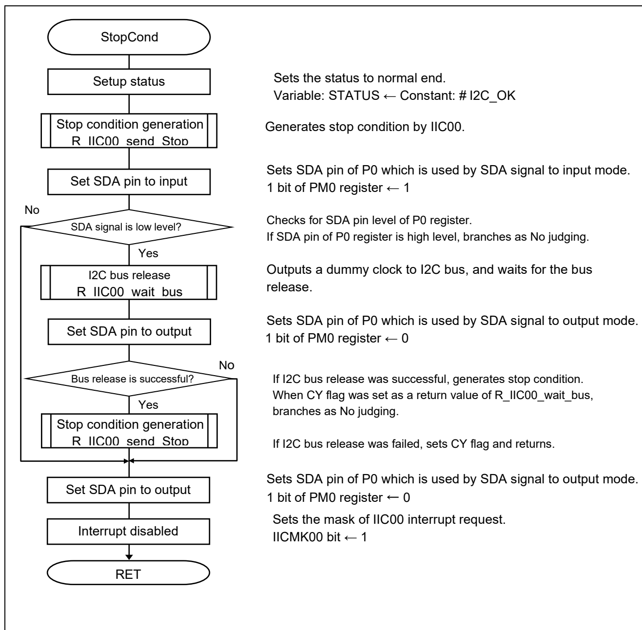
Figure 5.32 Stop Condition Execution
