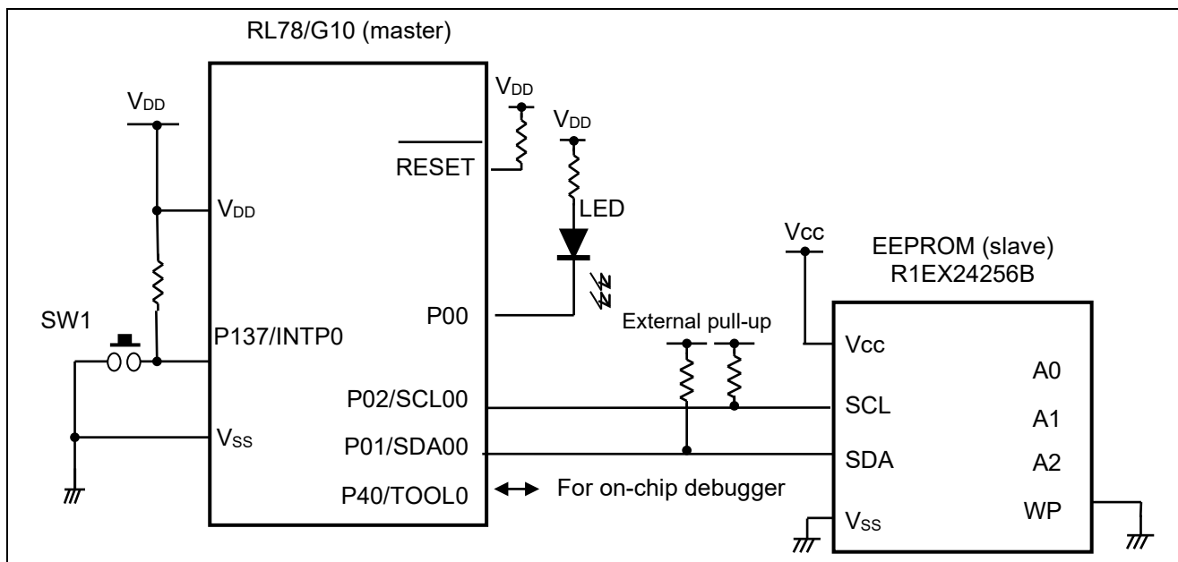
Figure 4.1 Hardware Configuration
