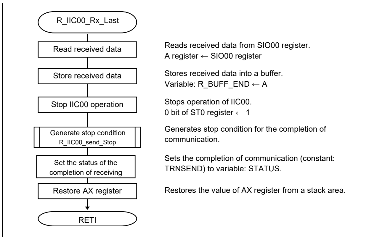
Figure 5.22 Final Data Reception Processing
