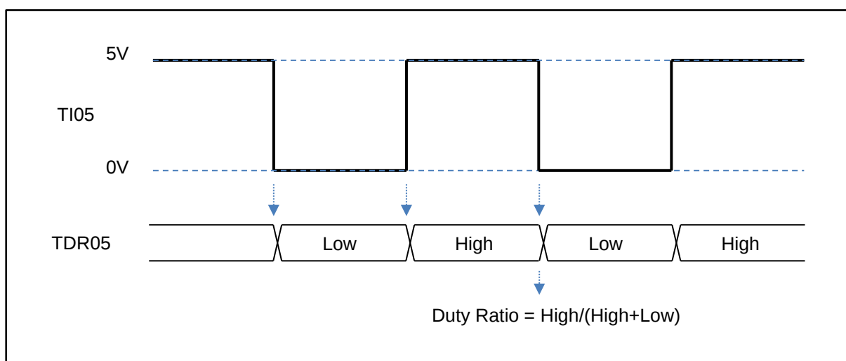
Figure 4-2. PWM Duty Ratio Measurement Method
