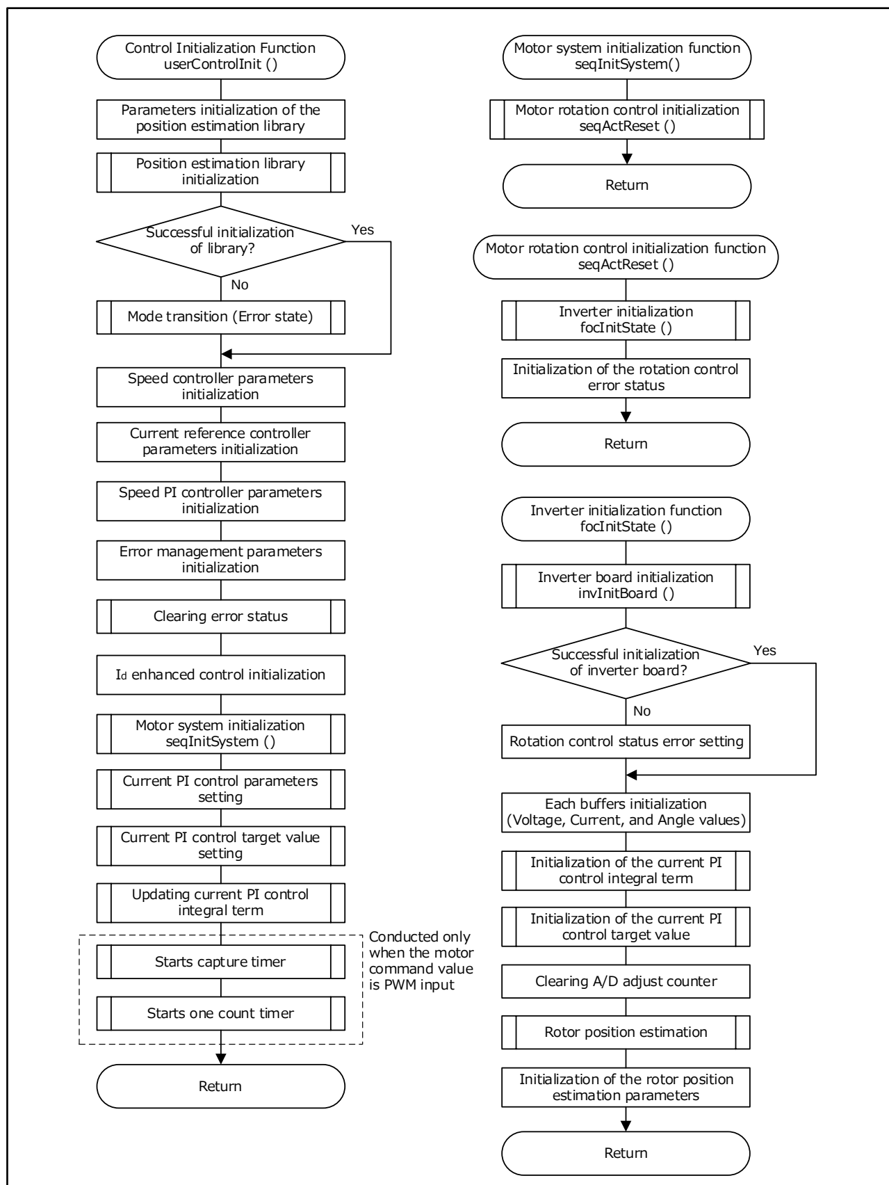
Figure 4-11. Control Initialization Function
