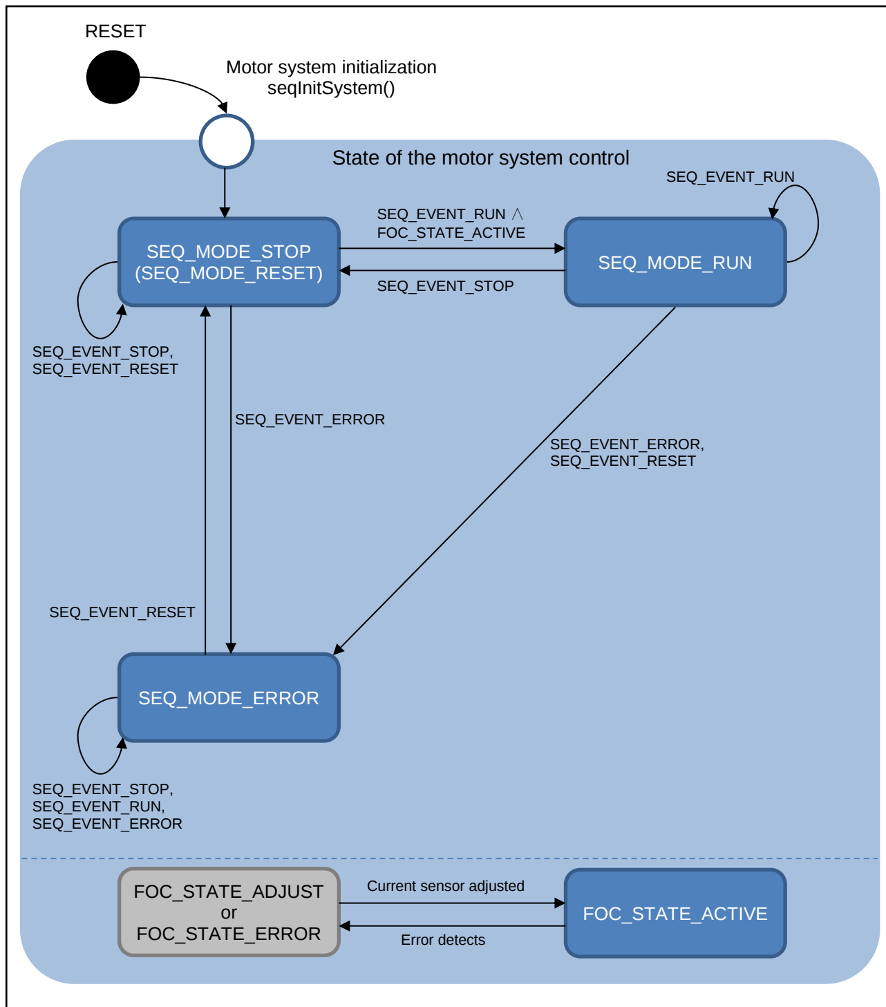
Figure 4-8. State Transition Diagram of the Motor System
