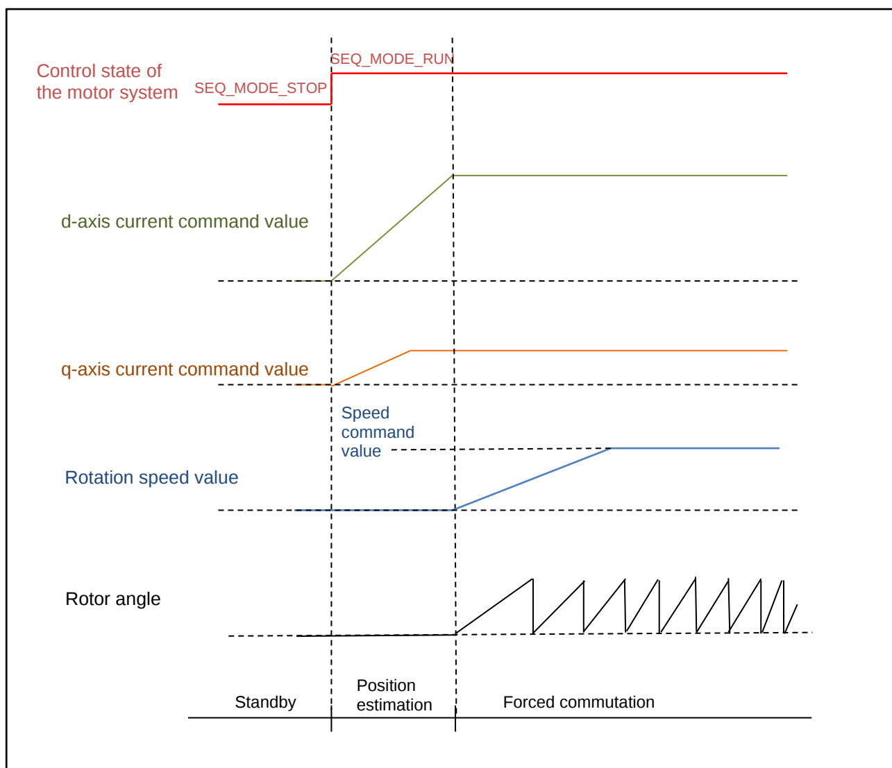
Figure 4-4. Operation Image of Synchronous Operation
