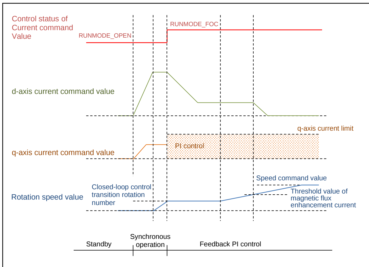
Figure 4-5. Operation Image of the Speed Control
