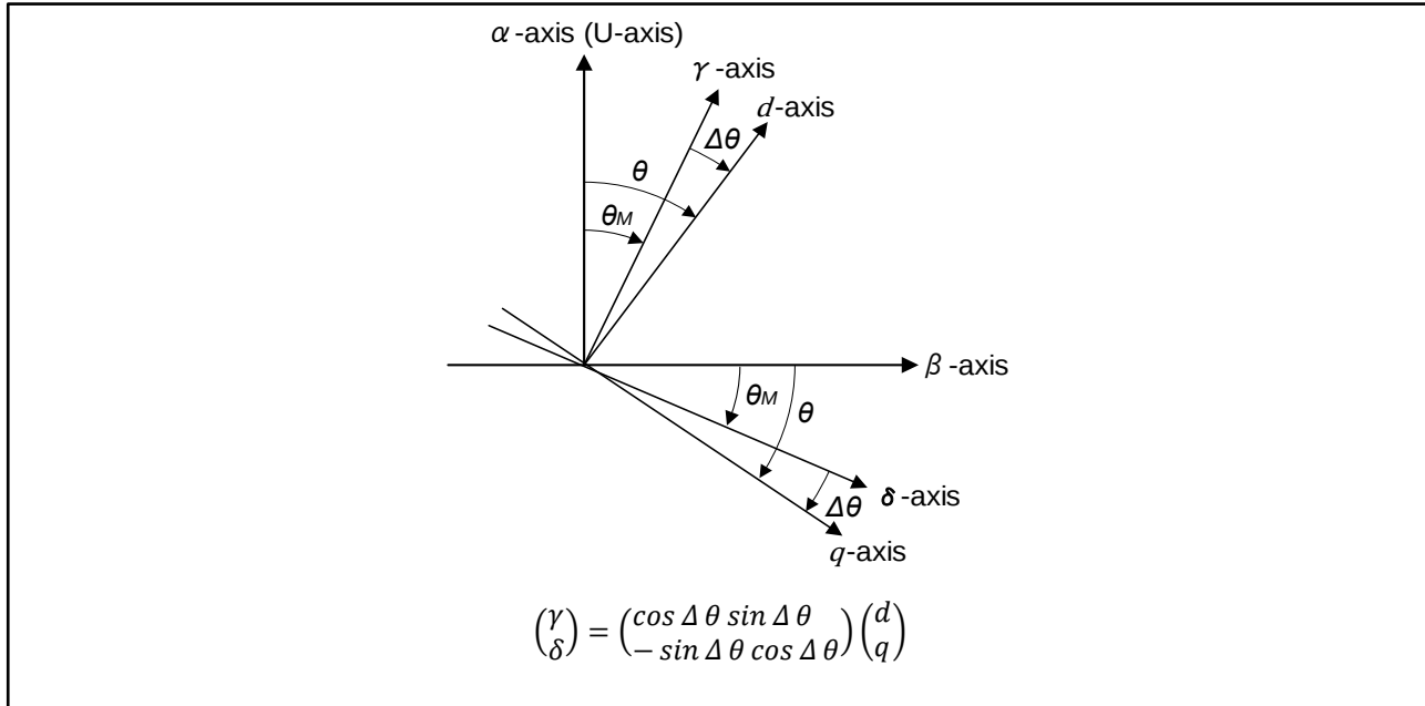
Figure 3-4. Relation Between d/q-axis and \gamma/\delta -axis
