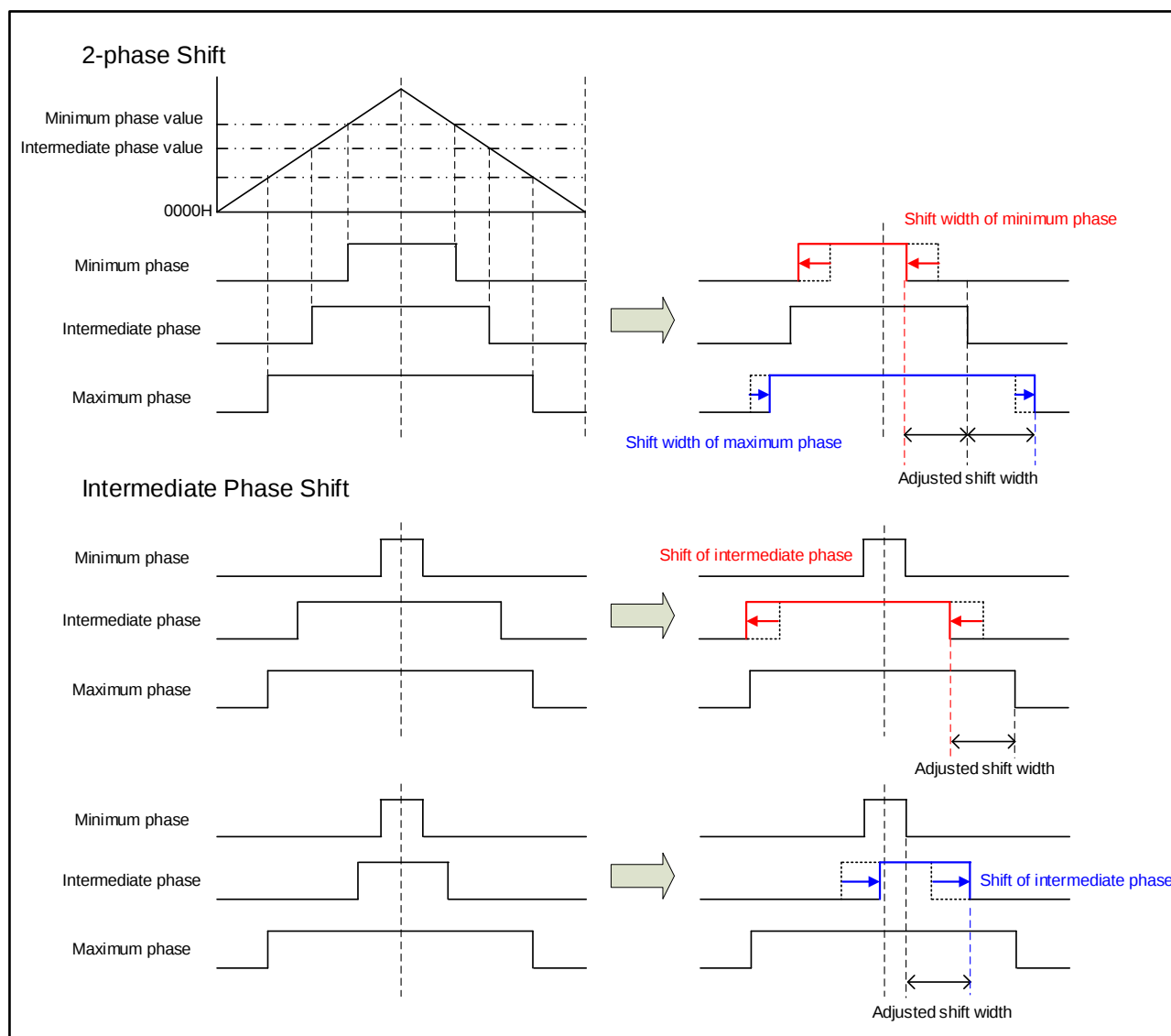
Figure 2-6. Example of the PWM Waveform Output Shift Process
