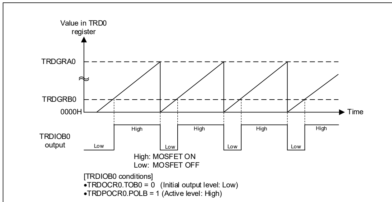
Figure 2-1 DC/DC Gate Control Example
