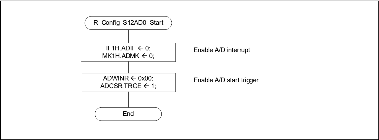
Figure 2-13 A/D Converter Start Flowchart
