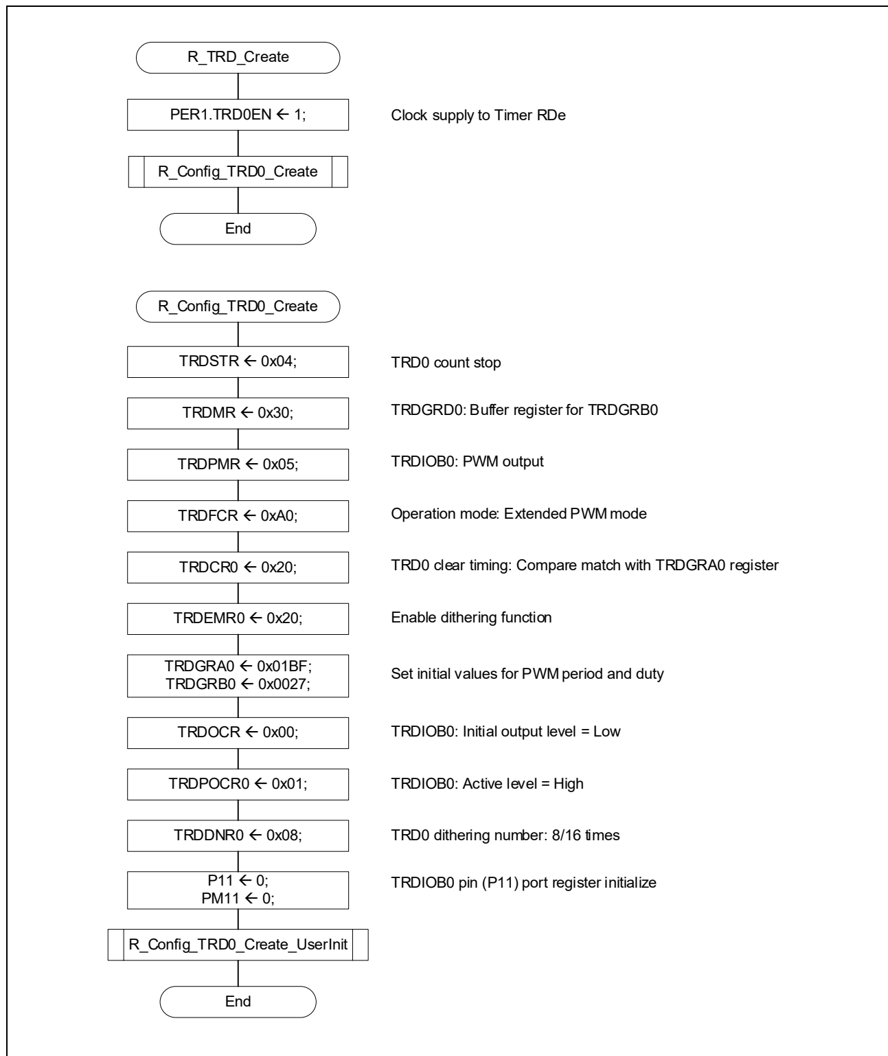
Figure 2-7 Initialize Timer Flowchart
