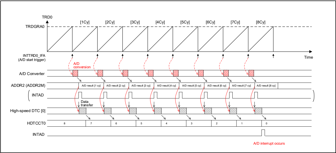
Figure 2-2 A/D Acquisition Image of Control Software
