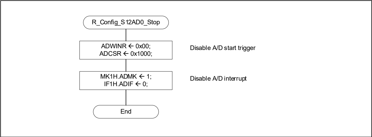
Figure 2-14 A/D Converter Stop Flowchart
