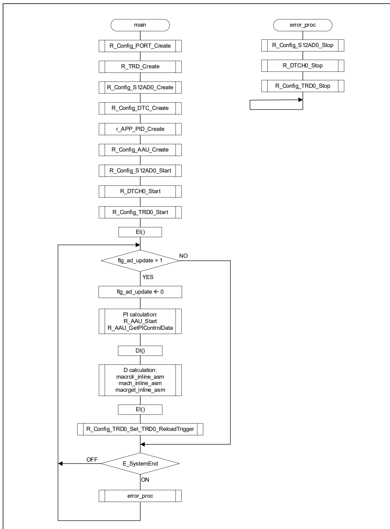
Figure 2-5 System Control Flowchart
