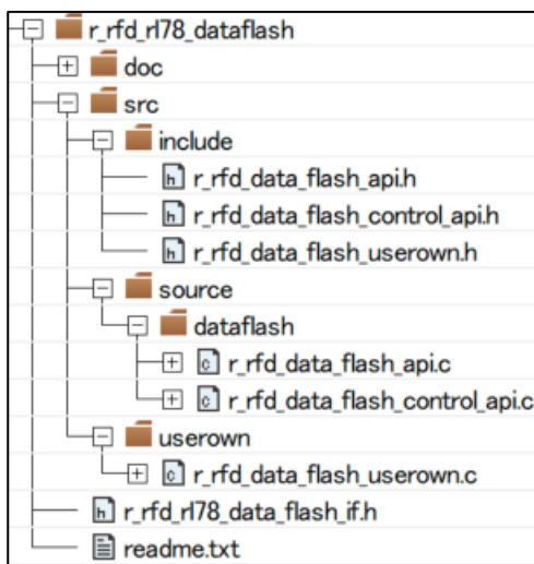
The developed r_rfd_rl78_dataflash folder
