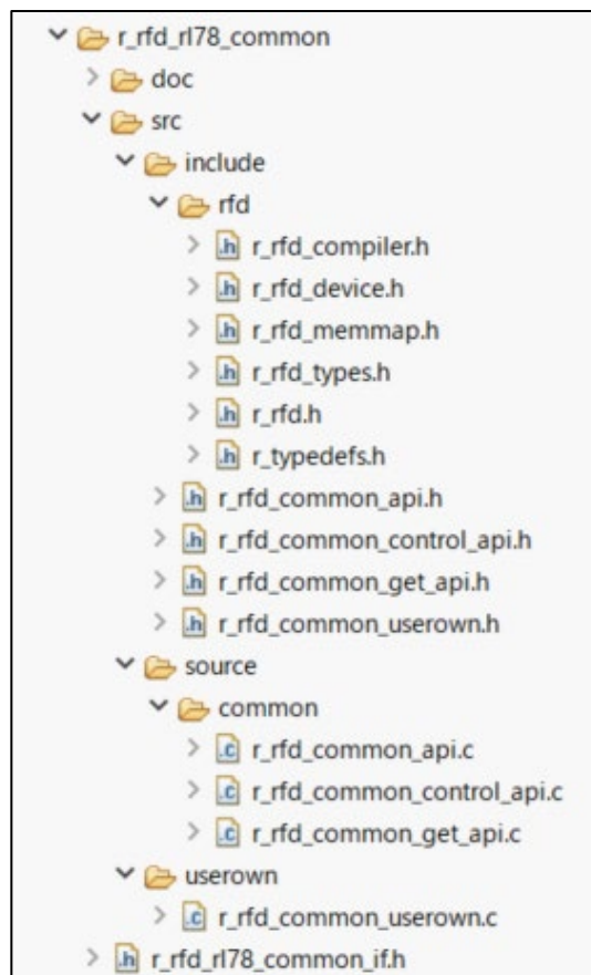
The developed r_rfd_rl78_common folder
