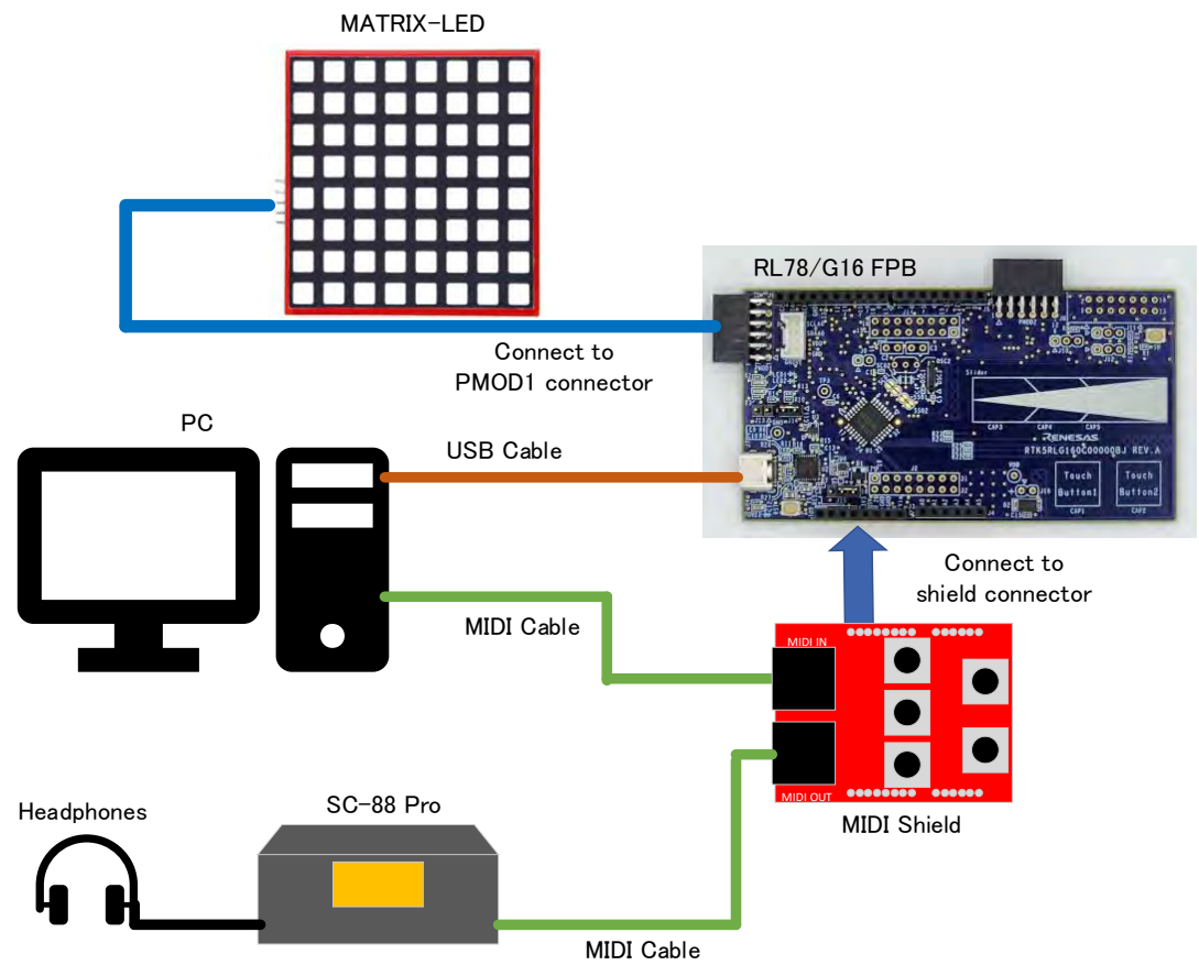
Figure 2-1 Hardware Configuration
