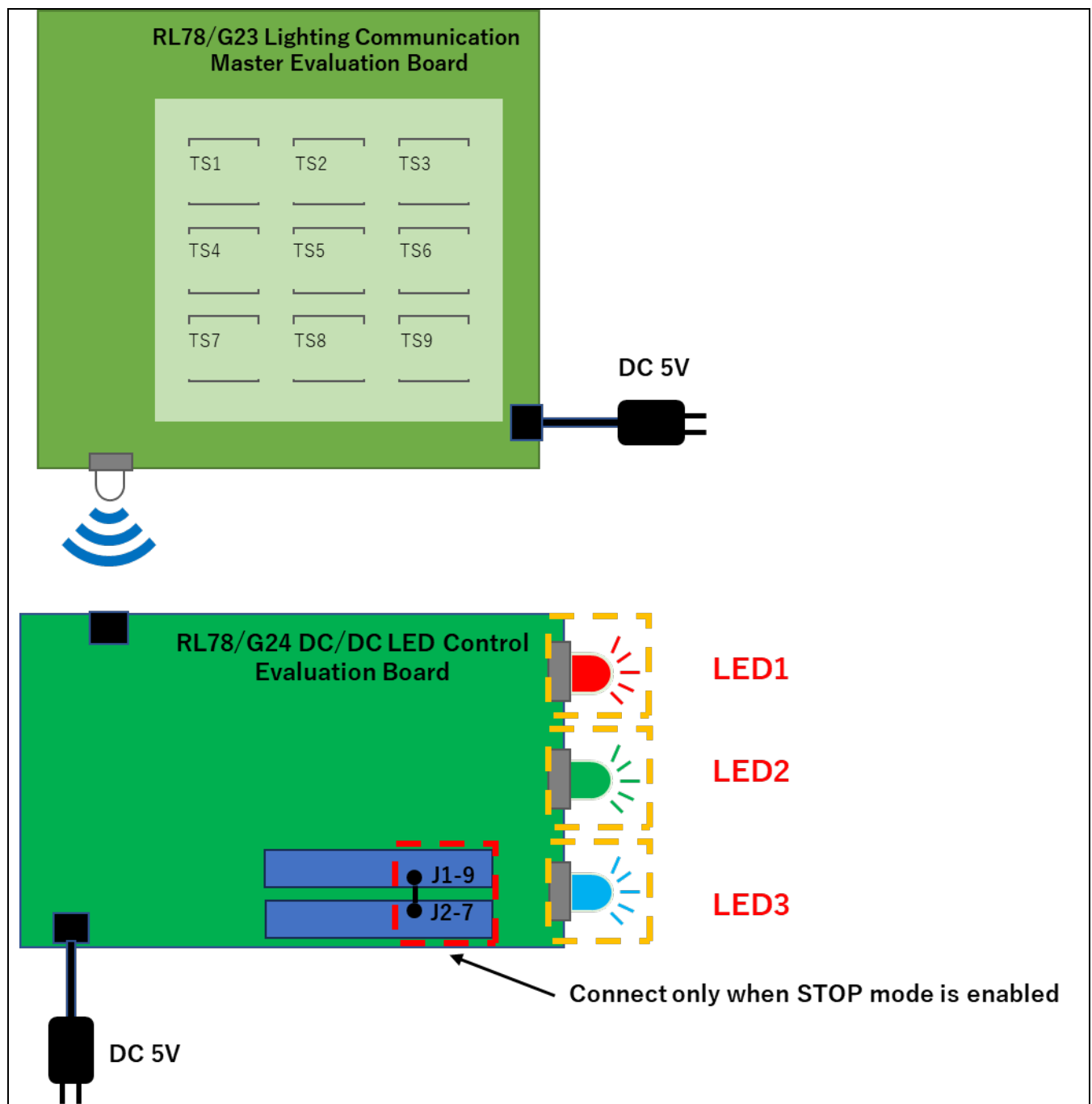
illustration 3-1System Configuration Diagram
