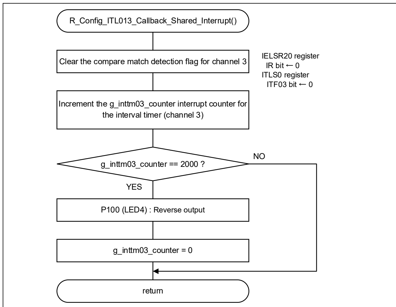
Figure 4.6 Interrupt Processing for Interval Timer Channel 3
