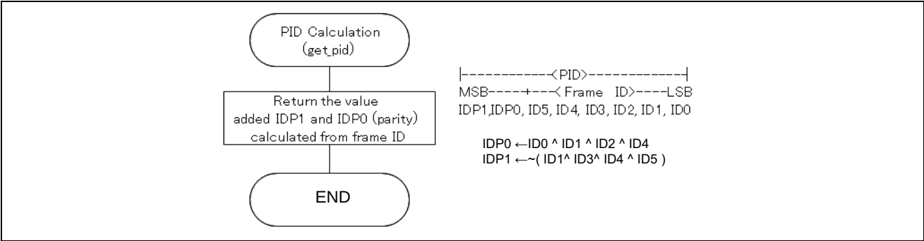
Figure 2-19 PID Calculation
