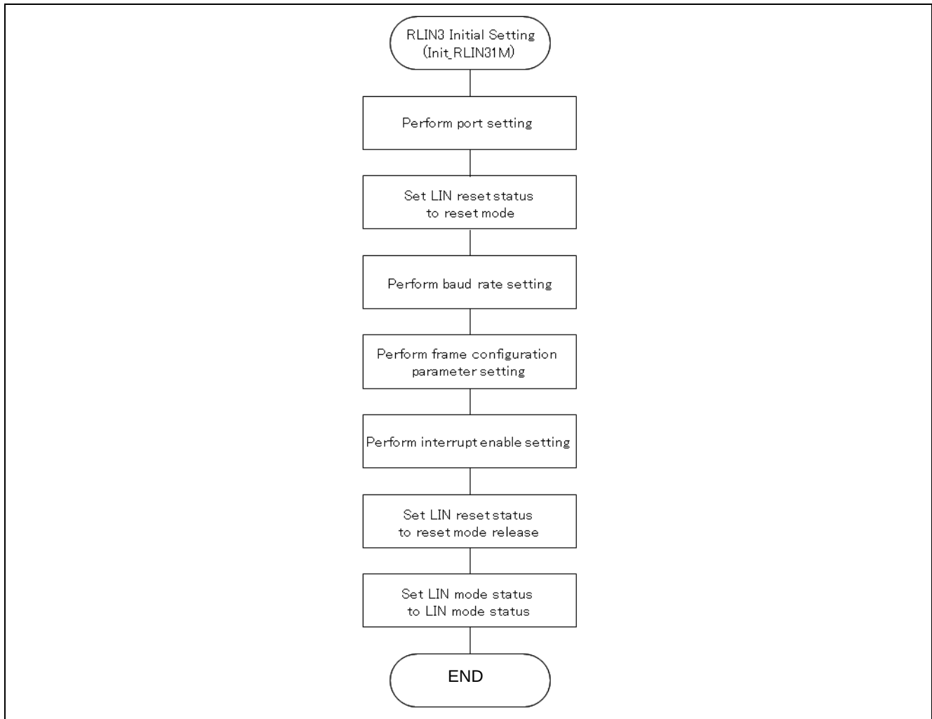
Figure 2-16 RLIN31 Initial Setting
