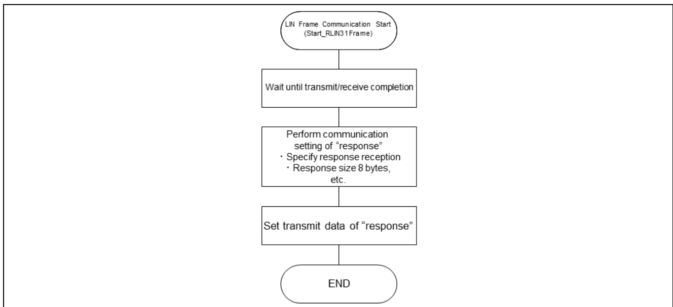
Figure 2-18 RLIN31 Frame Communication Start
