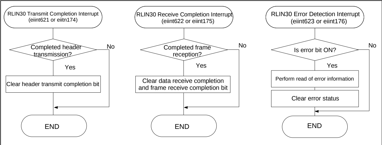
Figure 2-20 RLIN30 Interrupt Handlers
