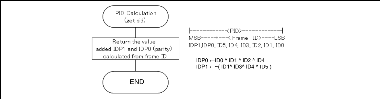
Figure 2-7 PID Calculation
