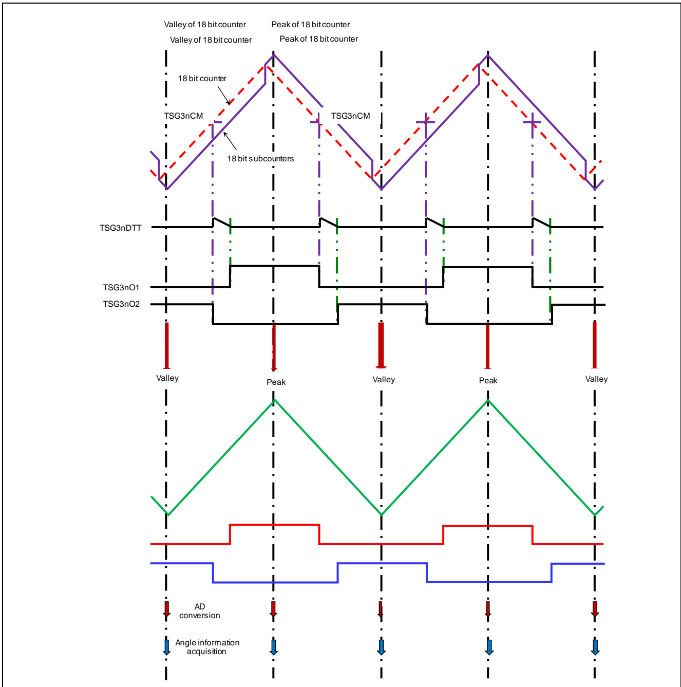
Figure 2-12 Operation overview
