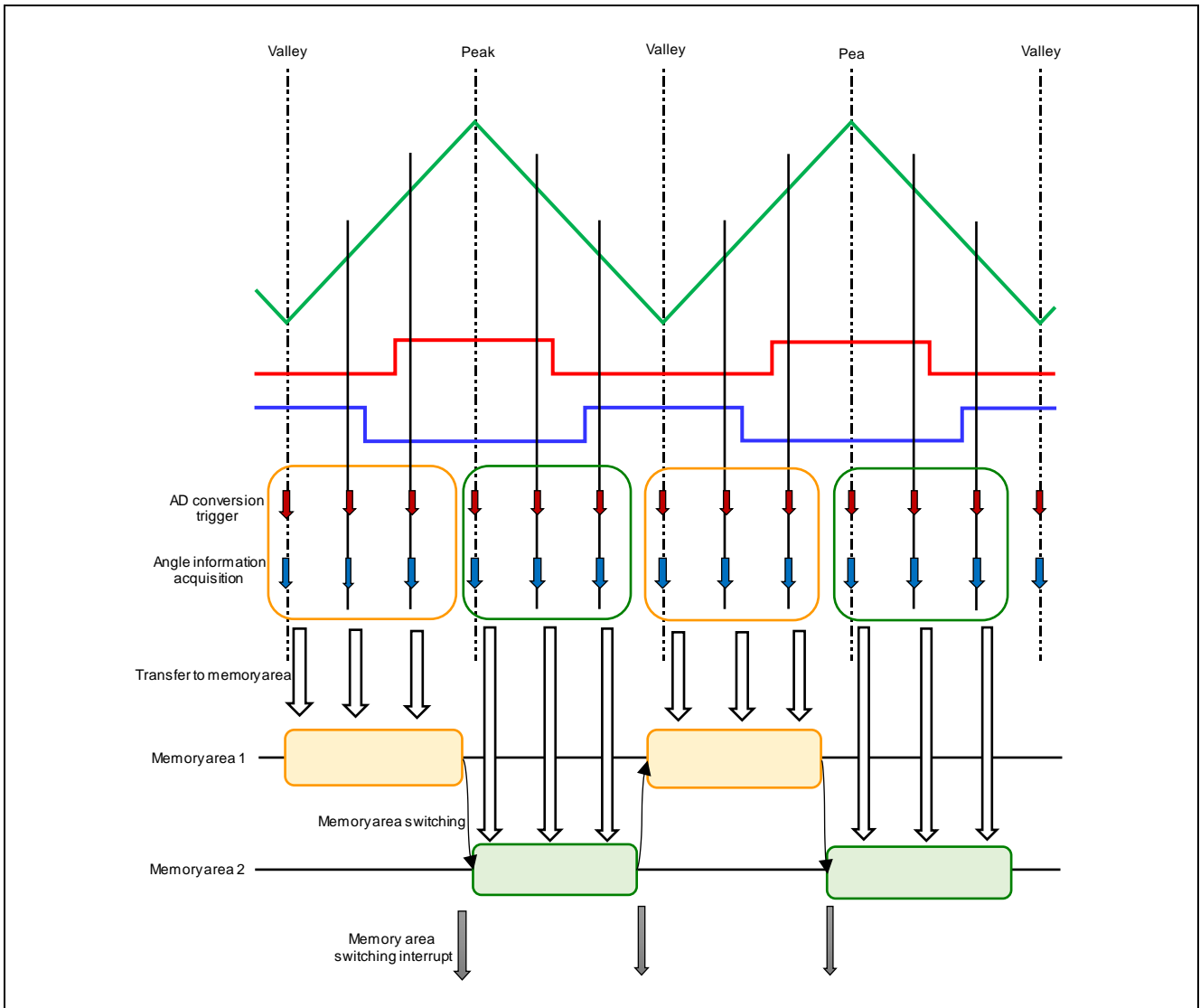
Figure 2-18 Operation overview
