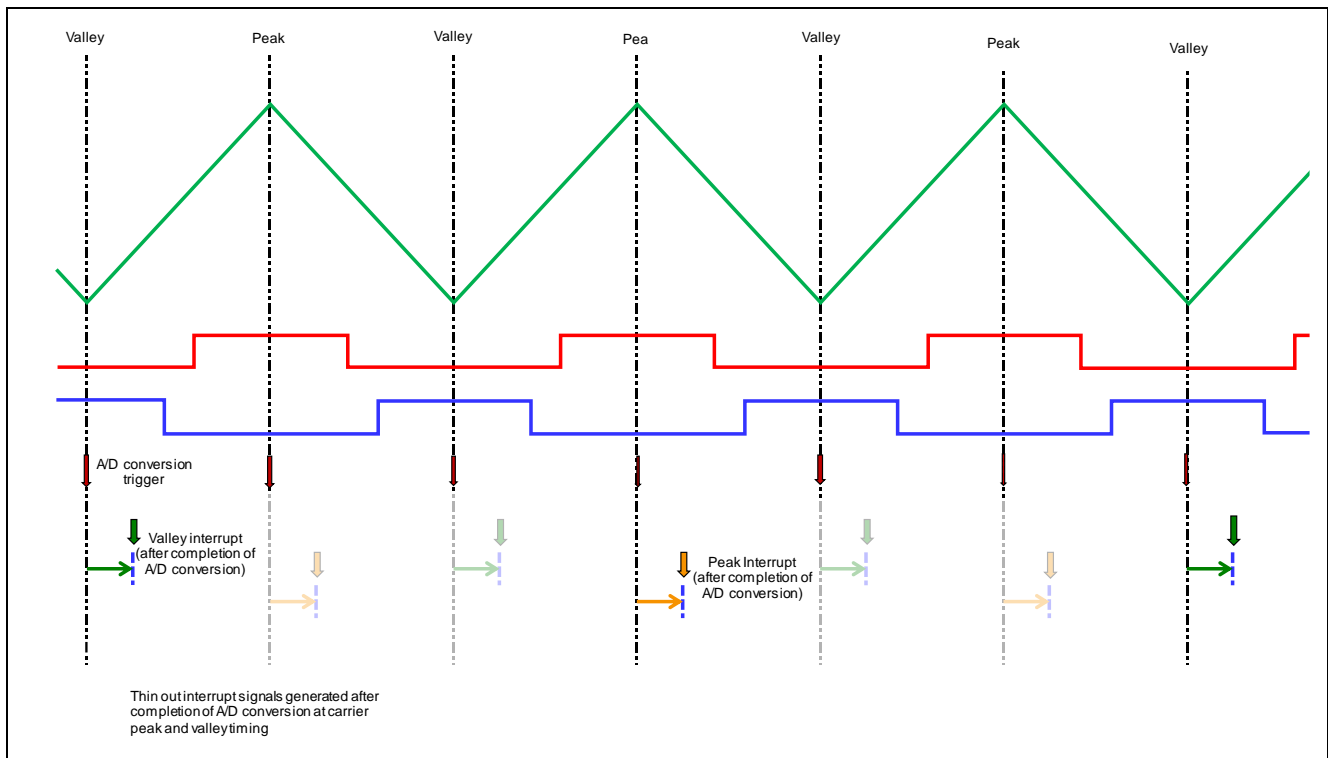
Figure 2-22 Operation overview
