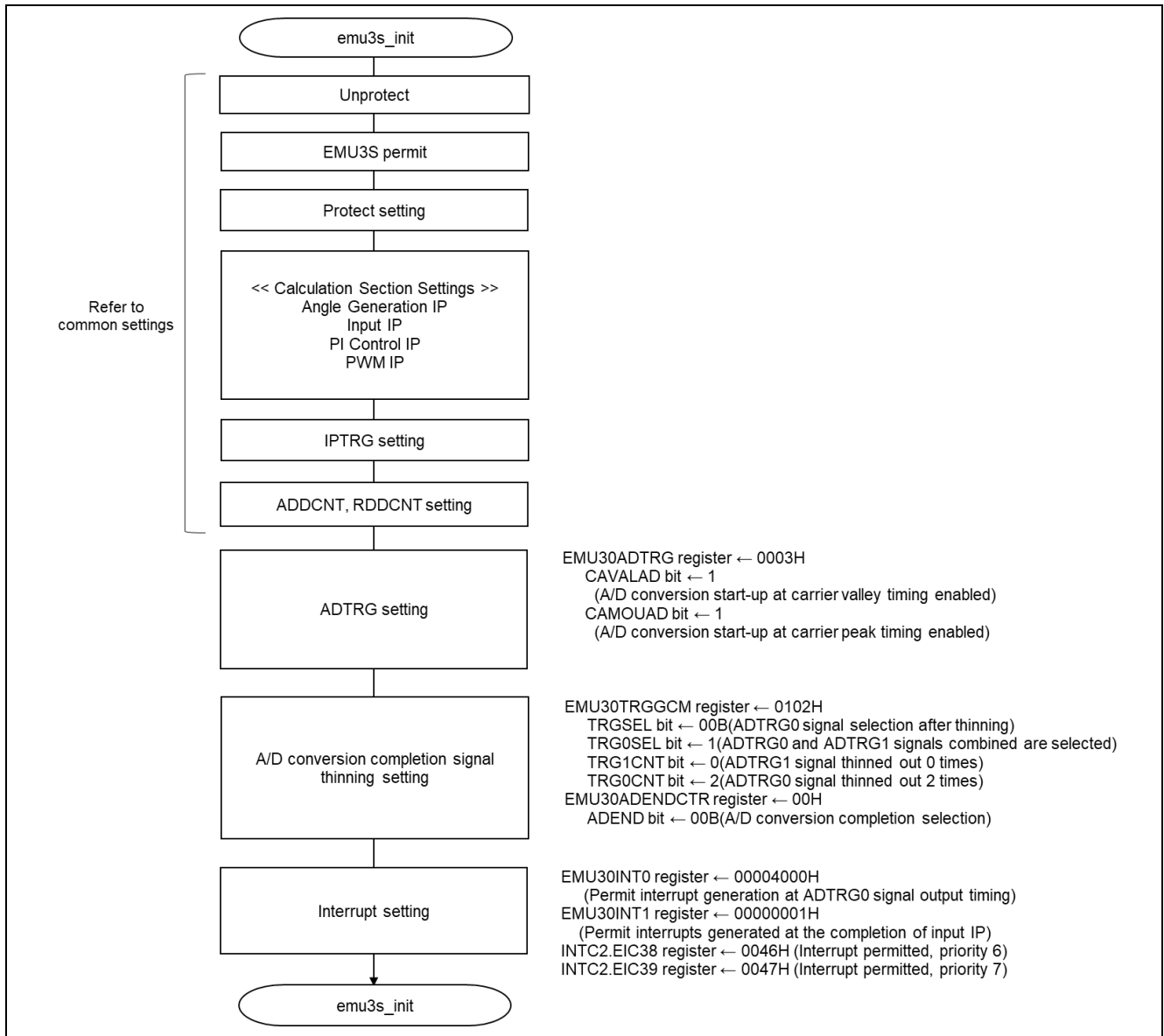
Figure 2-23 Operation flow
