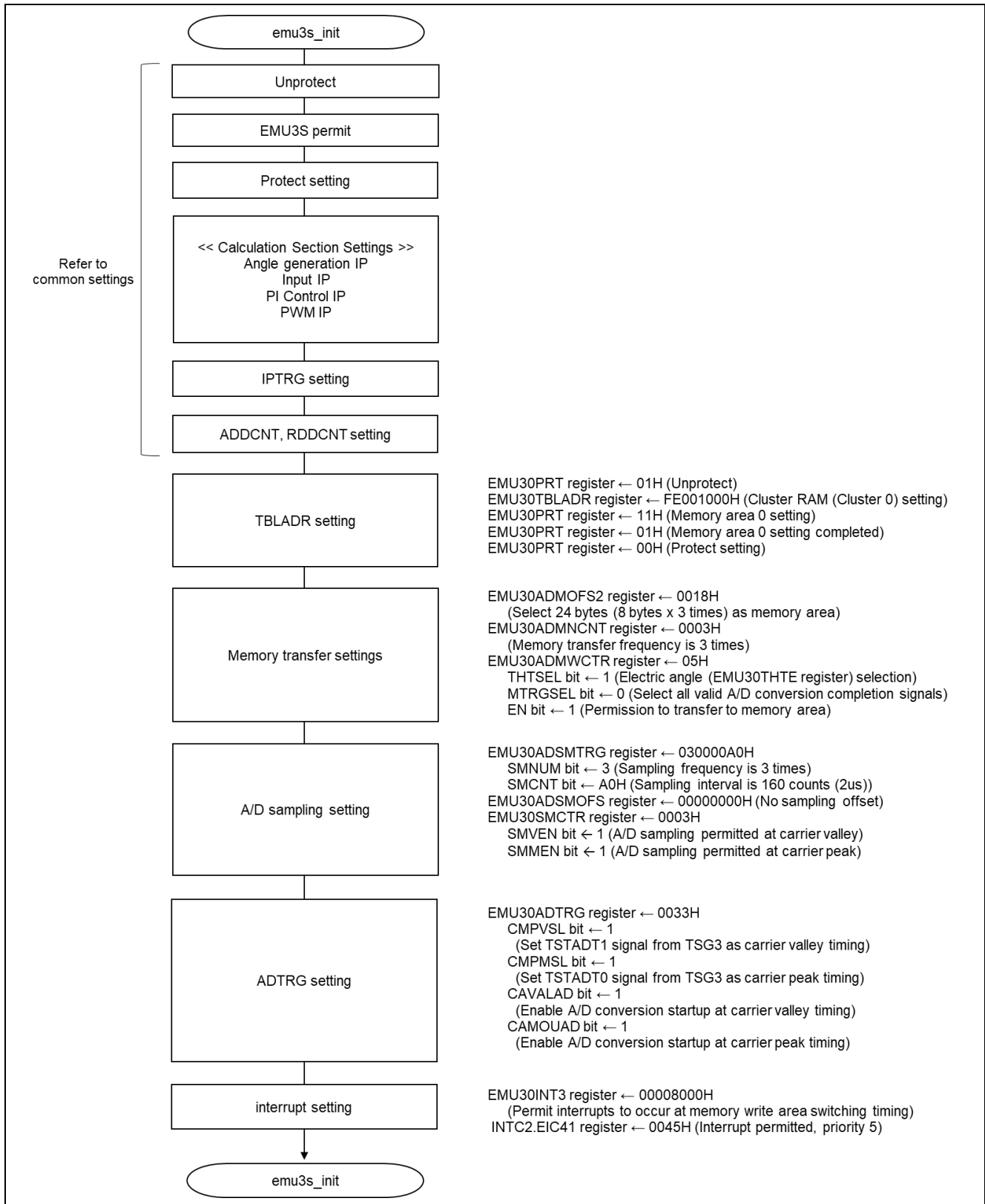
Figure 2-20 Operation flow
