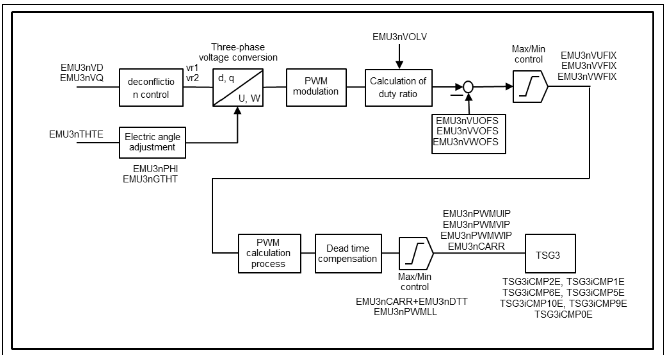
Figure 2-5 Block diagram of PWM IP
