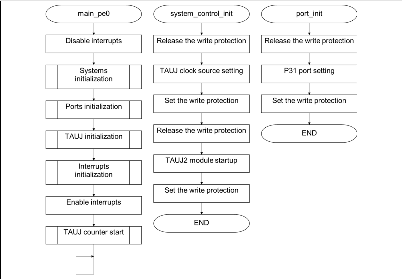
Figure 1-4 Operation flowchart (1/3)
