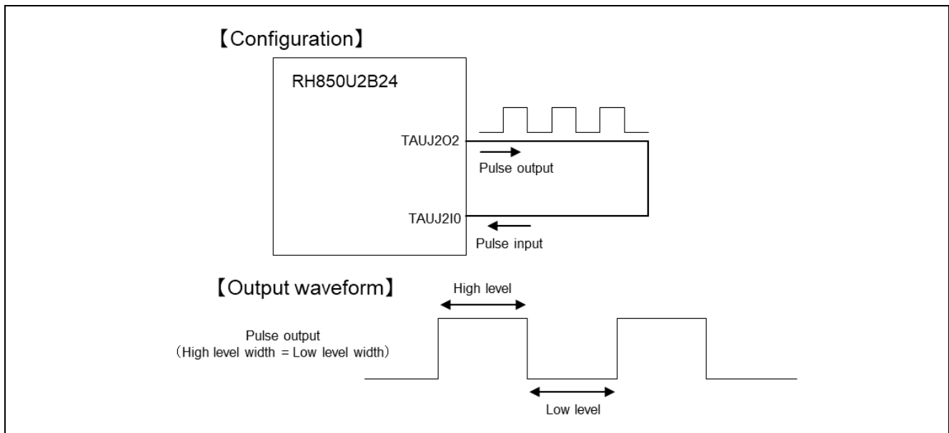
Figure 2-1 Overview diagram
