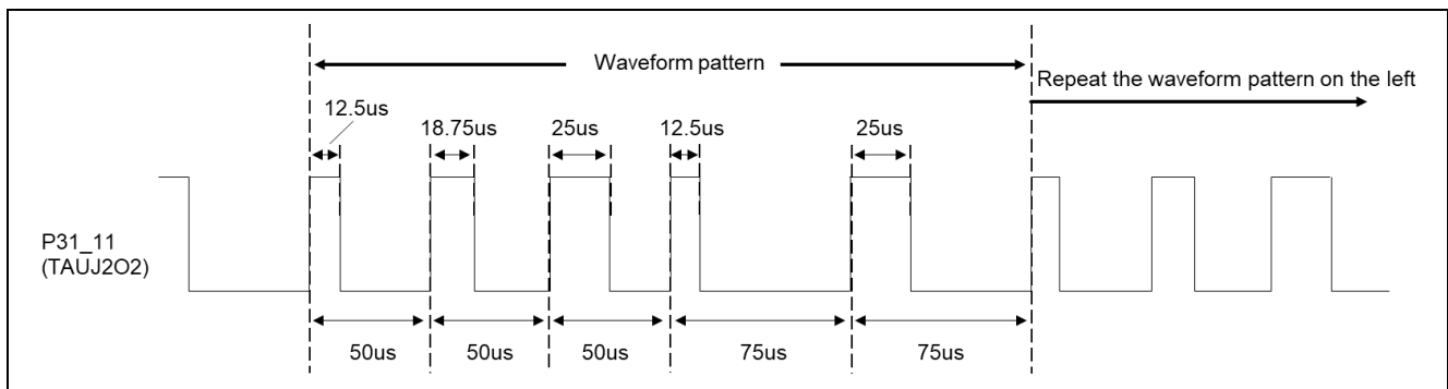
Figure 1-2 Output waveform
