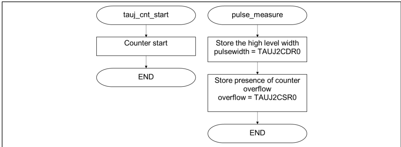
Figure 2-3 Operation flowchart (3/3)
