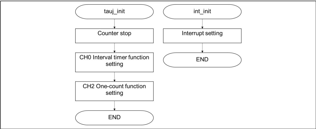
Figure 1-4 Operation flowchart (2/3)
