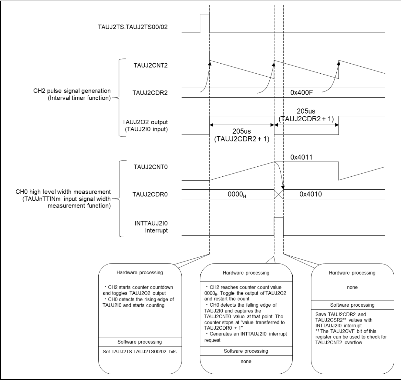
Figure 2-2 Operating diagram
