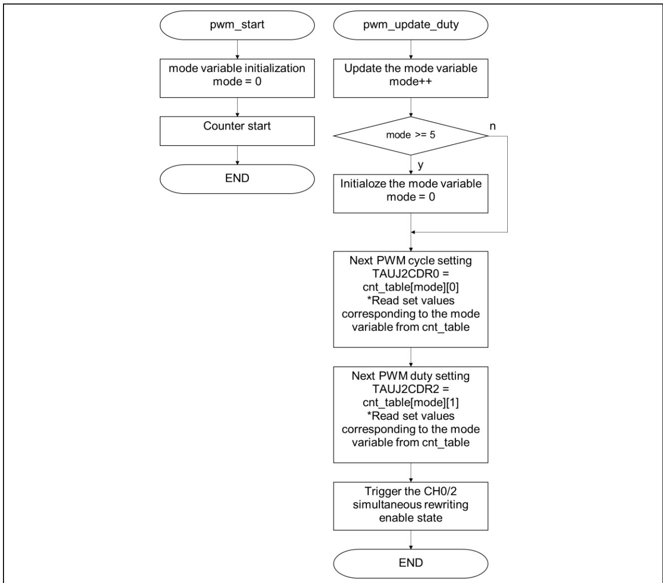
Figure 1-4 Operation flowchart (3/3)
