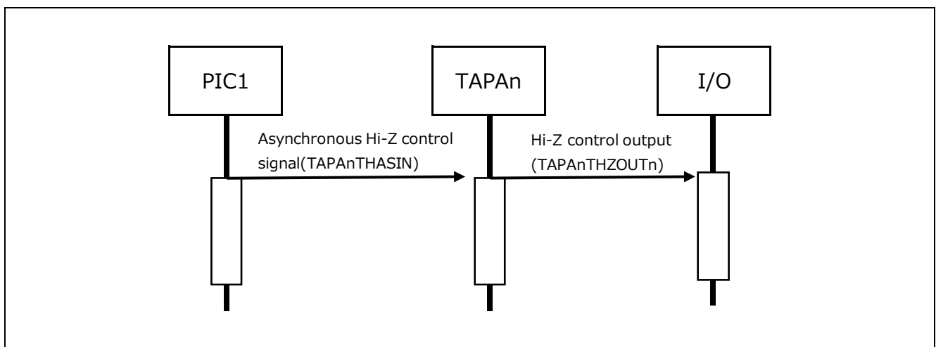
Figure 2-1 Asynchronous Hi-Z control operation
