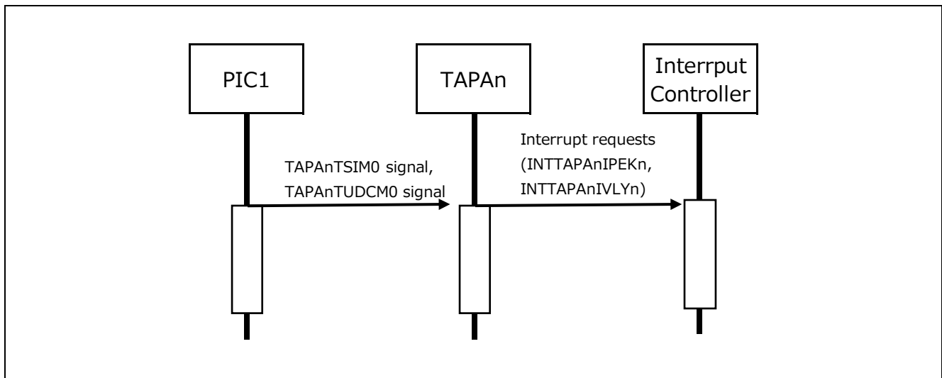
Figure 3-1 Interrupt request output
