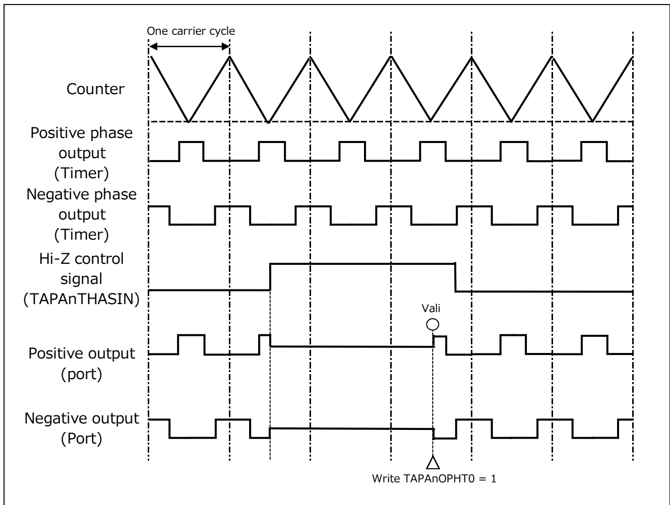
Figure 2-2 The Hi-Z state can be released regardless of the input level of the Hi-Z control signal
