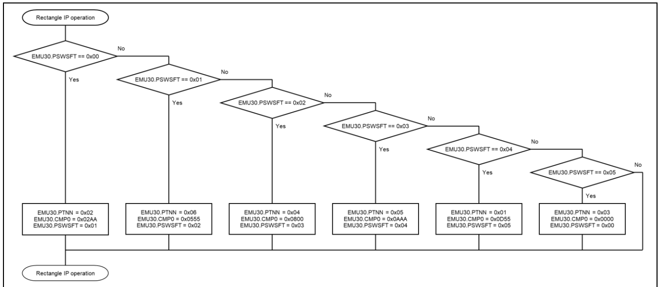
Figure 2-6 Operation flowchart of rectangle IP (handled by interrupt on angle compare 0 match)
