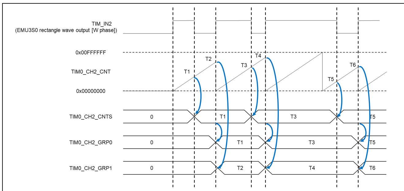
Figure 2-11 Operation overview
