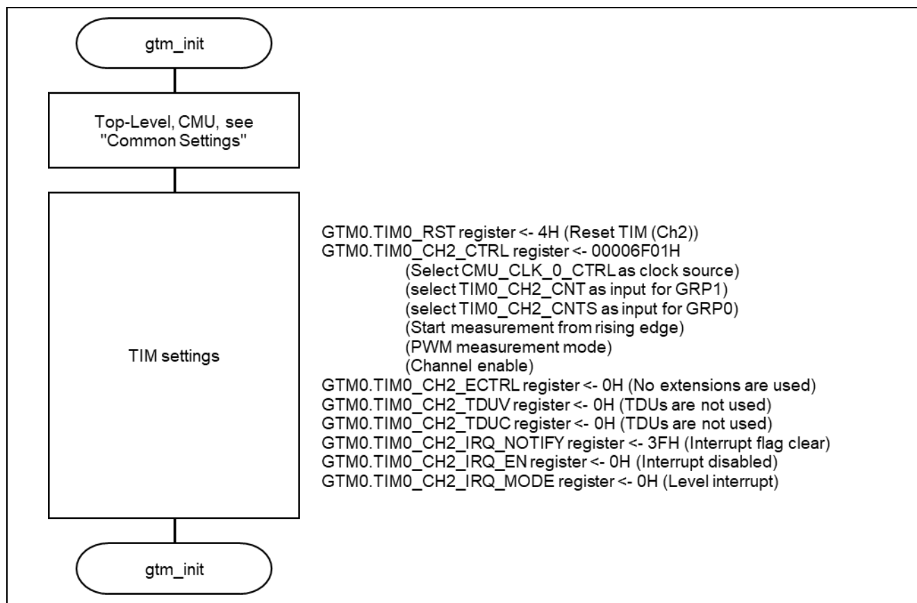
Figure 2-12 GTM (TIM) operation flowchart
