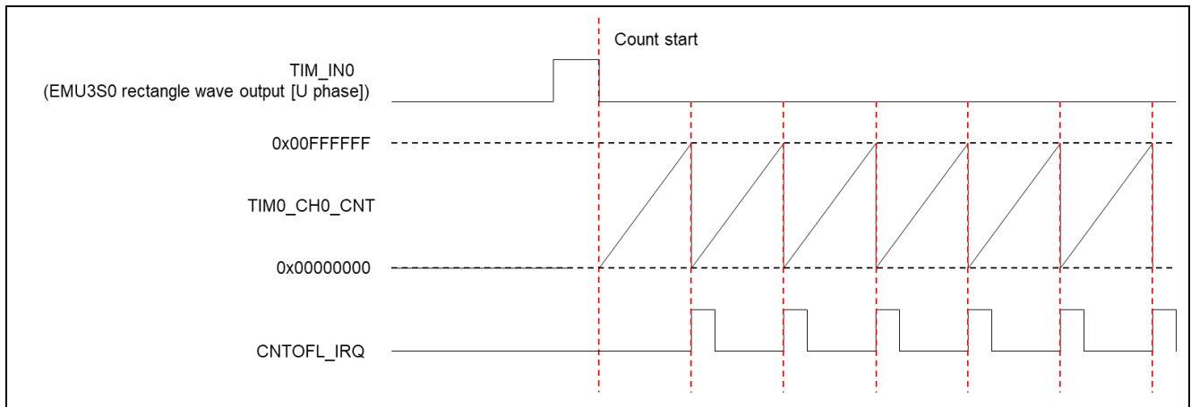
Figure 2-7 Operation overview
