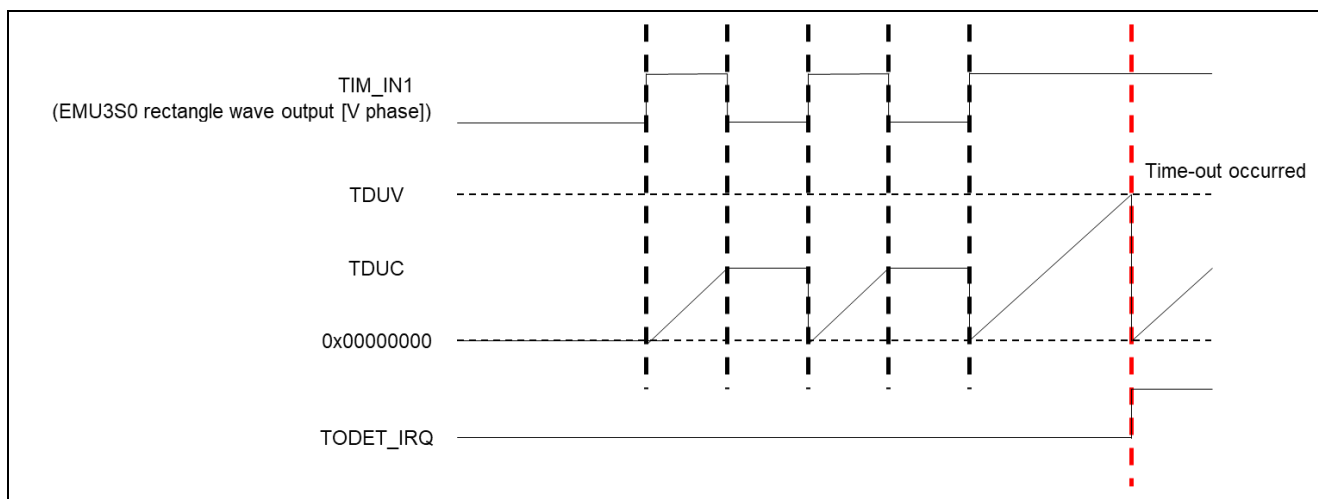
Figure 2-9 Operation overview
