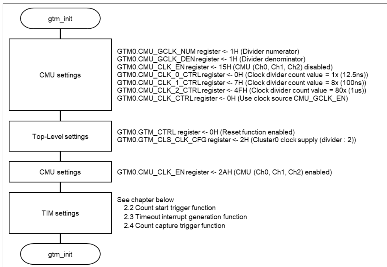
Figure 2-2 GTM initial settings
