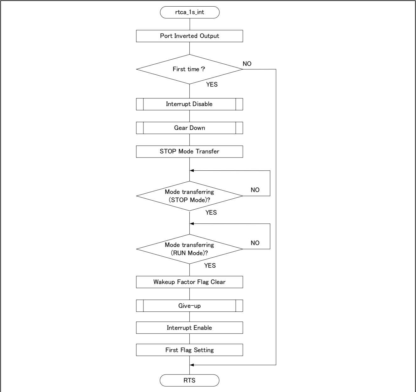
Figure 2-9 RTCA1S Interrupt Function Flowchart
