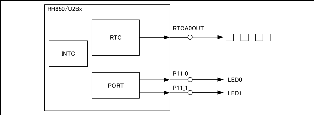
Figure 2-1 System Configuration
