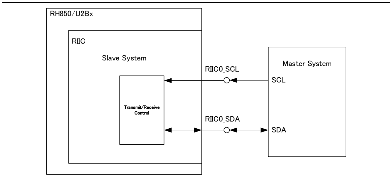
Figure 2-17 System Configuration
