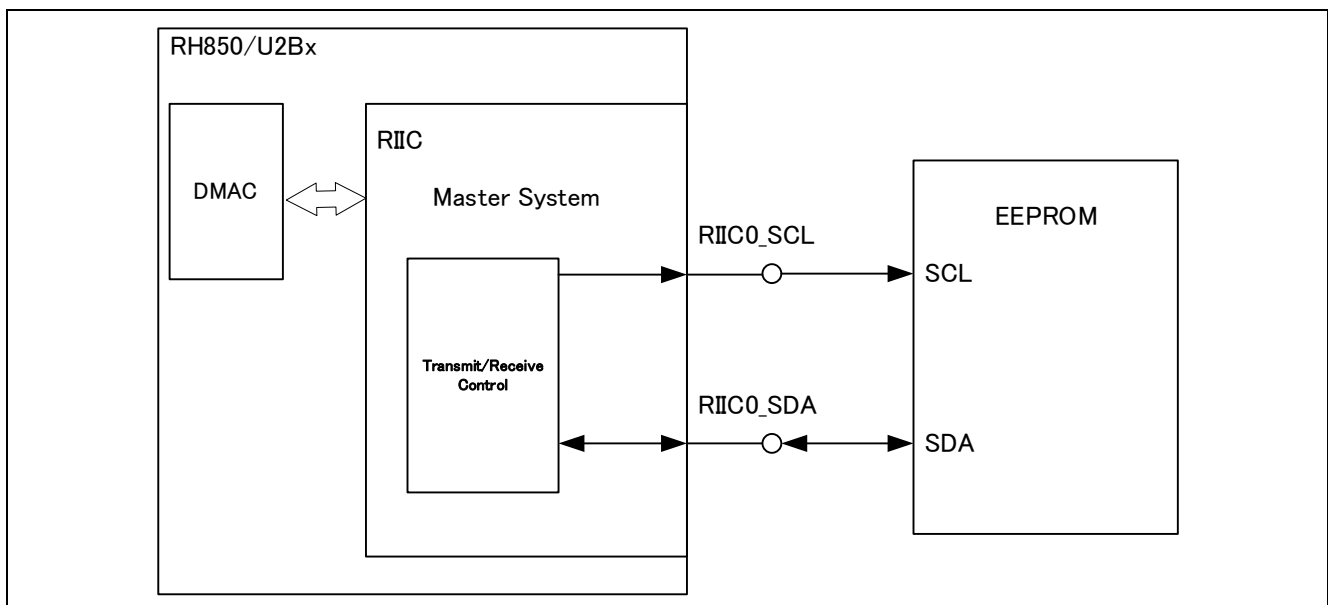
Figure 2-7 System Configuration
