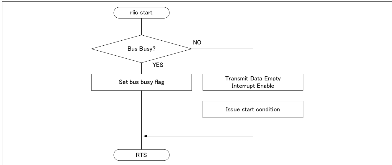
Figure 2-13 RIIC Start Function Flowchart
