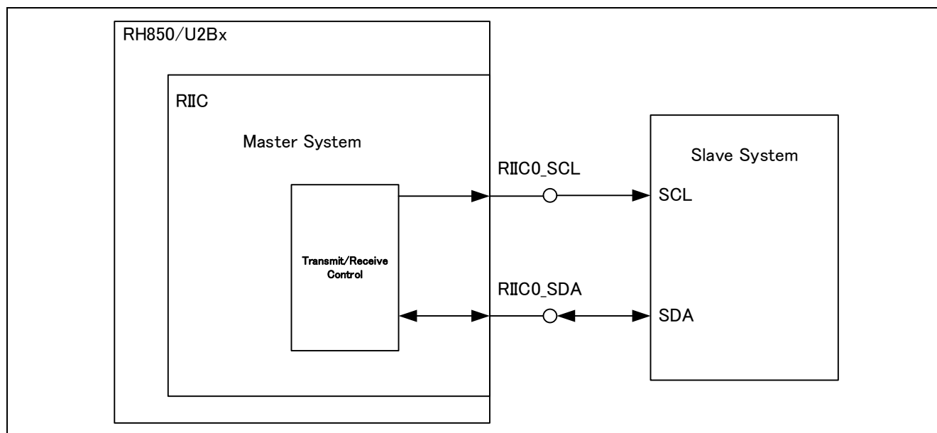
Figure 2-11 System Configuration
