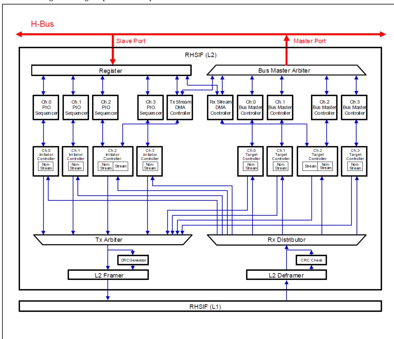
Figure 6: Transport Layer simplified Block Diagram
