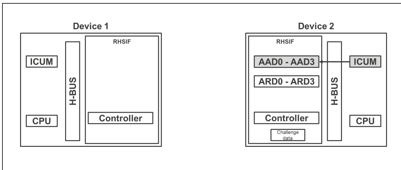
Figure 14: Challenge & Response Authentication Step -3- [2]
