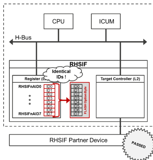
Figure 11: ID-Based Authentication Process Step -4- [2]
