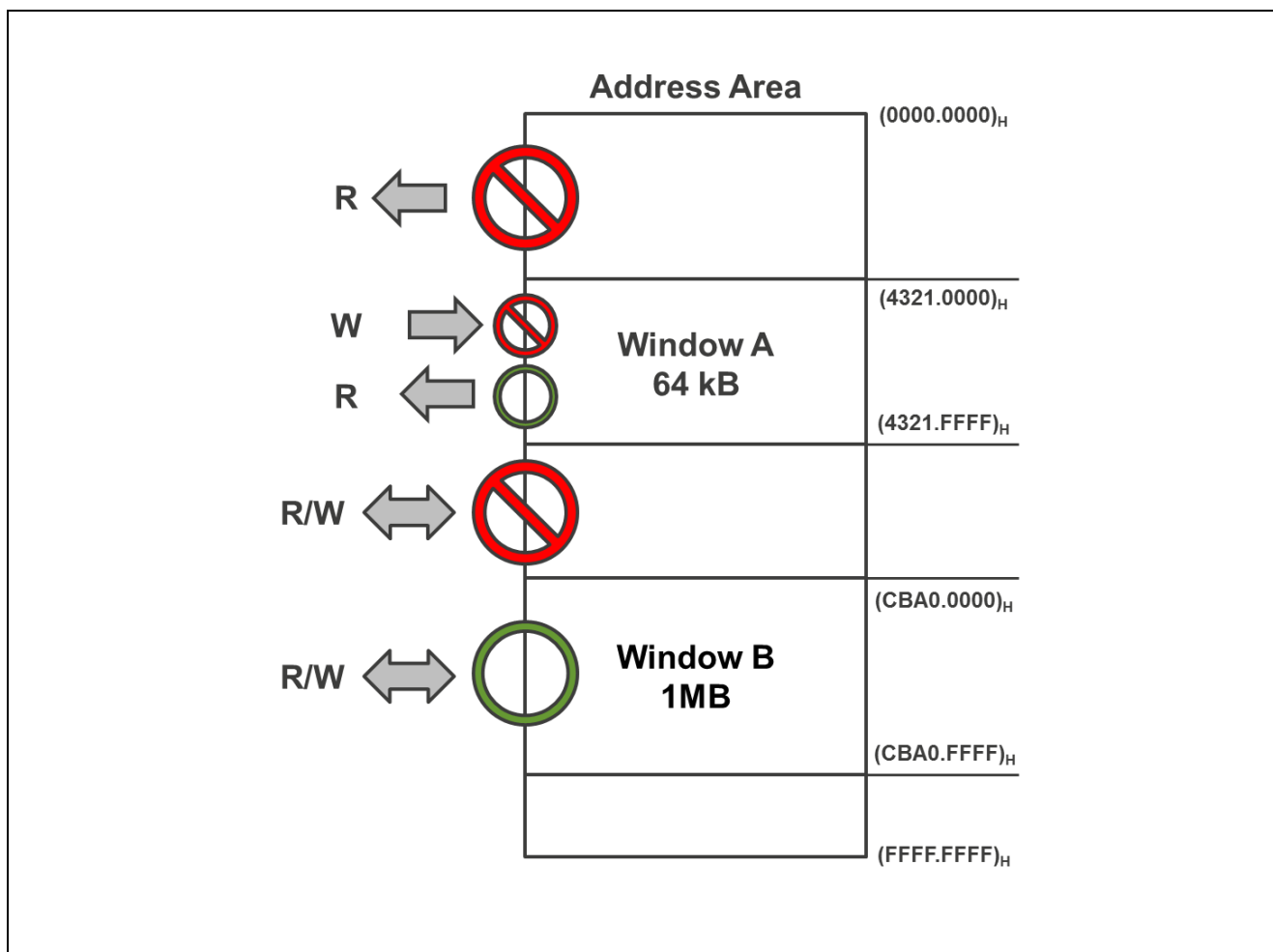
Figure 17: Memory Address Windows [2]
