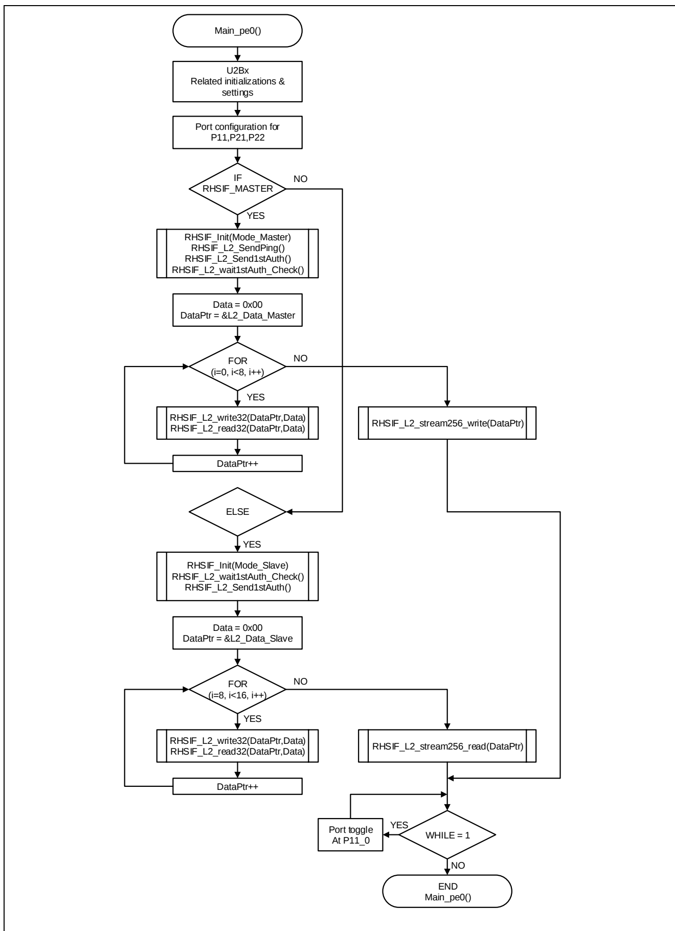
Figure 21: Flowchart “main_pe0.c”
