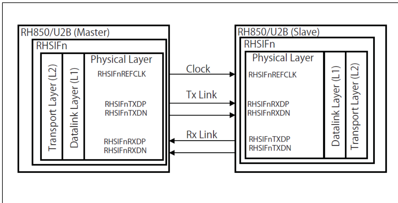
Figure 2: Interconnection between RHSIF Devices [1]
