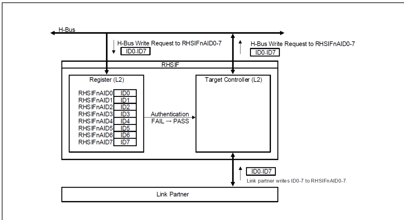
Figure 7: ID-Based Authentication Process -Overview- [2]
