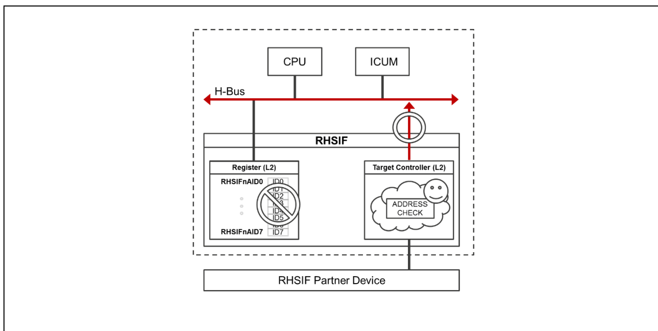
Figure 9: ID-Based Authentication Process Step -2- [2]
