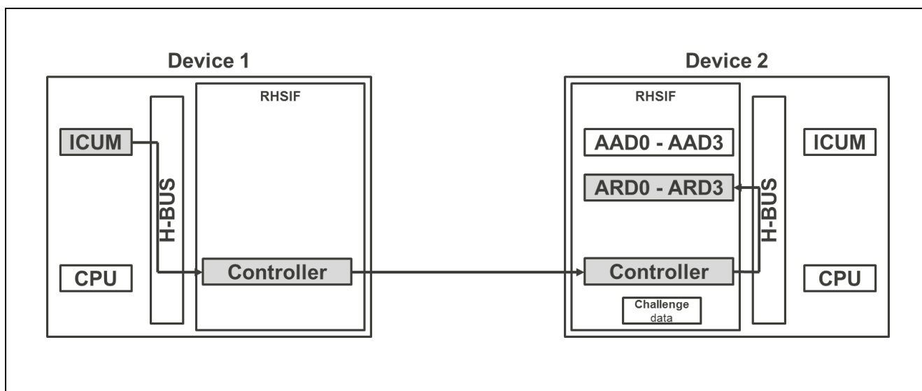
Figure 15: Challenge & Response Authentication Step -4- [2]
