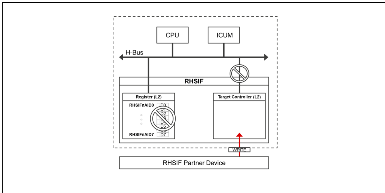
Figure 8: ID-Based Authentication Process Step -1- [2]
