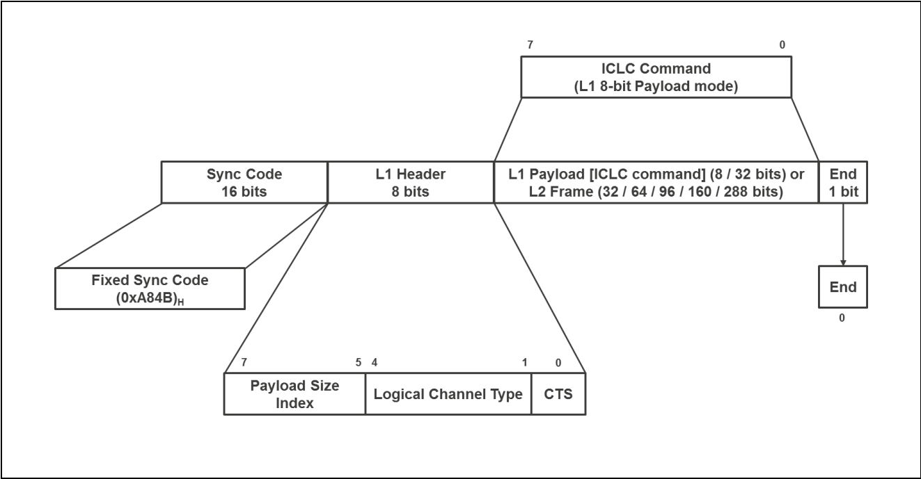
Figure 3: RHSIF L1 Frame detail [2]
