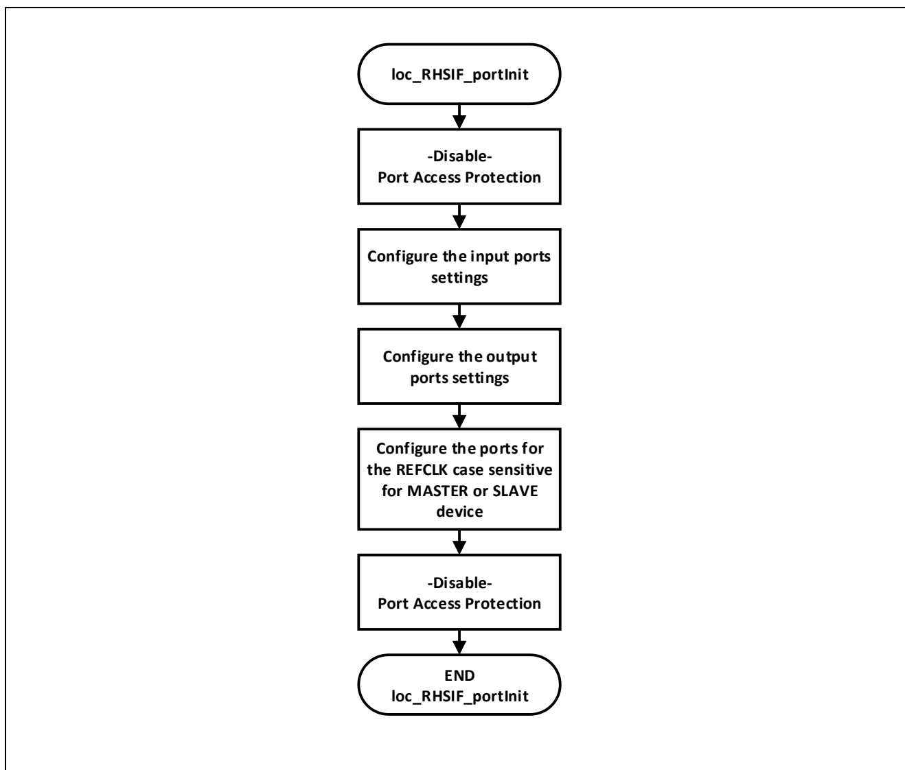
Figure 24: Flowchart “loc_RHSIF_portInit” Function
