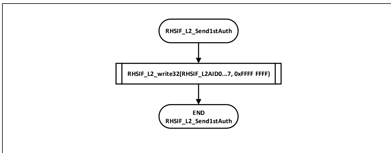
Figure 26: Flowchart “RHSIF_L2_Send1stAuth” Function
