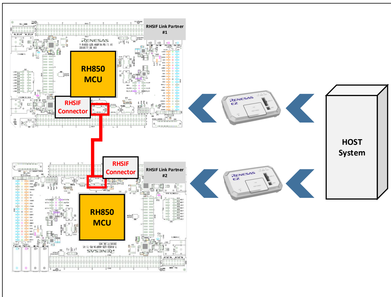
Figure 18: PiggyBack Board Hardware Interconnection
