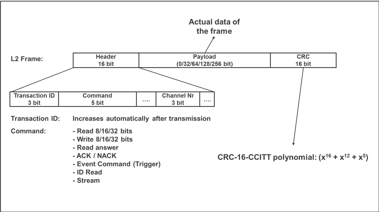
Figure 4: RHSIF L2 Frame detail [2]
