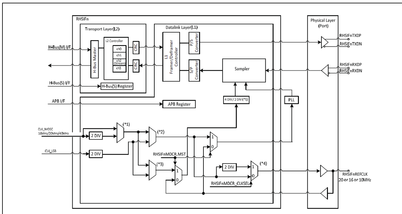
Figure 1: RHSIF Module Block Diagram [1]
