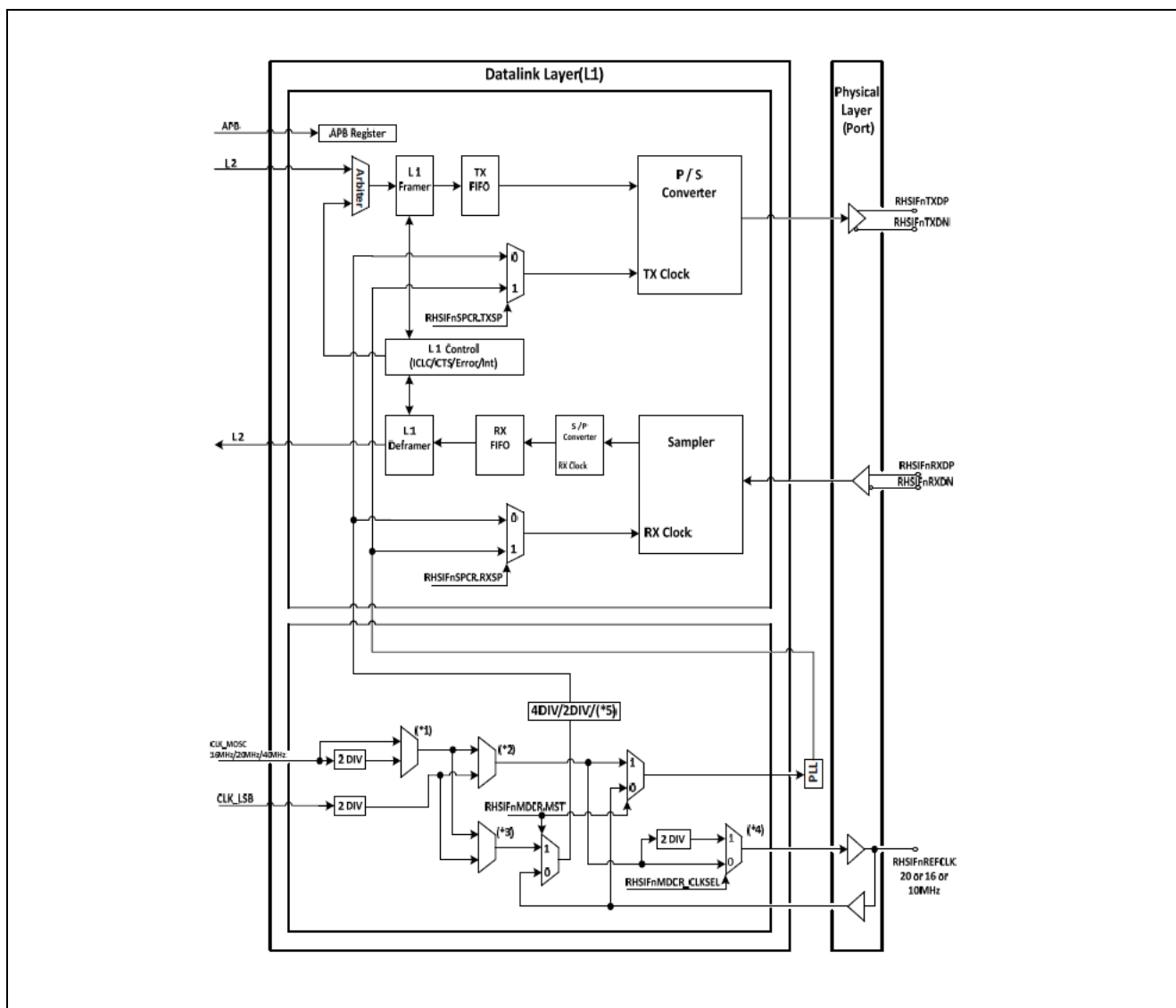
Figure 5: Datalink Layer Block Diagram [1]
