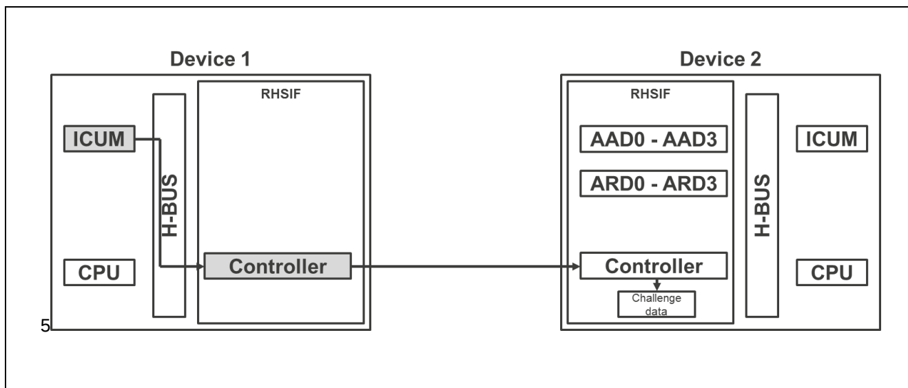
Figure 12: Challenge & Response Authentication Step -1- [2]
