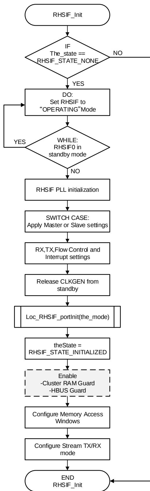
Figure 23: Flowchart “RHSIF_Init” Function
