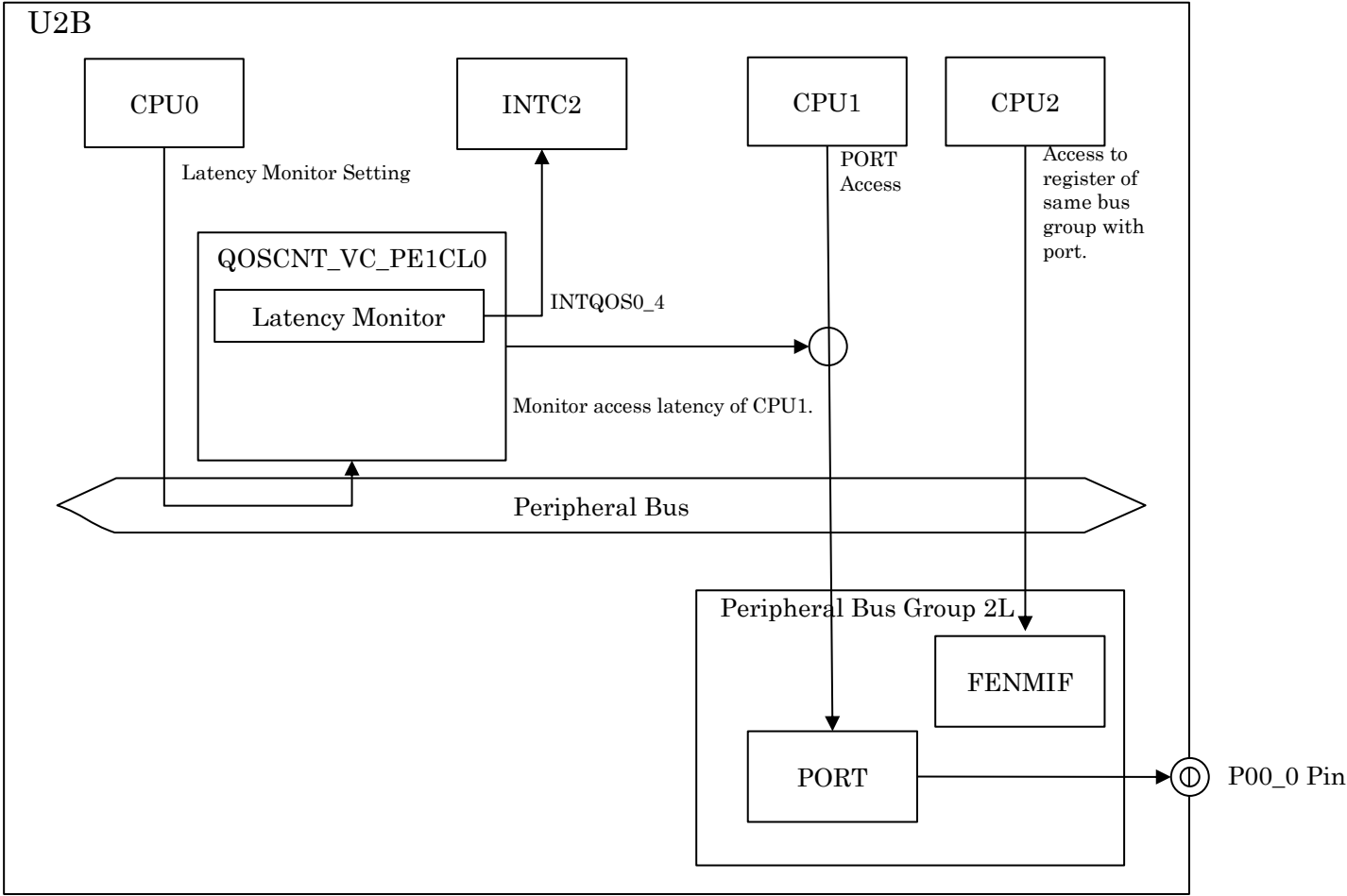
Figure 3-9 System Configuration
