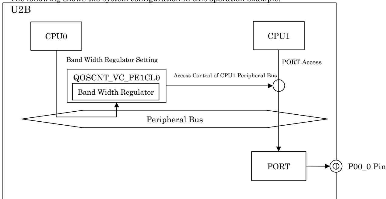
Figure 3-1 System Configuration
