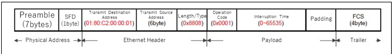
Figure 1-4 Frame Format of PAUSE Frame
