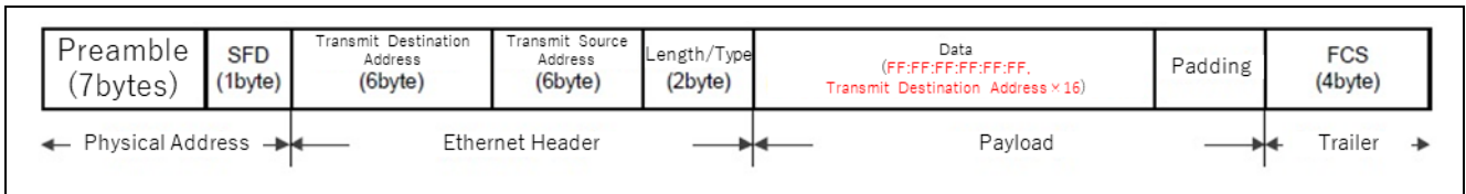
Figure 1-5 Frame Format of Magic Packet
