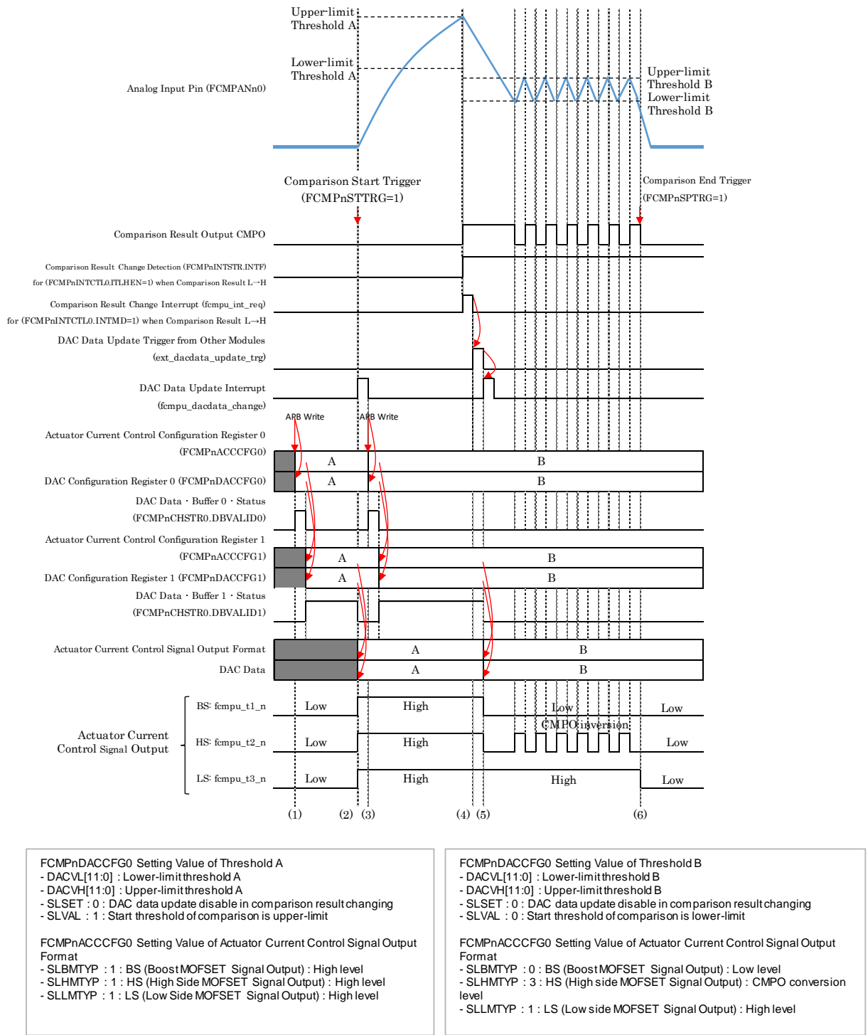
Figure 3-1 Actuator Current Control by External Trigger
