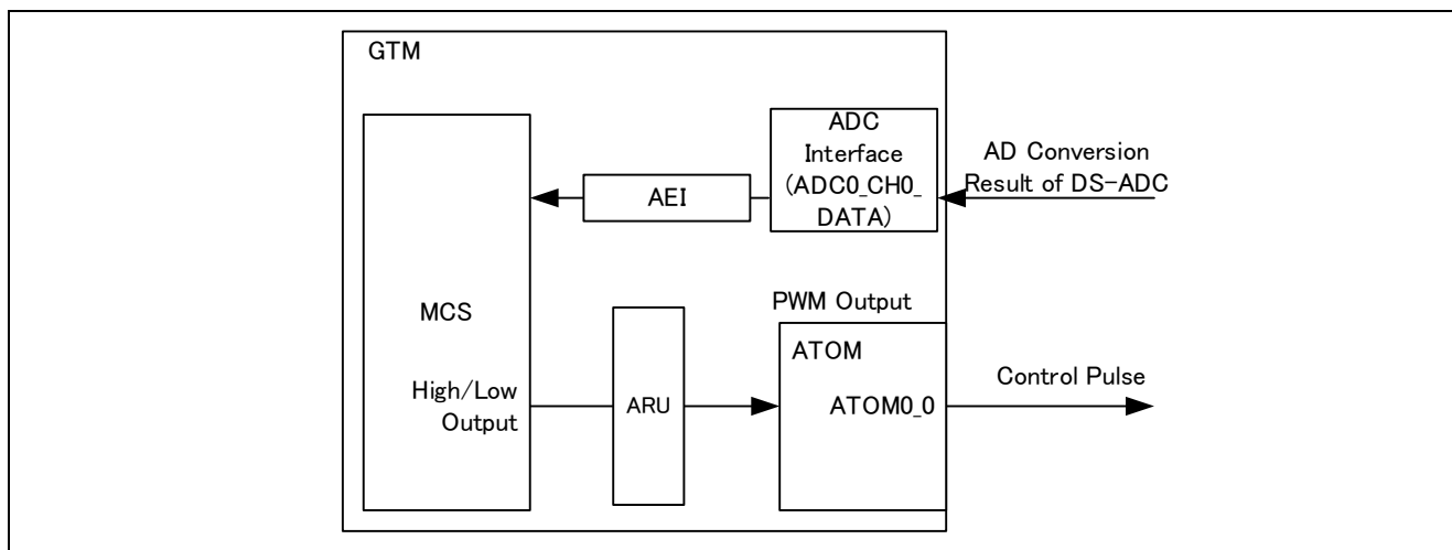
Figure 2-8 Overview Diagram
