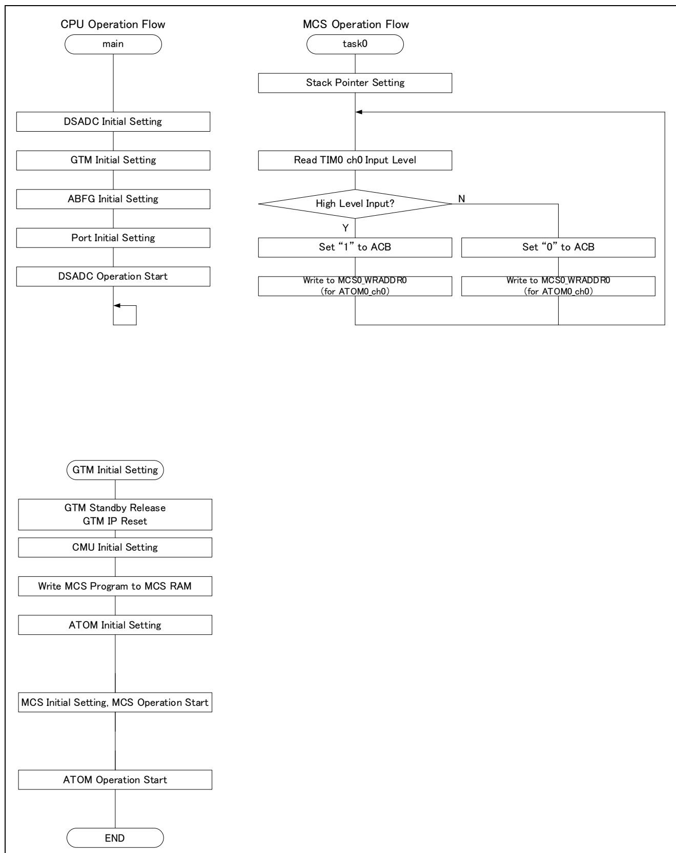
Figure 2-7 Operation Flow
