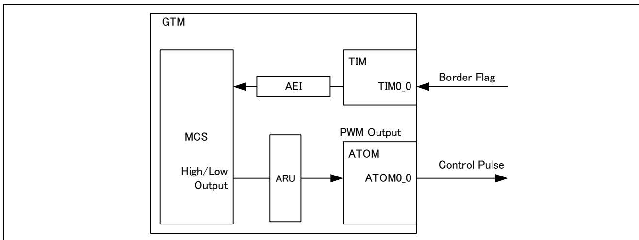
Figure 2-6 Overview Diagram
