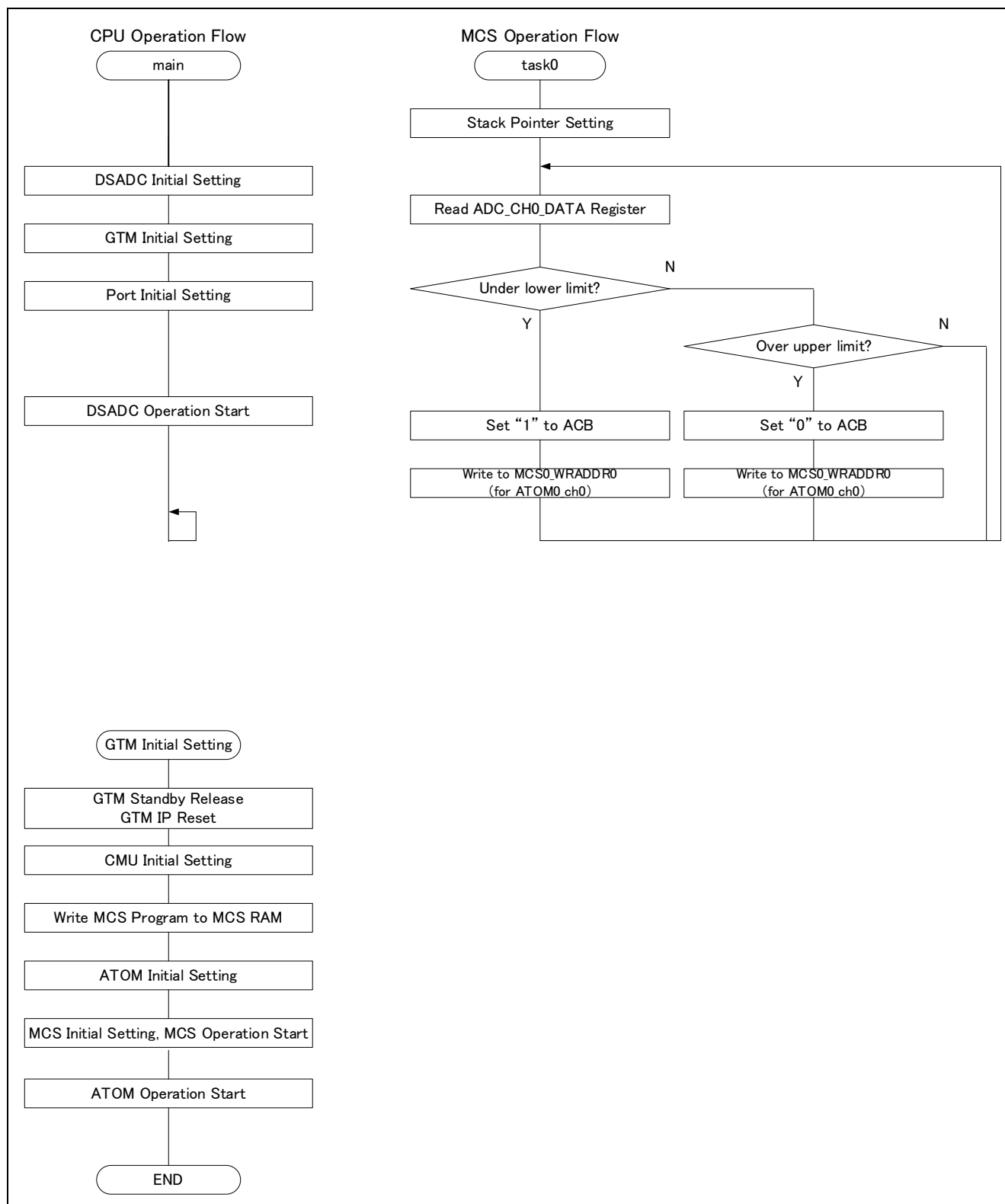
Figure 2-9 Operation Flow
