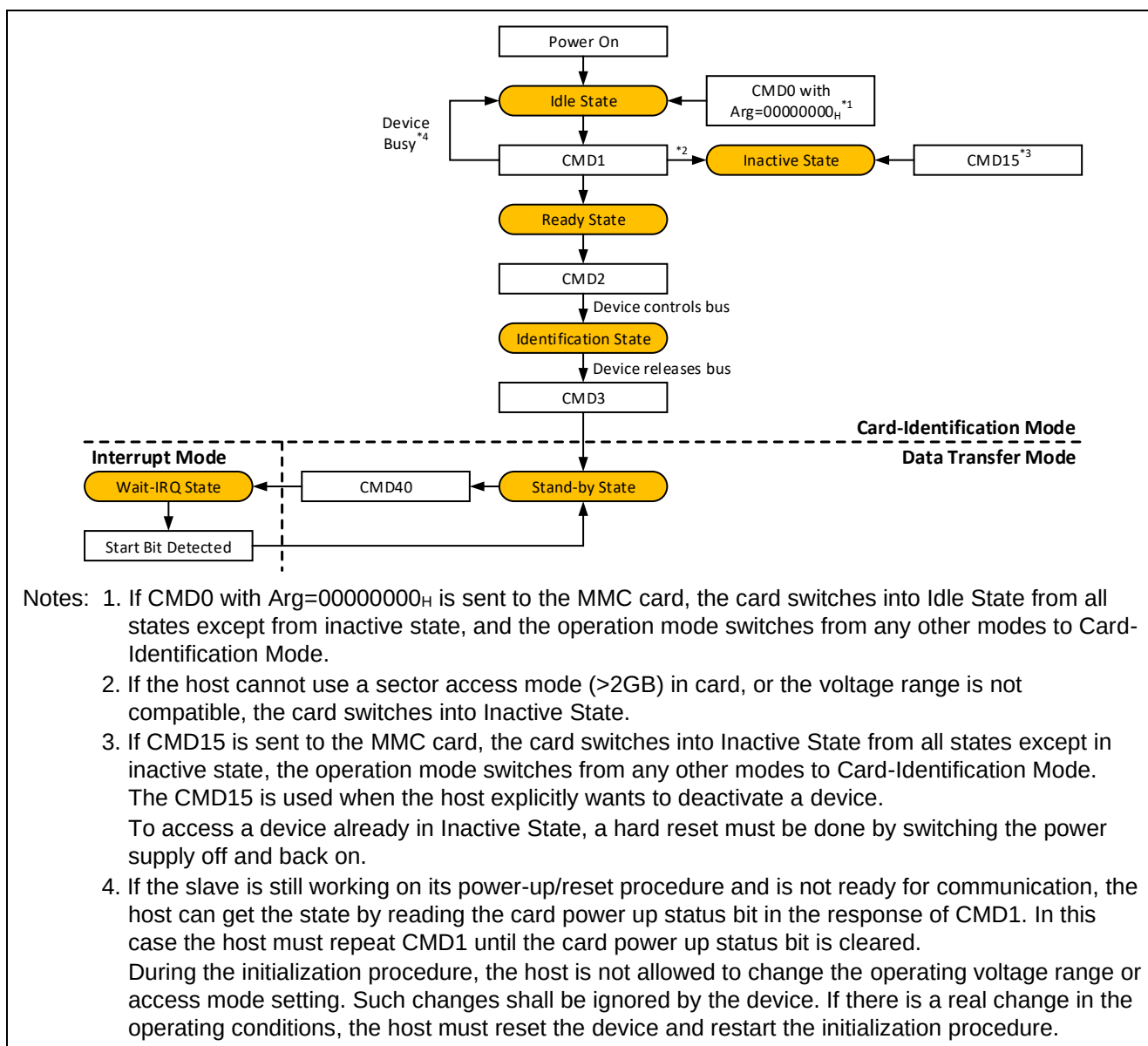
Figure 5-3 Card-Identification Mode
