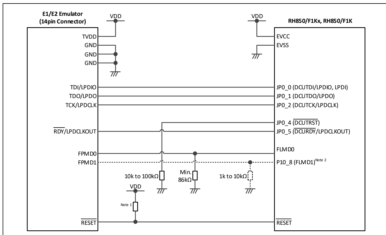
Figure 45: LPD (4 pins) connection
