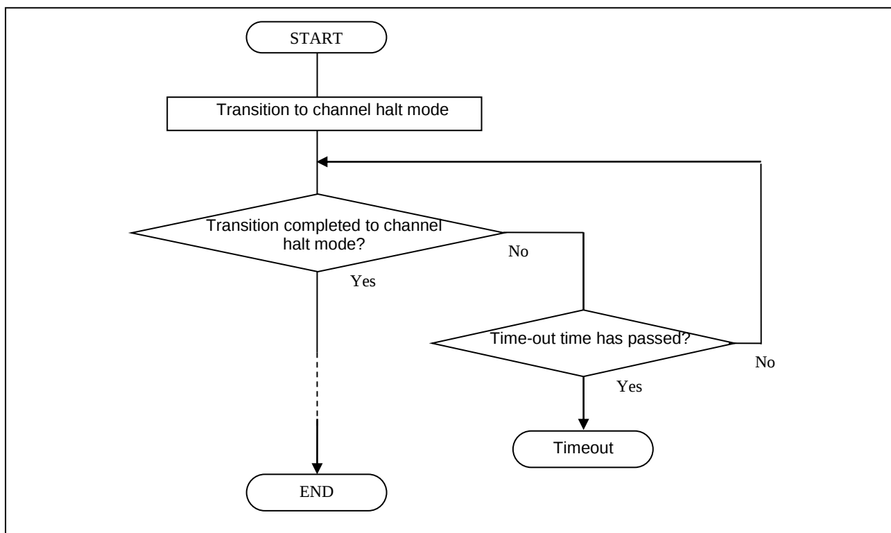
Figure 4-1 Example of Processing with Loop Time Limit
