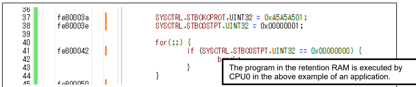
Figure 4-39 Example of a Program that Causes a Transition to Cyclic Stop Mode
