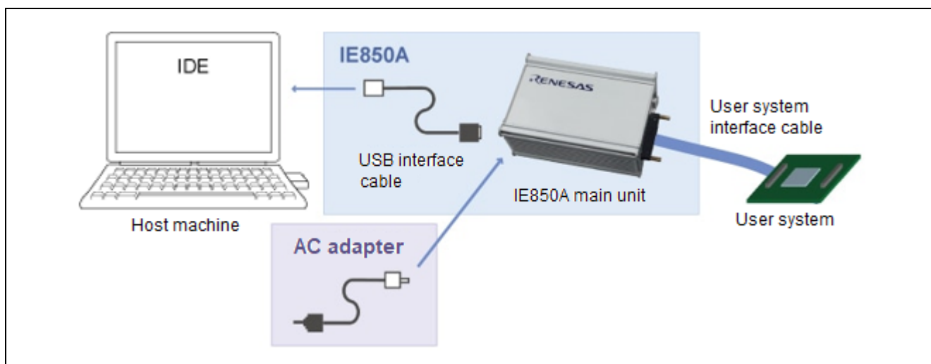
Figure 2-2 System Configuration (IE850A Emulator)
