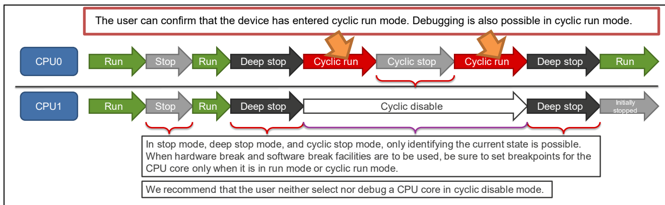
Figure 4-27 Confirming Cyclic Run Mode in Example Application 2
