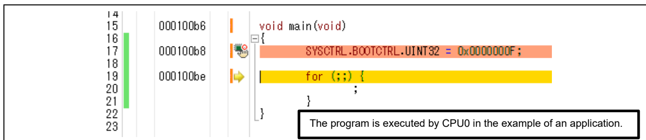
Figure 4-6 Example of a Program for Activating the Initially Stopped Core
