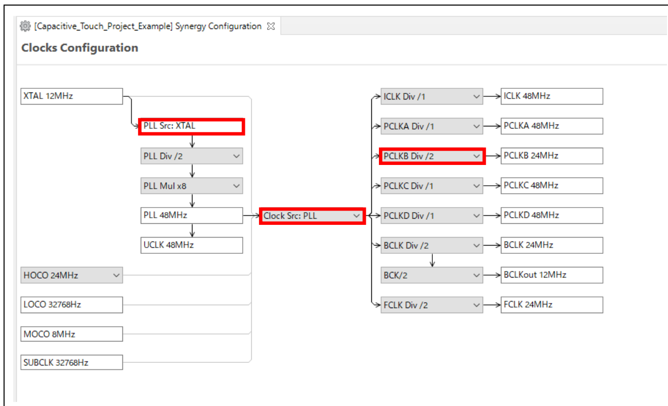
Figure 5. Clocks Tab – Clocks Configuration
