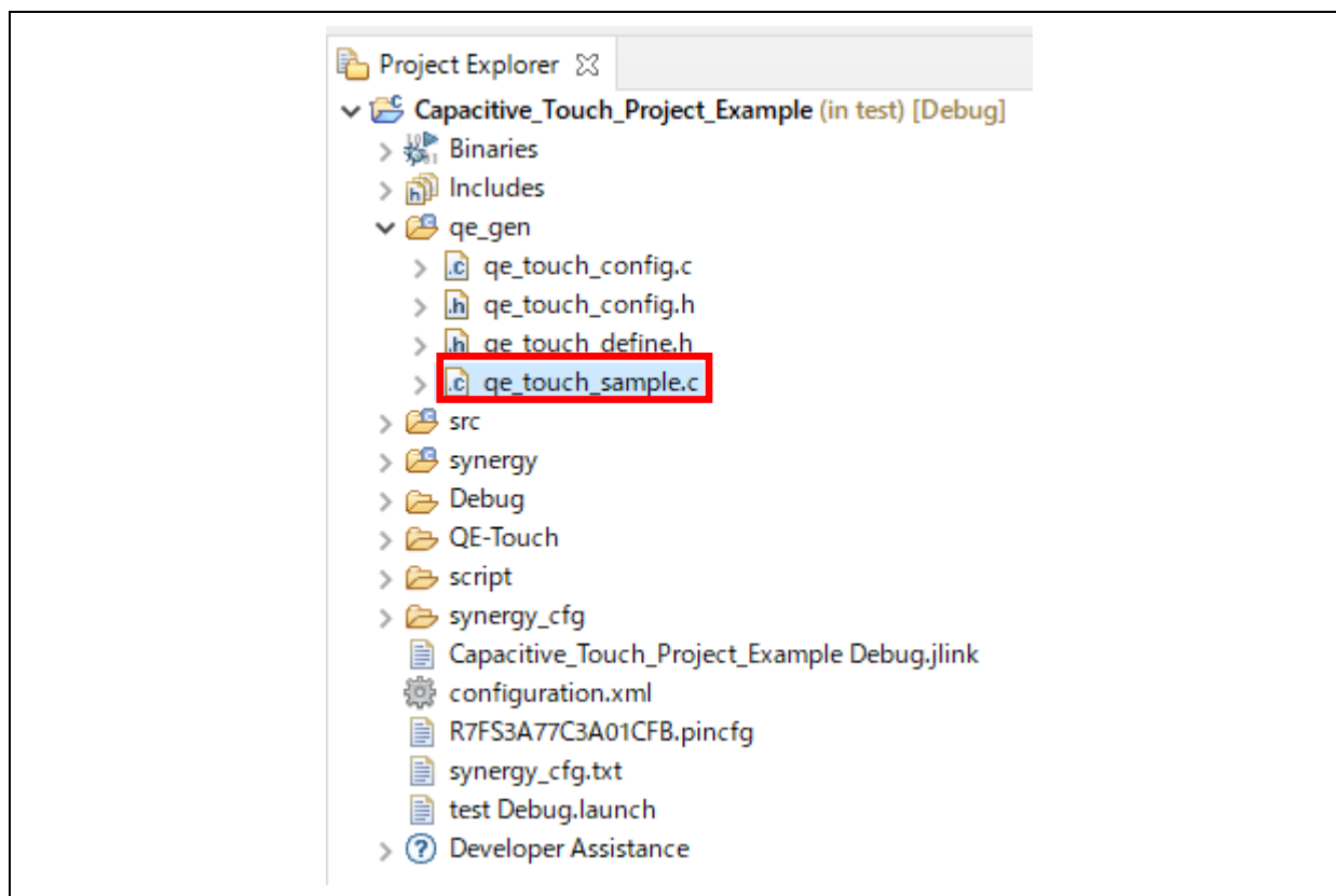
Figure 48. qe_touch_sample.c
