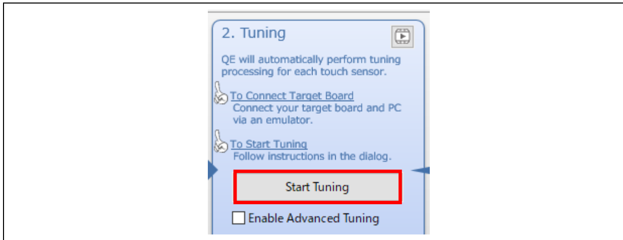
Figure 38. Start Tuning
