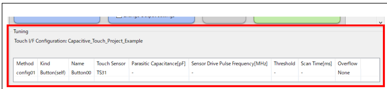
Figure 33. Tuning Pane
