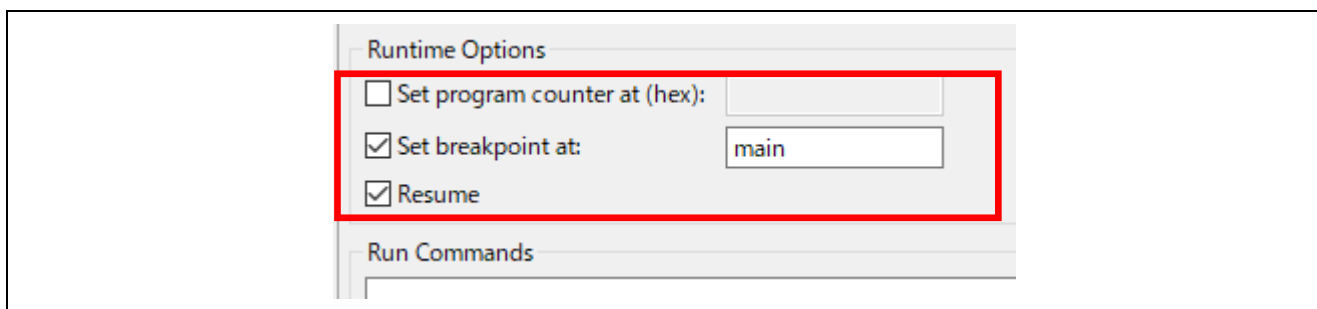
Figure 37. Runtime Option
