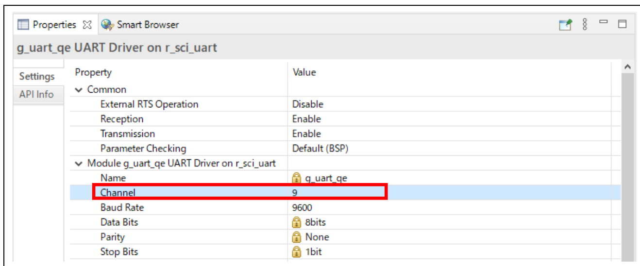
Figure 23. Channel
