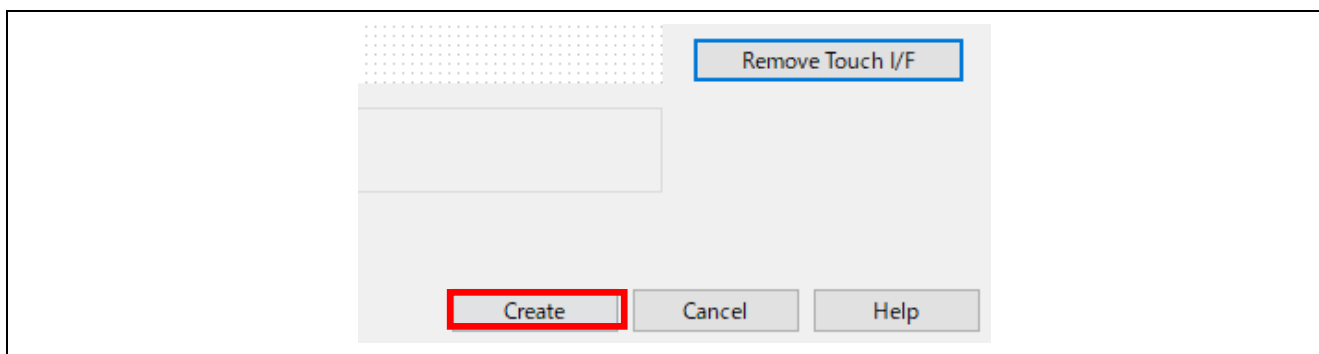
Figure 32. Create Button
