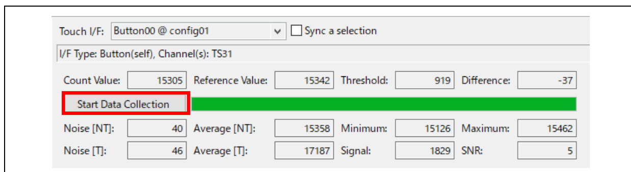
Figure 65. Stop Data Collection Button (touch-on state)
