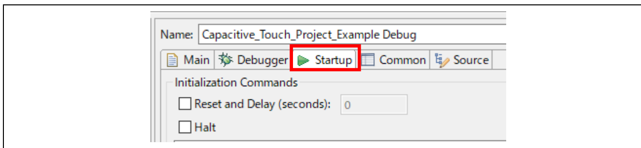
Figure 36. Startup Tab
