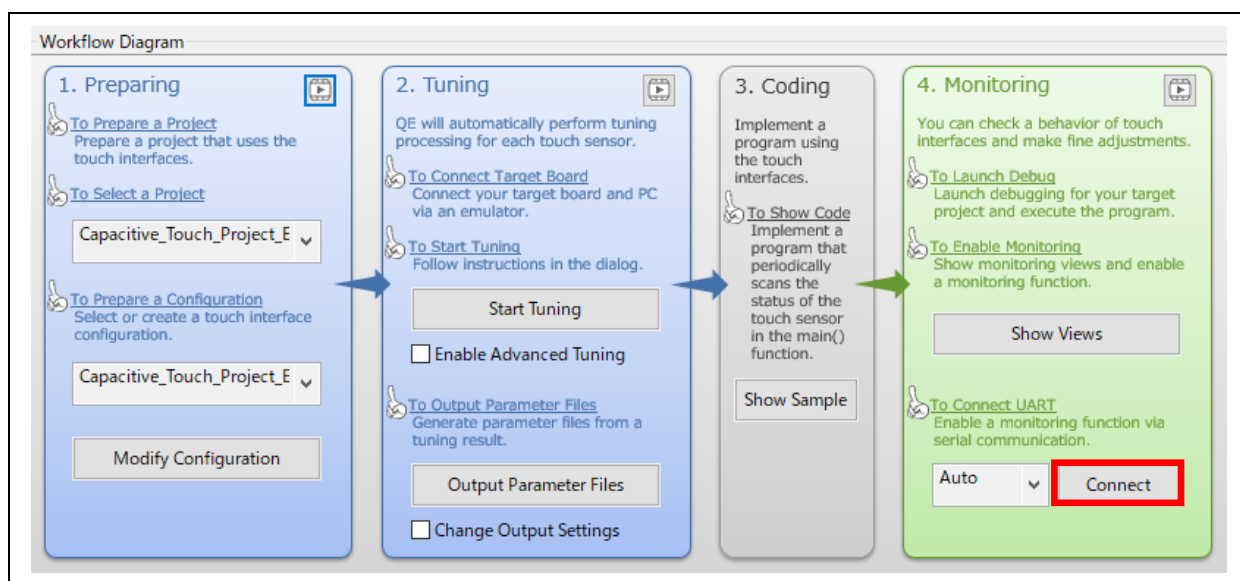
Figure 68. Connect Button
