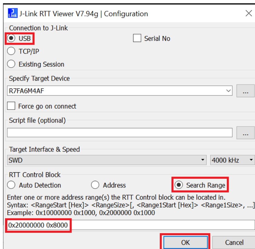
Figure 30. SEGGER RTT Viewer Connection Setup when MCU Running in Standalone Mode
