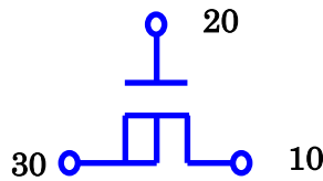
Figure 2-3 Terminal configuration (G2 model)
