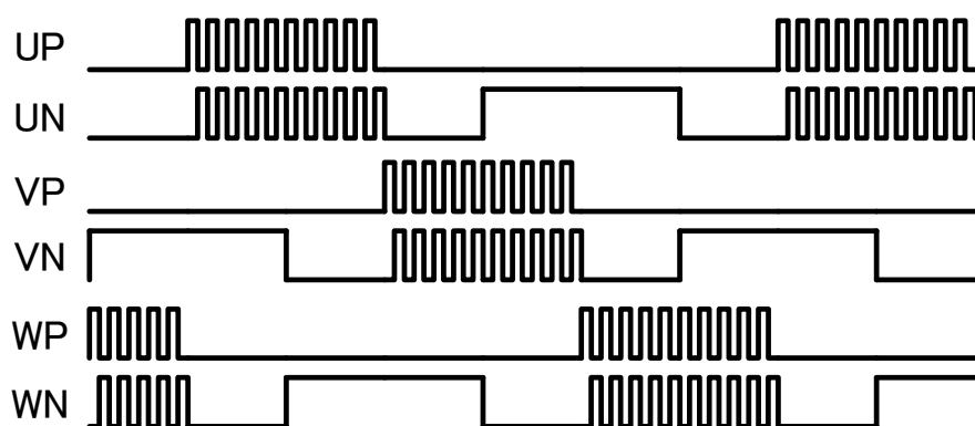
Figure 3-4 Upper Arm Chopping (Complementary PWM)
