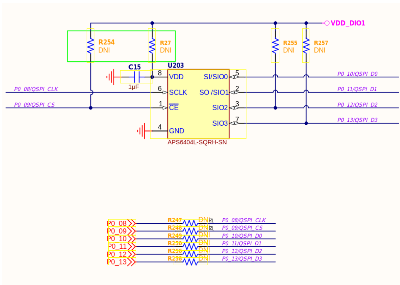
Figure 1. PSRAM Circuitry schematic
