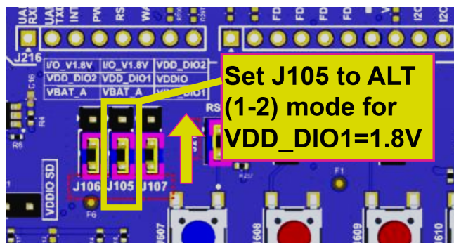
Figure 5. VDDIO jumper configuration for 1.8 V - EVK reference
