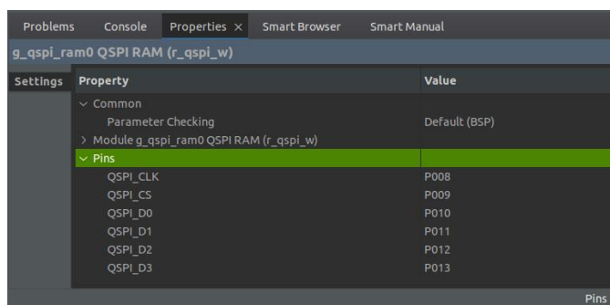
Figure 8. Default pin assignment for QSPI PSRAM
