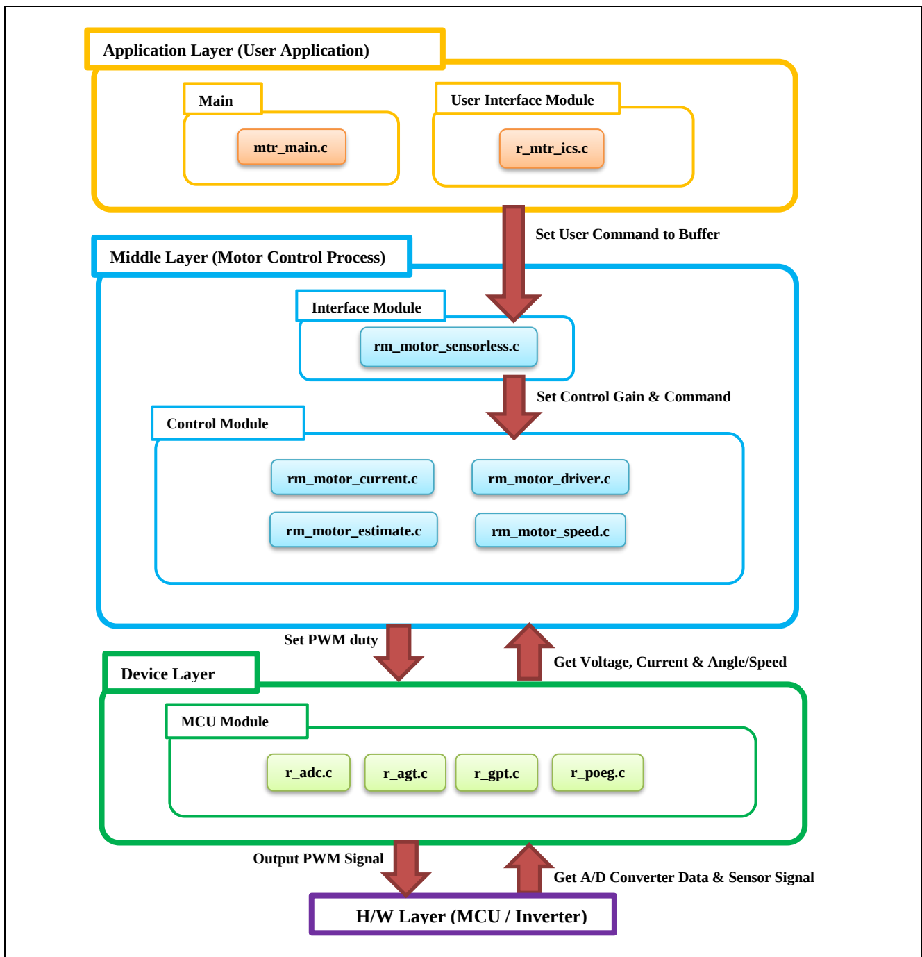
Figure 2-7 Module Configuration
