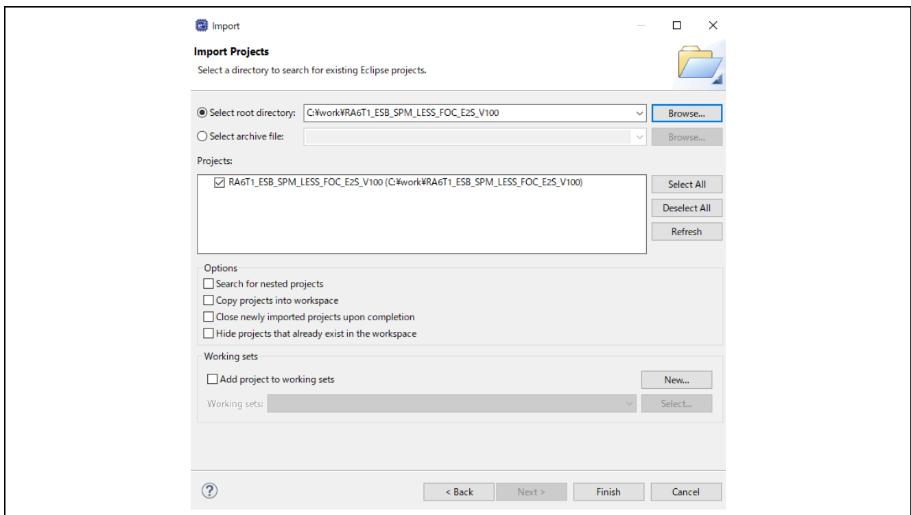
Figure 4-3 Import Projects
