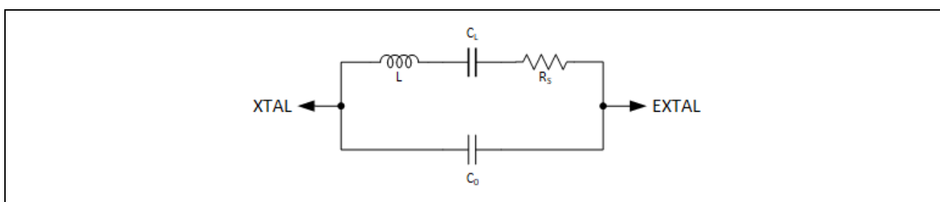
Figure 14. Equivalent Circuit of the Crystal Resonator
