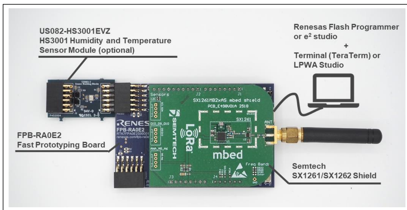
Figure 8. FPB-RA0E2 Hardware Setup Example
