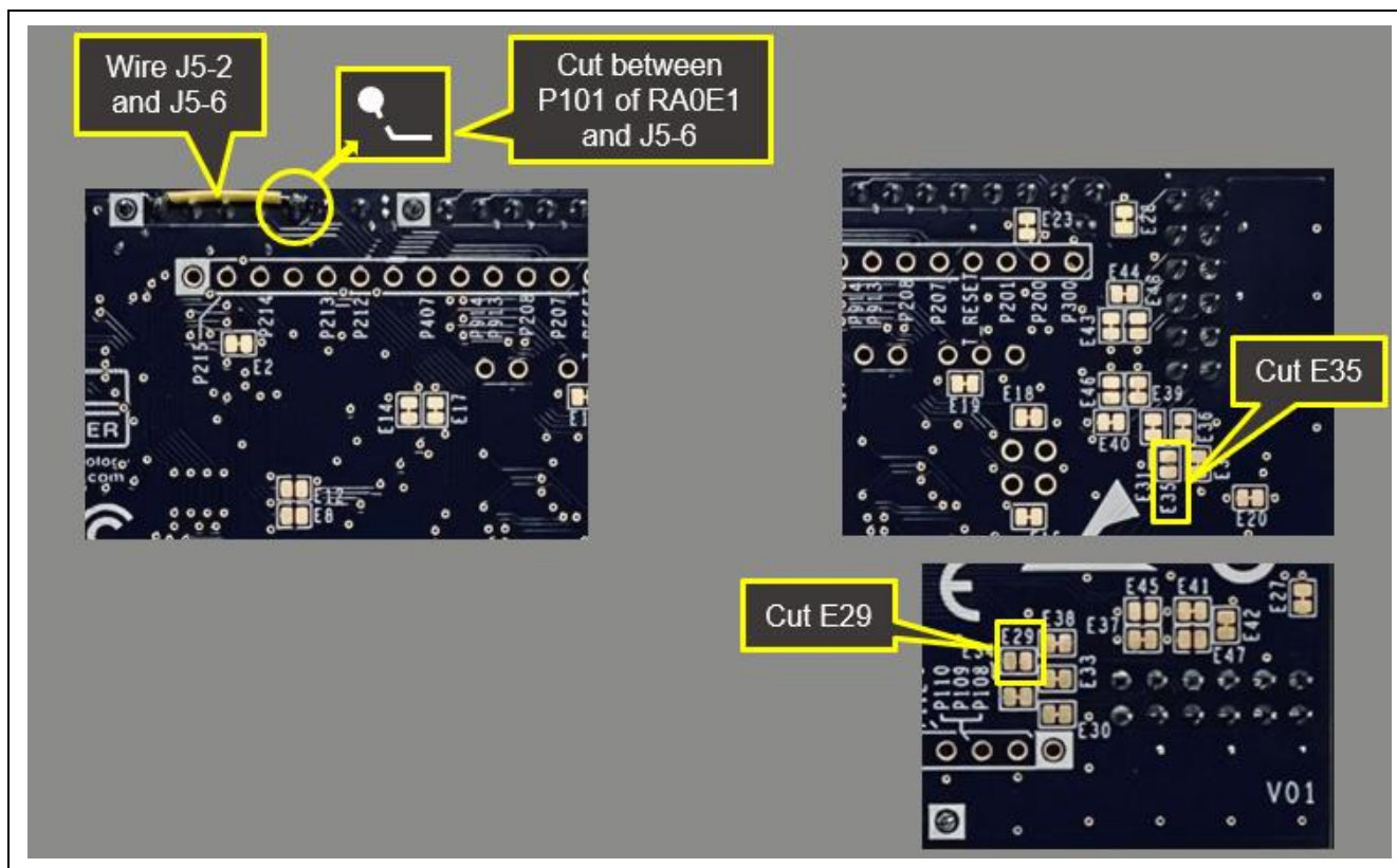
Figure 7. FPB-RA0E1 Configuration Pins
