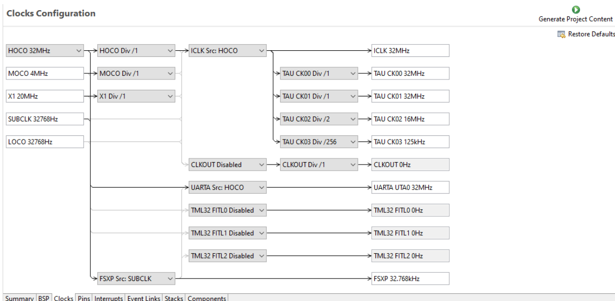
Figure 6. Clock Settings Using Renesas FSP Configurator
