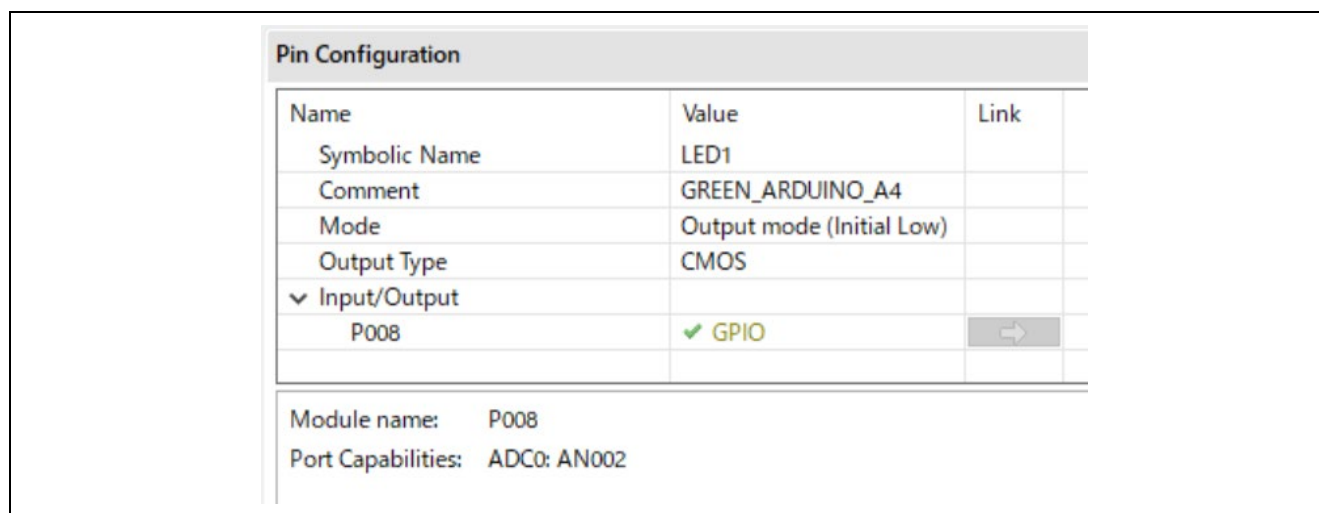
Figure 15. Configuring P008 on the RA0E1 as Output and Low using FSP Configurator
