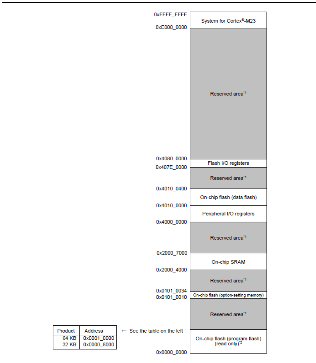
Figure 10. RA0E1 Memory Map
